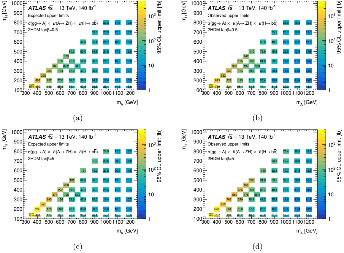
Figure 11. Expected and observed upper limits at 95% CL on \sigma(gg \rightarrow A) \times B(A \rightarrow ZH) \times B(H \rightarrow b\bar{b}) . The limits are shown for \tan\beta = 0.5 (a,b) and \tan\beta = 5 (c,d). The \tan\beta value is relevant only for the choice of A boson width.
