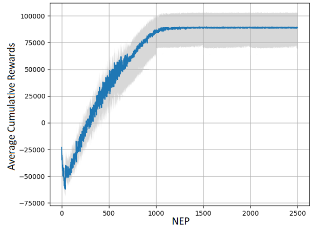
Fig. 3. Multi-Agent: Average Cumulative Reward as a function of NEP
