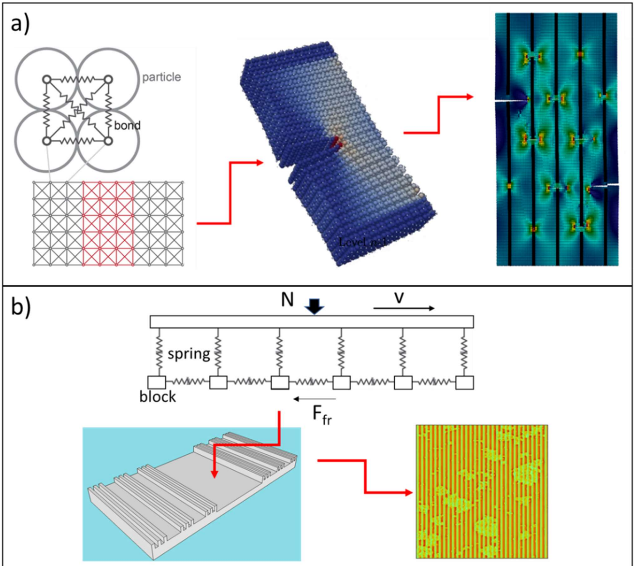
FIGURE 14. a) Hierarchical lattice spring to simulate the fracture of fibre-reinforced composite materials, highlighting the effect of load concentrations and crack stopping effects; b) Spring block model to simulate the friction of hierarchically rough surfaces, highlighting the propagation of surface detachment fronts.
