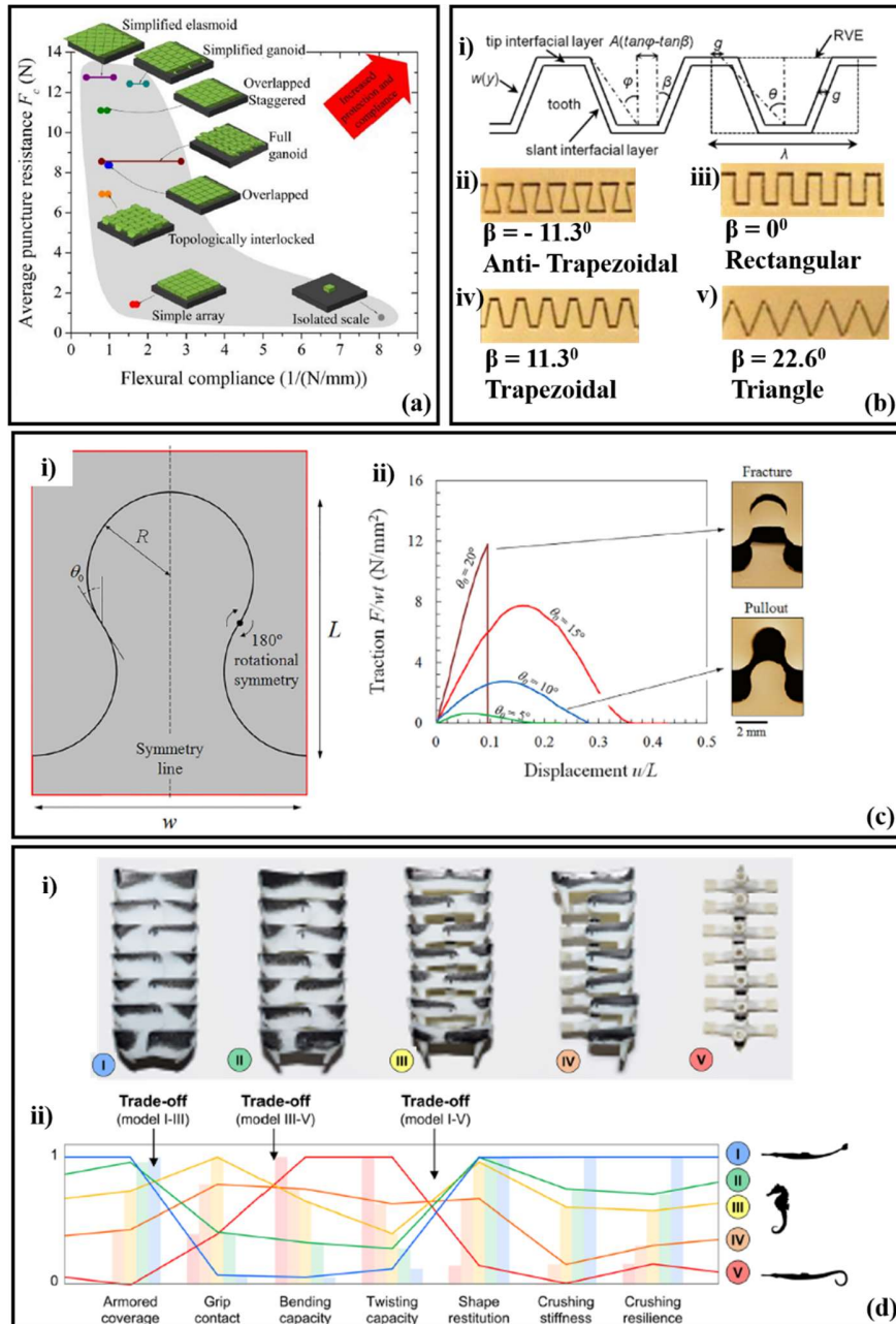
FIGURE 13. (a) Ashby plot showing the combination of flexural compliance vs puncture resistance for different designs[110]. (b) (i) Schematic diagram of suture interfaces with their geometrical parameters. (ii)- (iv) Optical images of suture interface prototypes[111]. (c) (i) Geometry of unit cell of jigsaw locking features, (ii) Representative pull-out curves with different interlocking angles, showing different failure modes: Tab pull-out and fracture[112]. (d) (i) Image of ink-stamped contact areas of the five models. (ii) Comparison of multifunctional performance of models I-V[113].
