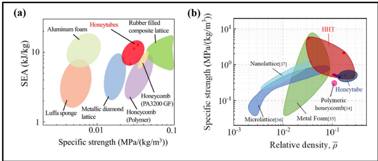
FIGURE 9. (a) Specific energy absorption plotted against specific strength of honeytubes compared to other lightweight cellular materials[95], and (b) Ashby chart for specific strength vs relative density of HHTs and its comparison with other materials[133].
