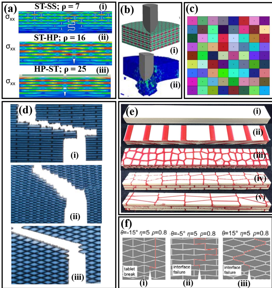
FIGURE 10. Bio-inspired composite structures. (a) (i)-(iii) Three staggered platelet composite specimens with different fracture responses[99]. (b) (i) Quarter geometry of the Nacre-like design in simulations. (ii) Simulation of the impact performance of a Nacre-like sample[100]. (c) Simple view of square Voronoi regions[101]. (d) Schematic of investigated topologies with their fracture patterns.(i) Bone like, (ii) Bio-calcite like, (iii) rotated bone-like[92]. (e) (i) Homogeneous PLA Specimen 1. (ii)-(iii) Nacre-like laminated composite specimens 2 and 3, without and with the use of Voronoi diagrams, respectively. (iv)-(v) Nacre-like laminated composite structure specimens 4 and 5, with doubled platelet and quadrupled platelet, respectively[91]. (f) (i)–(iii) Schematics showing the two different failure modes: interface failure (ii) & (iii) and tablet break (i)[102].
