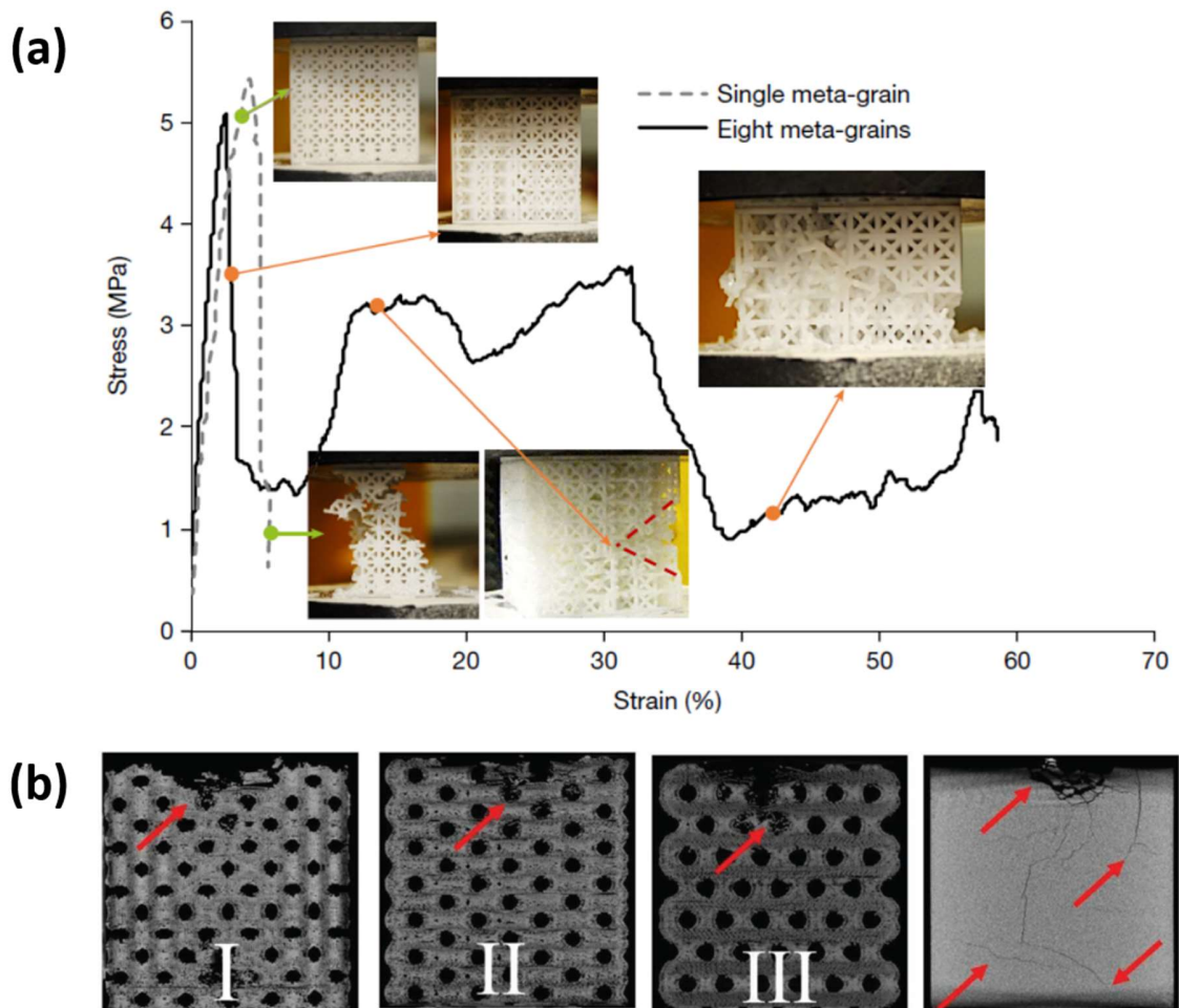
FIGURE 7. (a) Stress-strain curve of single and eight meta-grain structures[81], (b) CT scan snapshots of Hypervelocity impact test of tubulane structures and PLA structure (extreme right)
