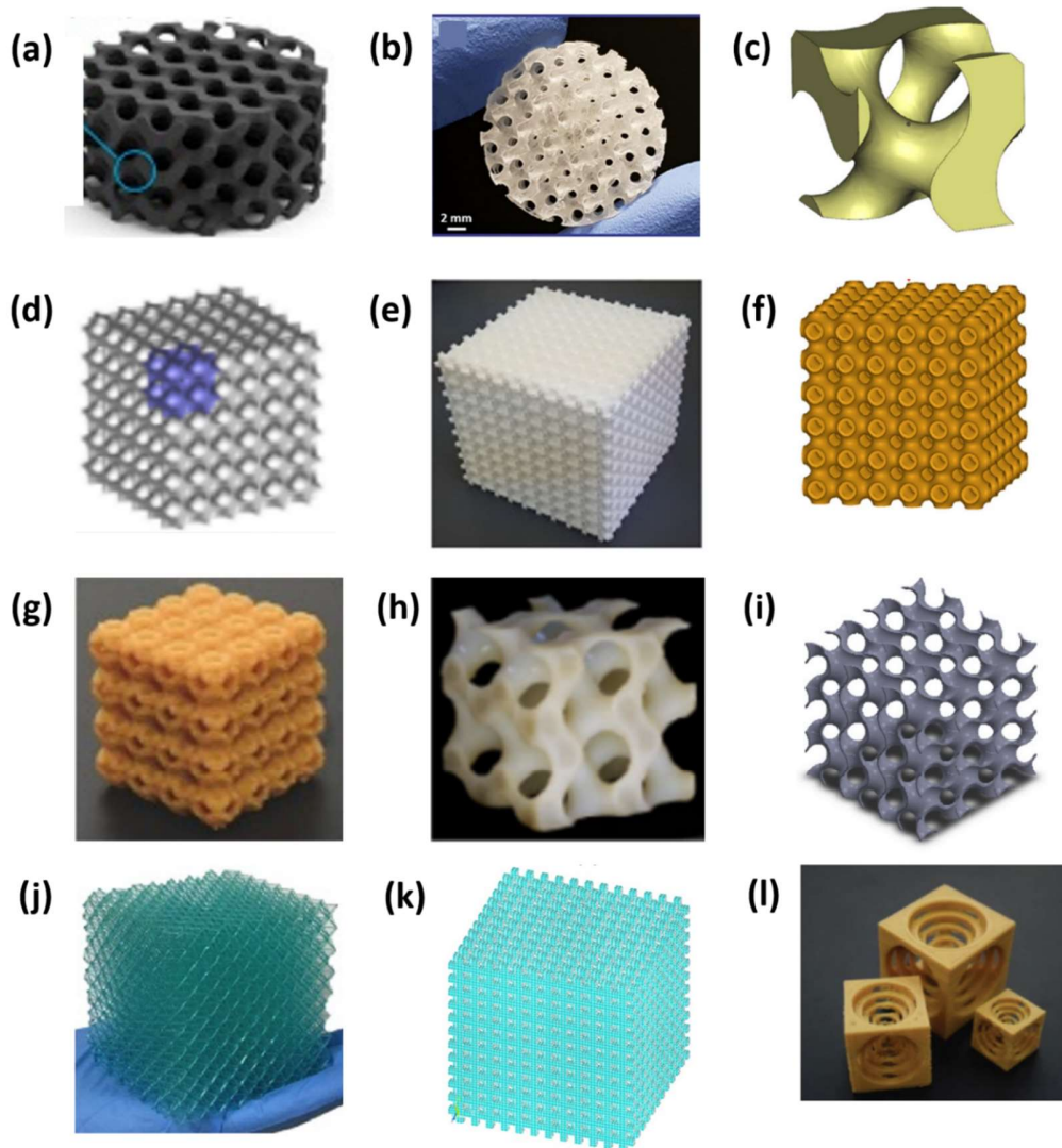
FIGURE 5. Mathematical model-based structures. (a) Surface embedded grapheme coating on a printed structure[69], (b) Scaffold with gradient porosity[70], (c) Strut-based TPMS structure[71], (d) Sheet-based TPMS structure[72], (e) Neovius cellular structure[73], (f) Solid lattice of primitive TPMS structure[74], (g) Primitive schwarzite structure[75], (h) Cellular co-continuous composite[78], (i) cellular solid-based gyroid structure[66], (j) 3D fabricated octet-truss structure with 80 mm side length[80], (k) Cubic-iso structure[67], (l) Boxception structure at multiple length scales[68].
