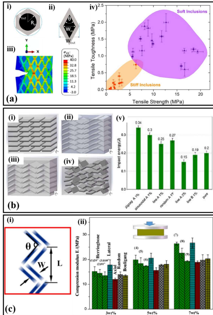
FIGURE 11. Bio-inspired composite structures. (a) (i)-(ii) Shape of circular and rhombic inclusions, respectively. R_{out} and R_{in} are the circumcircle radius of the repeat units and the radius of the inclusions, respectively. W_{out} and W_{in} is the short diagonal length of the repeat units and the short diagonal length of the inclusions respectively. (iii) Simulation of crack propagation in the rhombus filled composites ( \theta = \pi/3 ) at 0.01/s. (iv) Chart of tensile toughness versus tensile strength of Verowhite and Tangoblack composites. Triangle points and sphere points are obtained from 20% notched samples and 40% notched samples, respectively[104]. (b) Fibre arrangement patterns. (i) Linear, (ii) sinusoidal, (iii) zigzag, (iv) random. (v) Impact energy of the different fibre arrangements. 1% and 2% are the fibre weight fractions. “Pure” indicates matrix without fibres[105]. (c) (i) Schematic diagram of “herringbone” microarchitectures. (ii) Comparison of compressive modulus for different mass fractions or different embedded microstructures in different parts[106].
