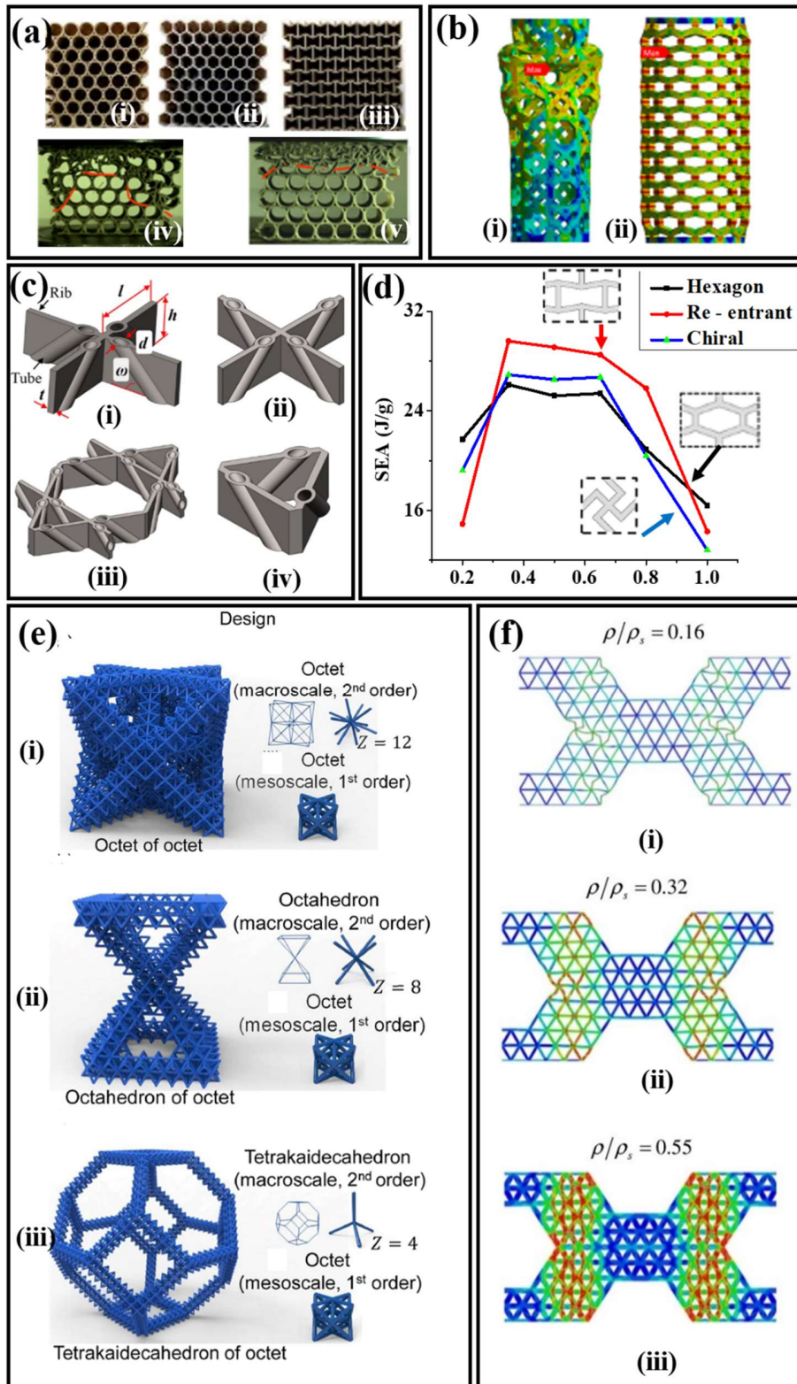
FIGURE 8. Bio-inspired cellular structures. (a) 3D printed honeycomb: circular, hexagonal and re-entrant (i)-(iii), Snapshots of compression behavior of circular honeycomb for a strain of \epsilon =
