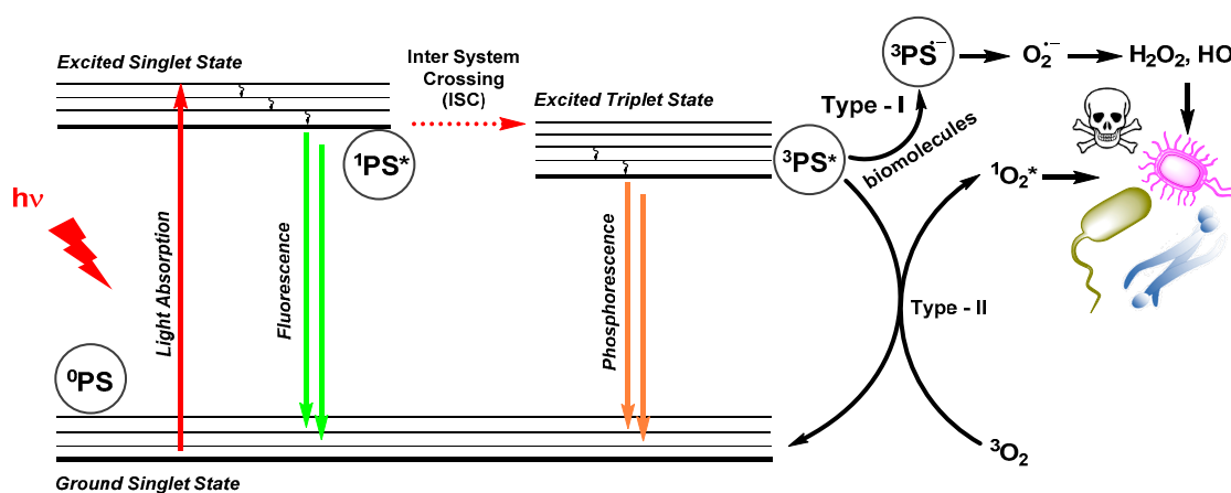
Figure 1. Simplified Jablonski diagram showing the generation of reactive oxygen species (ROS) by a photosensitizer (PS) following absorption of light, intersystem crossing and Type-I and -II mechanisms. In antimicrobial photodynamic therapy (aPDT), the resulting ROS are able to kill bacteria and fungi as illustrated on the right.
