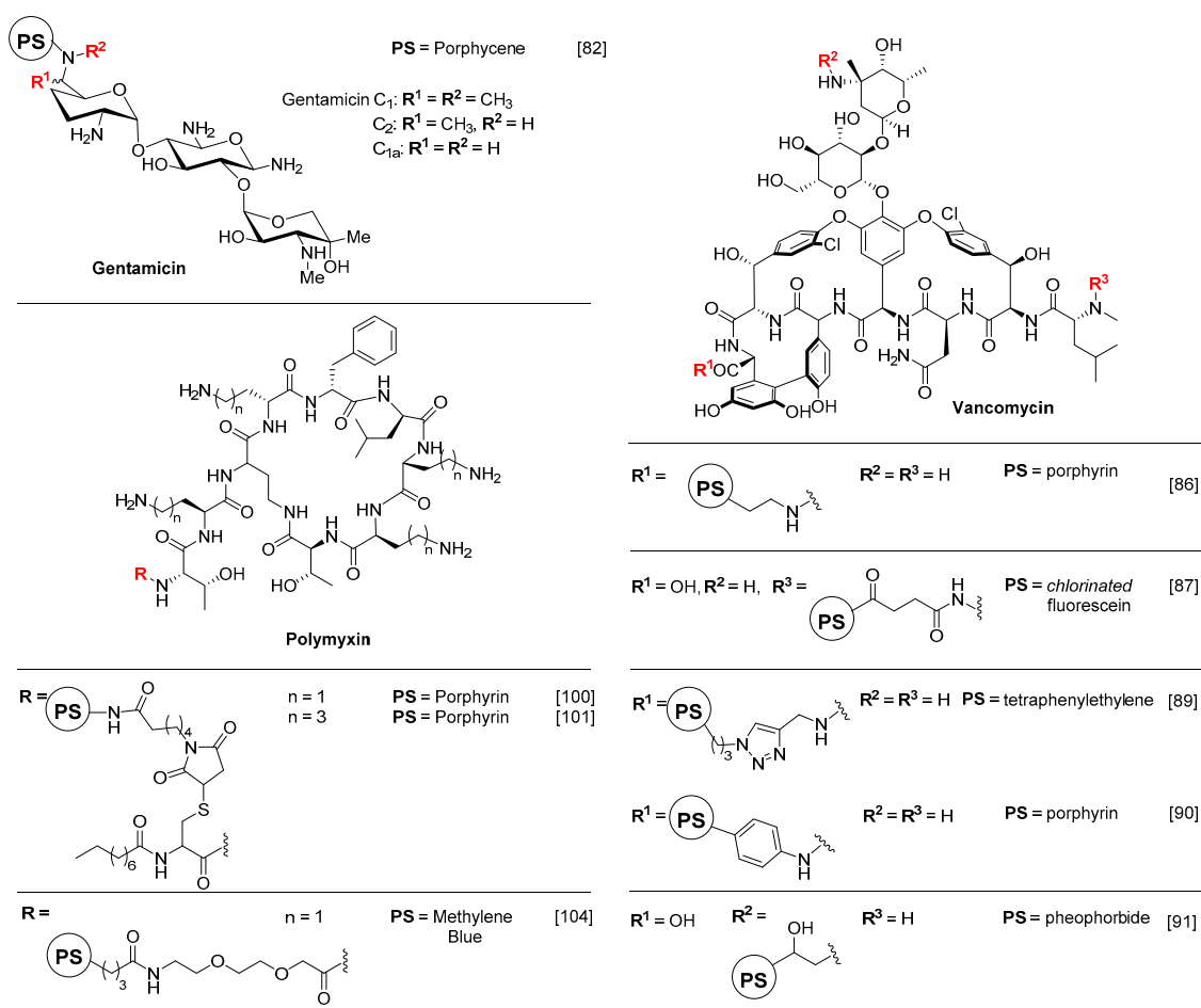
Figure 5. Recent examples of PS-conjugates using antibiotics and antimicrobial peptides (AMPs) as targeting or membrane-disrupting sub-units.
