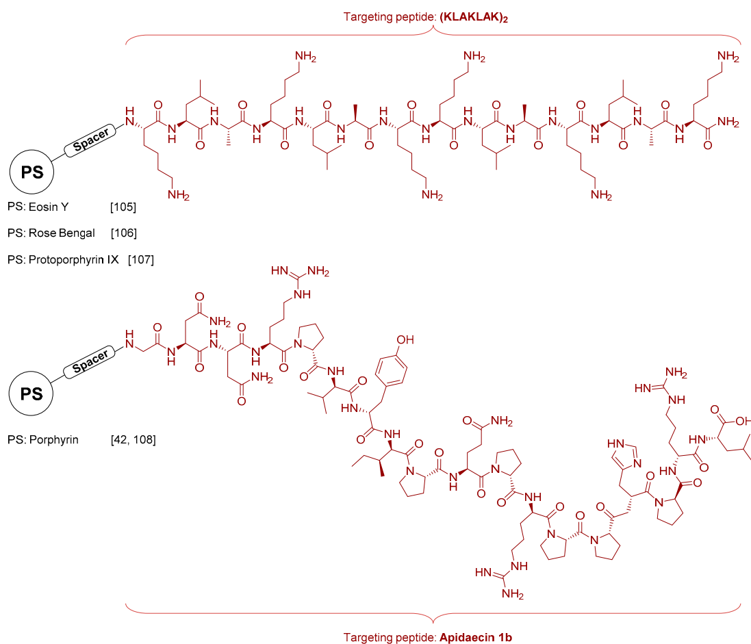
Figure 7. Examples of aPDT probes based on the AMP sequences (KLAKLAK) 2 and Apidaecin 1b conjugated to different photosensitizing units.
