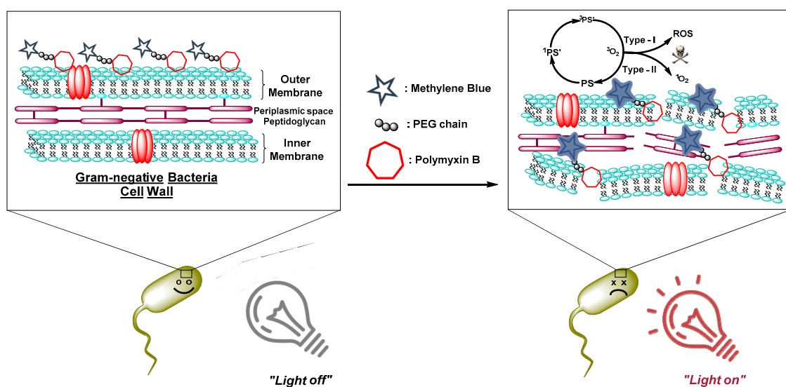
Figure 6. Illustration of the targeted aPDT treatment of Gram − bacteria with the Polymyxins (PMX)-methylene blue (MB) conjugate, during which the PMX cyclopeptide binds to the pathogen membrane and ROS are generated once the light is switched on—an example of entropically driven aPDT.
