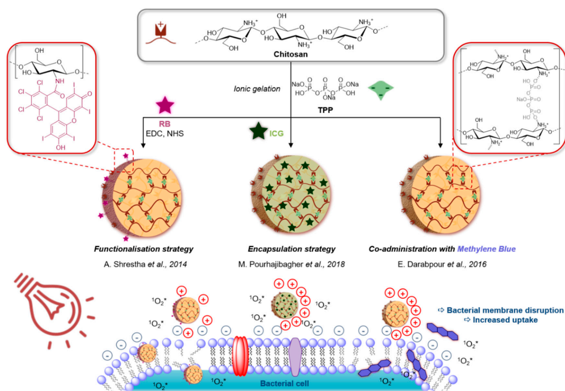
Figure 9. Examples of the preparation of chitosan nanoparticles (NPs) by ionic gelation for aPDT via covalent surface attachment [127], encapsulation [130] or co-administration, [126] of different PS.
