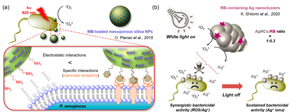
Figure 12. (a) Comparison of the bacterial specificity reported for amino- and mannose-functionalised MB-loaded mesoporous silica NPs for aPDT treatment of P. aeruginosa [153]; (b) Bactericidal modes of action of (RB)-containing silver nano-clusters during and after light irradiation [160].
