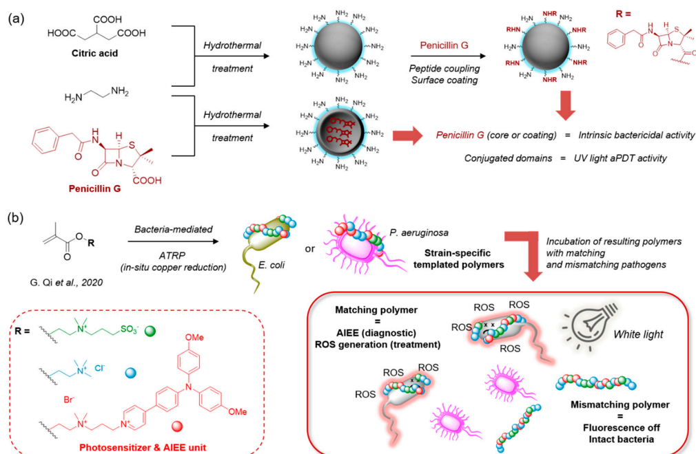
Figure 11. (a) Preparation of bactericidal ROS-generating CNPs using Penicillin G as surface targeting moiety or core carbon source [147]. (b) Example of controlled co-polymerisation of cationic, zwitterionic and PS-containing monomers mediated by bacteria, leading to template polymers able to detect and eradicate selectively their original bacterial strain [151].
