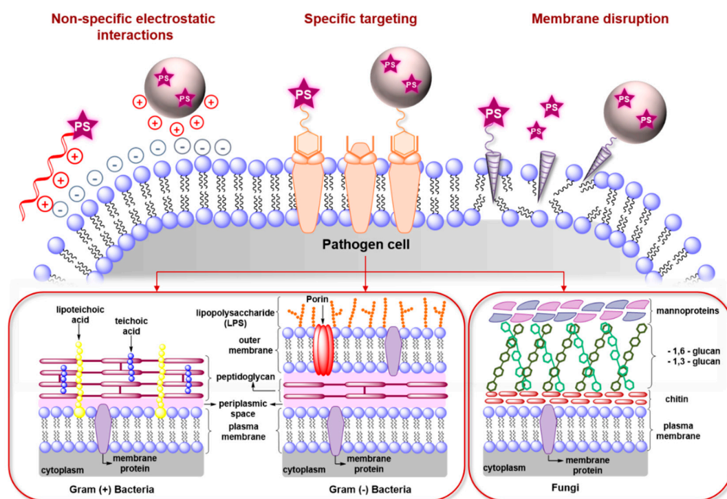
Figure 3. Different strategies applicable in the design of molecular or nano-PS targeted towards pathogens. The different designs involve the conjugation of non-specific poly-cationic materials, specific targeting ligands, or of membrane disrupting agents to known PS, either by direct conjugation to the chromophore, by using nano-carriers, or by co-administration. The lower section shows the differences between the surface of the main types of pathogens targeted by aPDT: Gram+ and Gram– bacteria and fungi.
