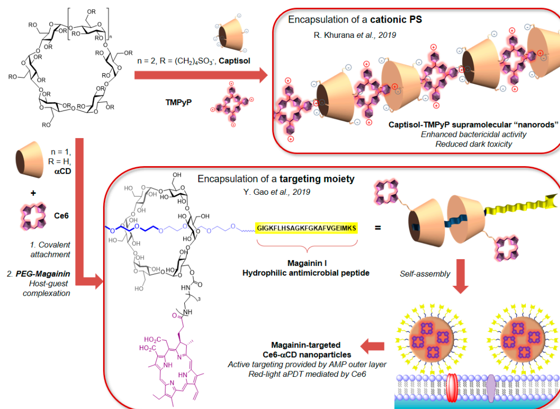
Figure 10. Examples of cyclodextrin derivatives used for the preparation of PS-containing NPs, either by encapsulation of the PS units [136], or by encapsulation of an AMP acting as a bacterial-targeting moiety [137].
