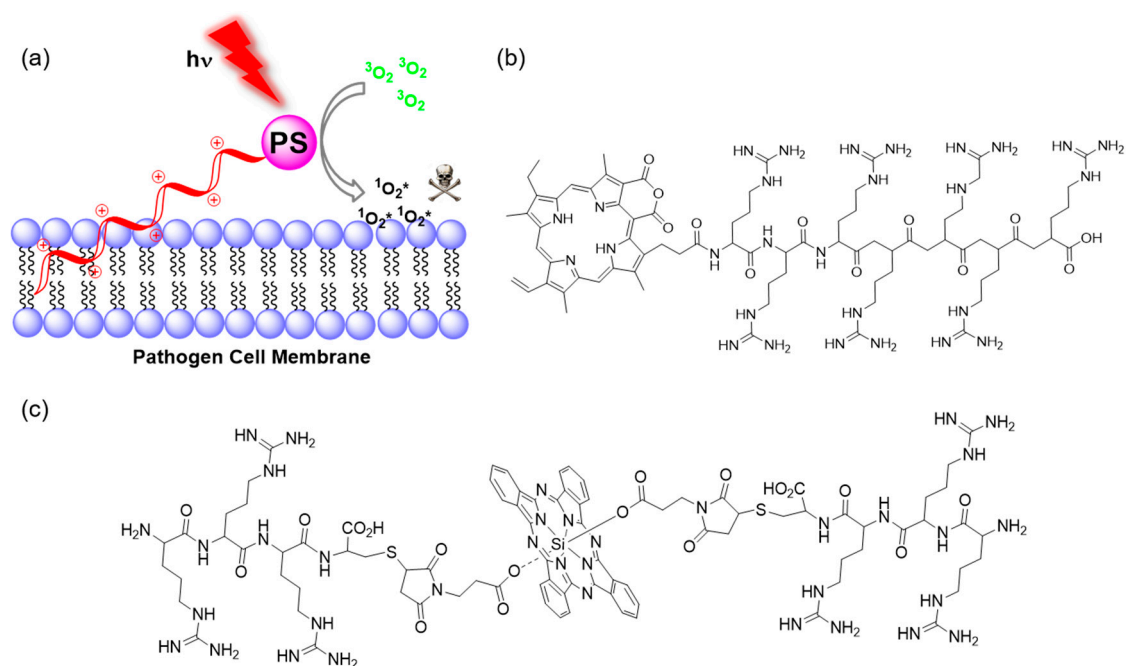
Figure 4. (a) General illustration of the interaction between the negatively-charged pathogen cell membranes with poly-cationic materials conjugated to PS building-blocks; (b) structure of the hepta-arginine-Purpurin 18 conjugate reported by Zhou et al. [70]; (c) structure of the oligo-arginine-SiPC conjugate reported by Zhao et al. [71]. Note: the stereochemistry of the peptides is undefined as it was not specified in the reports.
