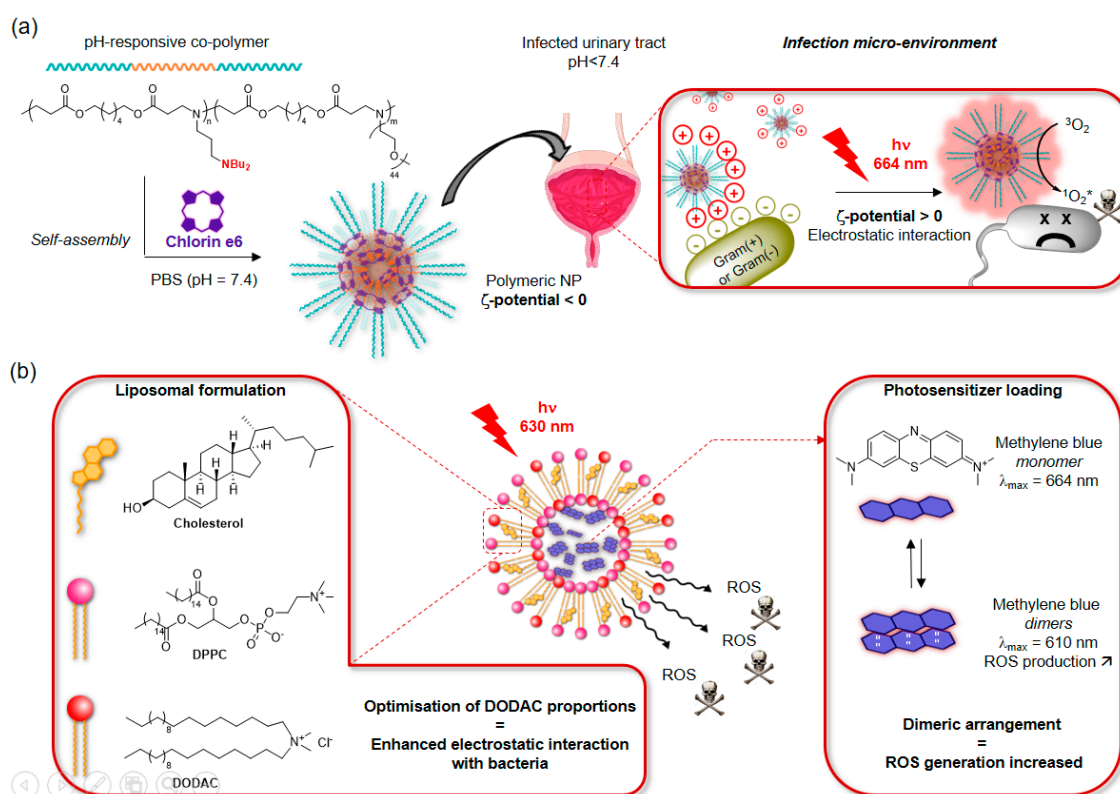
Figure 8. (a) Design of Ce6-containing pH-responsive polymeric nanoparticles for the treatment of bacterial infections in slightly acidic media such as the urinary tract [117]. (b) Example of liposomal formulation allowing both bacterial targeting via tuning of the surfactant proportions, and of the photosensitisation properties via MB loading [118].
