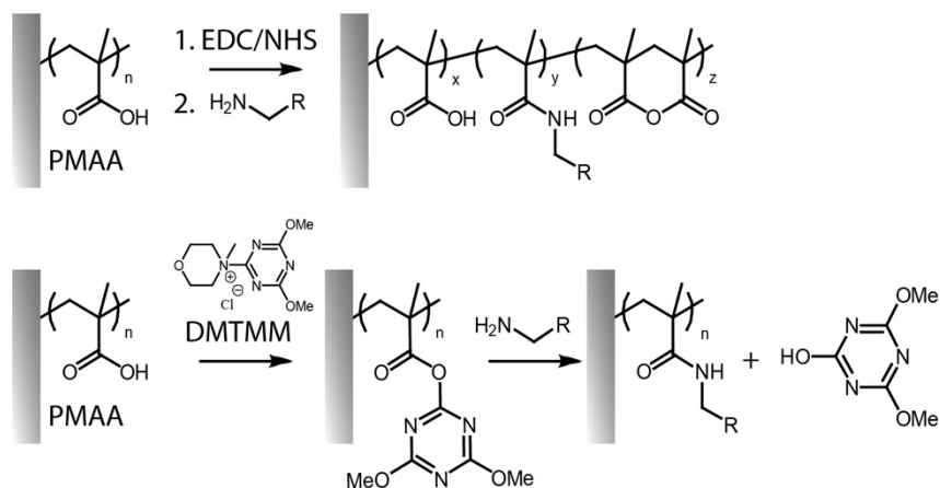
Figure 2. Activation of PMAA brushes with EDC/NHS can result in a mixture of amide, anhydride and carboxylic functions on the brush backbone (top). Coupling of amines to PMAA brushes using DMTMM as activating reagent (bottom).
