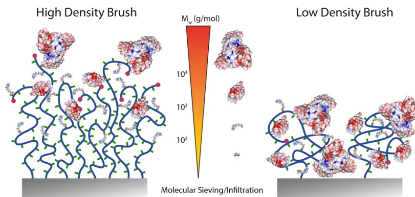
Figure 6. Schematic representation of expected functionalisation density profiles depending on the molecular weight of molecules to be coupled to dense and sparse polymer brushes.
