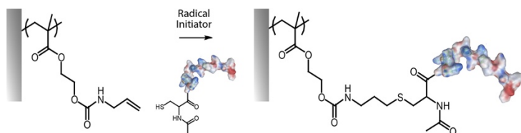
Figure 11. Example of thiol-ene radical coupling of a peptide (through a cysteine residue) to allylamine-functionalised PHEMA brushes.
