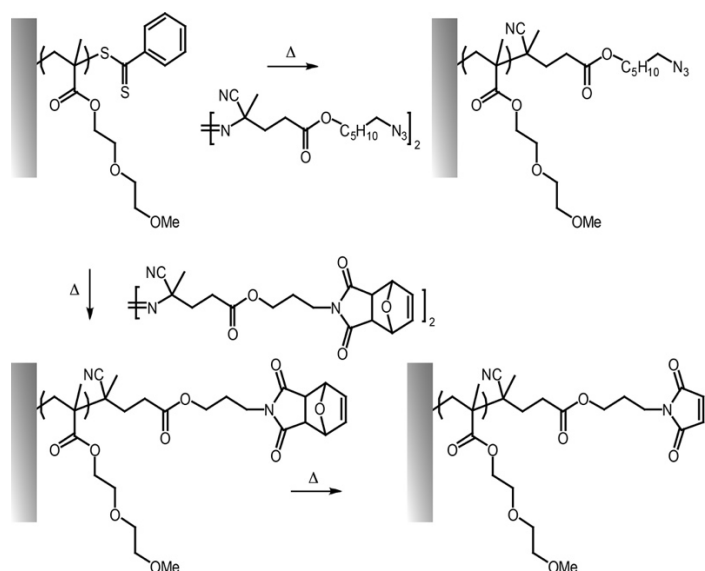
Figure 8. Examples of end chain functionalisation of polymer brushes based on the coupling of azobis-derivatives to introduce azide and maleimide residues (via retro-Diels-Alder reaction).
