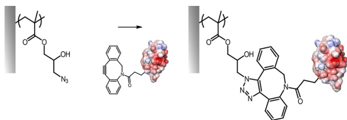
Figure 12. Example of strain-induced azide-alkyne cycloaddition for the coupling of a cyclooctyne-conjugated protein to azide-functionalised brushes.
