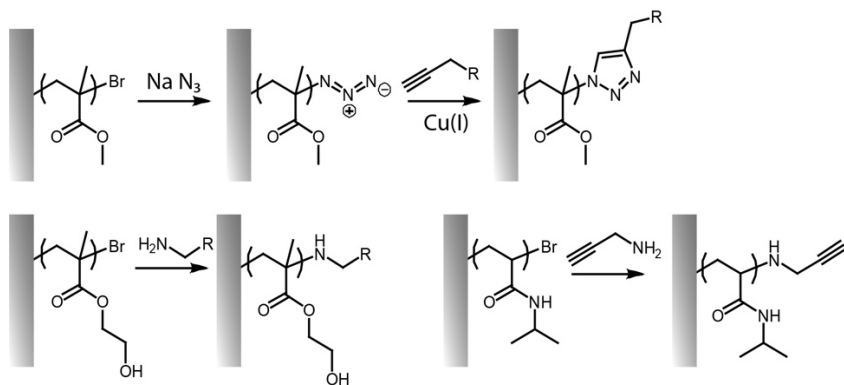
Figure 7. Examples of end-chain functionalisation of polymer brushes, based on nucleophilic substitution reactions to convert bromide end groups to reactive alkynes or azides for subsequent click reactions.
