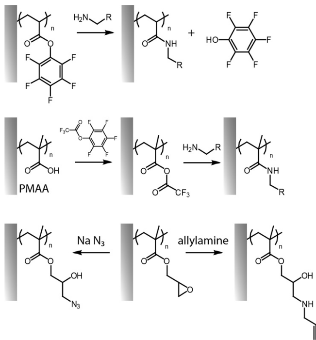
Figure 3. Functionalisation of pentafluorophenyl ester-activated brushes (top, reactive polymer; middle, for activation of carboxylic acid residues) and PGMA brushes (bottom)
