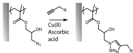
Figure 4. Coupling of alkynes on azide-functionalised PGMA brushes.
