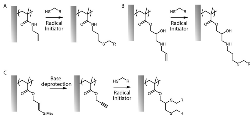
Figure 5. A and B) Two examples of thiol-ene coupling applied to allylamine post-polymerisation functionalised polymer brushes. C) Example of thiol-yne coupling to poly(propargyl methacrylate) brushes.
