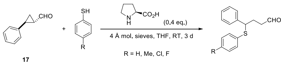
Scheme 2.19. Iminium ion driven nucleophilic ring-opening of 17
