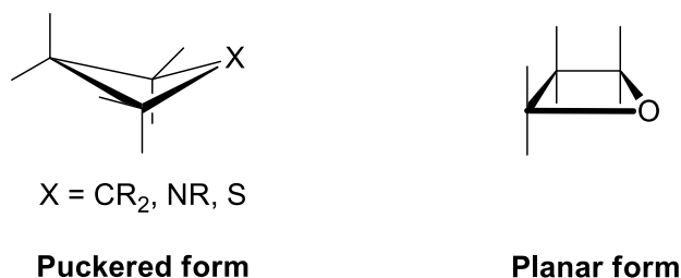
Fig. 1.7. Puckerred and planar four-membered rings
