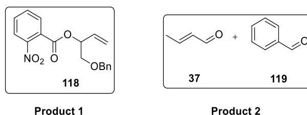
Fig. 5.6. Products from the attempted cross-coupling of 98
