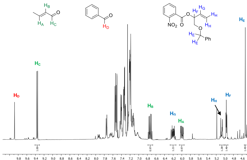
Fig. 5.7. Crude ^1\text{H} NMR of the reaction mixture showing 37 , 118 and 119
