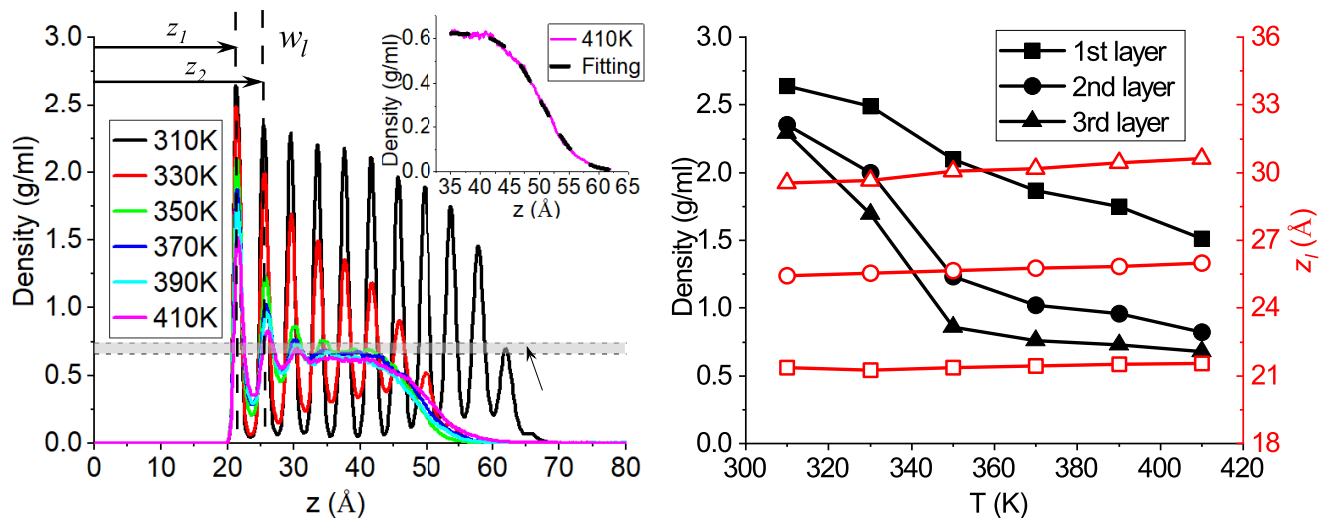
(a) Density profiles of dodecane along the direction normal to the substrate. Statistics collected from the molecules located within the middle 30 Å in x direction, with a bin width of 0.1 Å in z direction. The inset indicates the fitting of the liquid-to-vapour density at 410 K. The density of dodecane in bulk phase at 0.1 MPa and 310–410 K is 0.66–0.74 g/ml, as indicated by the grey band bounded by dashed lines.
