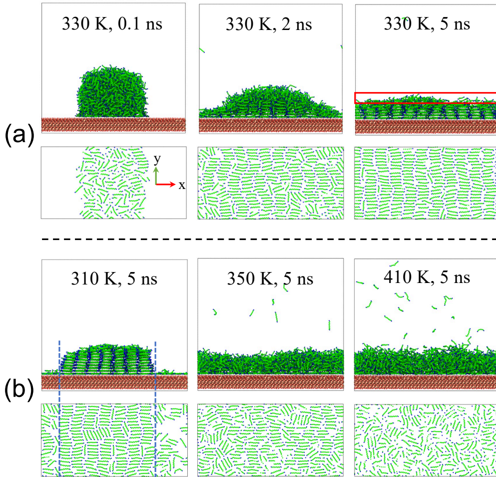
FIG. 6: (a) Time evolution of interfacial dodecane crystallisation in S1 at 330 K and the corresponding dodecane layout of the contact monolayer. The free surface is highlighted in (330 K, 5 ns). (b) Snapshots of S1 and the attached layer at different temperatures at 5 ns. The droplet boundary is indicated by blue dashed lines in (310 K, 5 ns).
