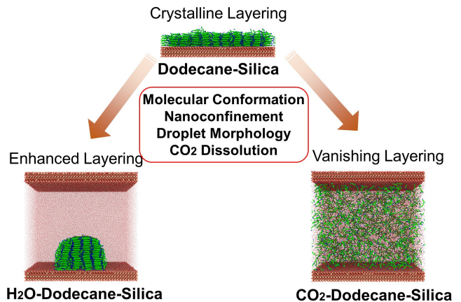
FIG. 1: Interfacial crystallisation under the impact of H 2 O and CO 2 .
