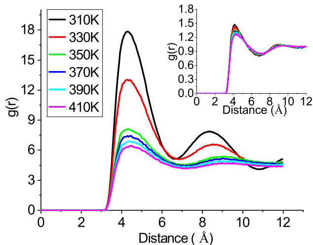
(c) RDF of dodecane -CH_3 group
