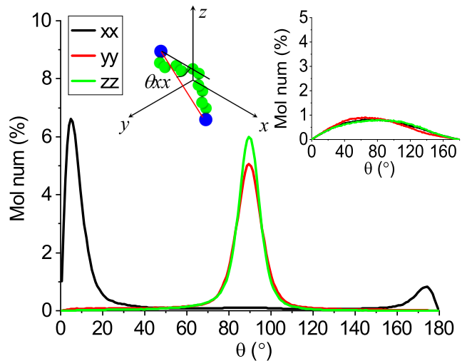
(b) PDF of molecular orientation with reference to x , y and z axes
