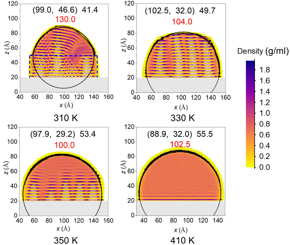
FIG. 10: 2D density contours of dodecane droplet at different temperatures in S2, averaged over the last 1 ns with the bin area equal to 0.5 \times 0.5 \text{ \AA} \times \text{ \AA} . The grey block indicates the silica substrate. The black dots indicate the data used for fitting the circle with the criterion \rho = [0.2 - 0.5] \text{ g/ml} 76 . The blue dashed box ( 9.5 \times 3.0 \text{ nm} \times \text{nm} ) is to highlight the droplet boundary. The black solid line indicates the fitted circle. The centre coordinates ( \text{\AA} , \text{\AA} ), radius ( \text{\AA} ) of the fitted circle and the contact angle \theta ( ^\circ ) are also indicated.
