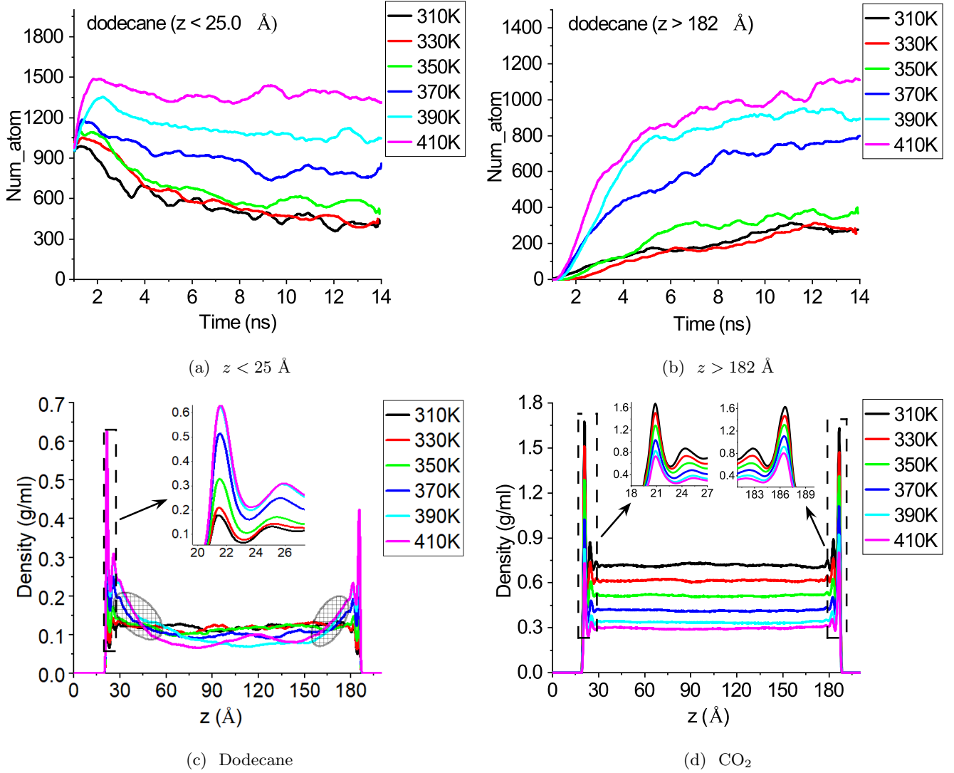
FIG. 13: Statistics of S3. In 13a and 13b: Time evolution of the number of dodecane molecules in specific regions in z direction. The data is averaged over a 10 ps interval. In 13c and 13d: Density profiles in z direction at 15 ns. The transition from surface adsorption to the free layer is highlighted in shadowed regions.
