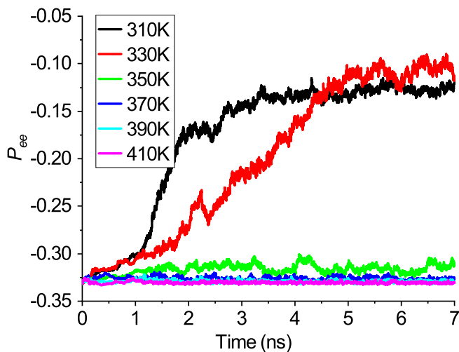
(a) Time evolution of the orientational order of dodecane molecules
