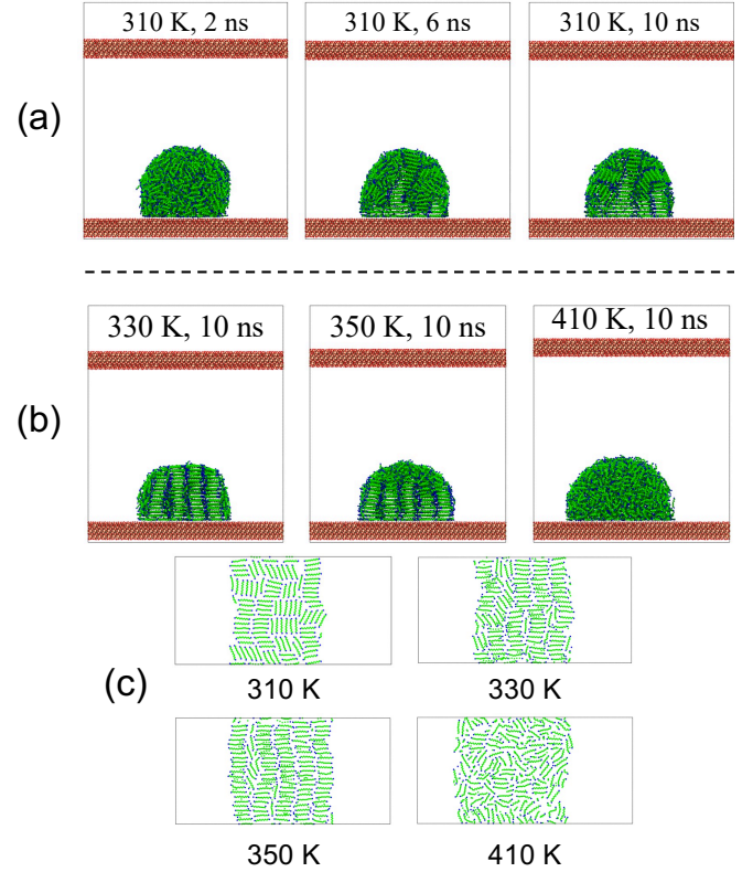
FIG. 9: (a) Time evolution of dodecane droplet in S2 at 310 K. H 2 O molecules are hidden. (b) Dodecane morphology at 330, 350 and 410 K at 10 ns. (c) The layout of dodecane molecules of the contact layer at 310, 330, 350 and 410 K at 10 ns.
