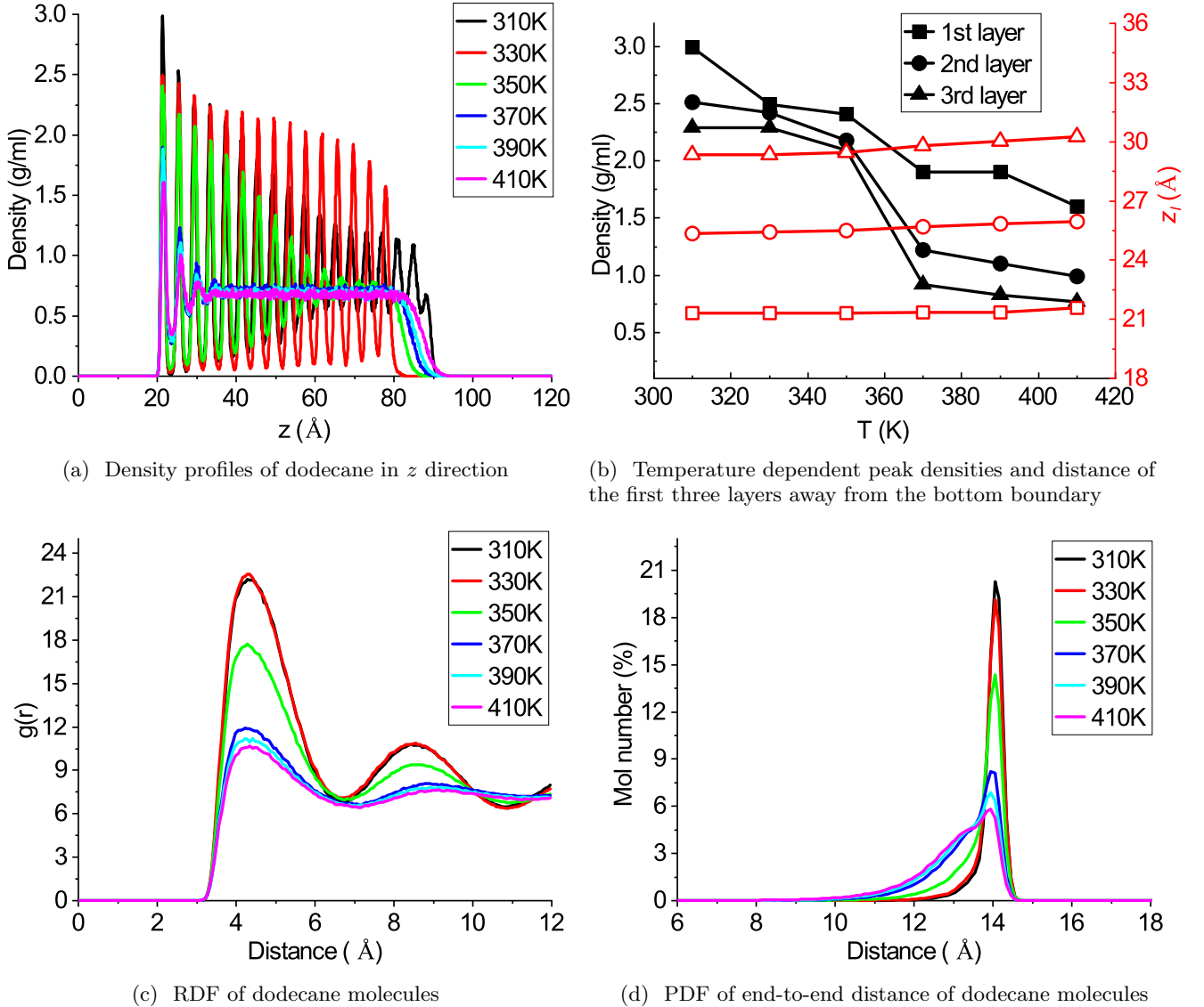
FIG. 11: Statistics in S2.
