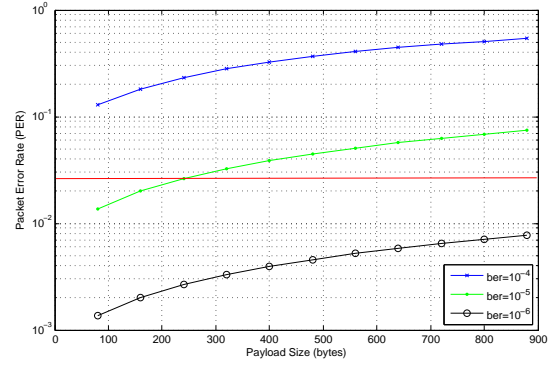
Figure 7.3: PER estimation for WLAN VoIP in different channel condition
