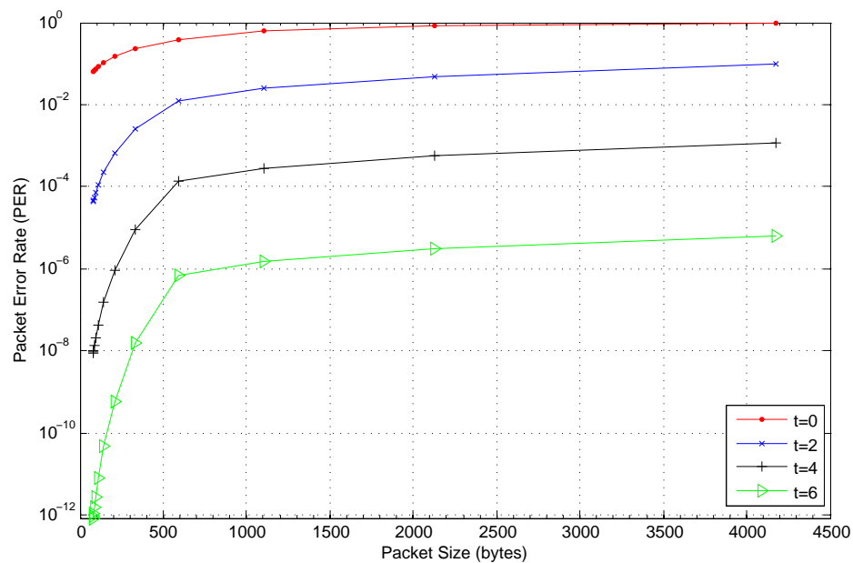
Figure 5.2: PER estimation with FEC for different error correction strength when \text{BER}=10^{-4}
