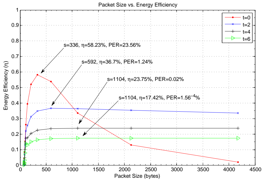
Figure 5.1: Energy efficiency estimation with FEC with different error correction strength for \text{BER}=10^{-4}
