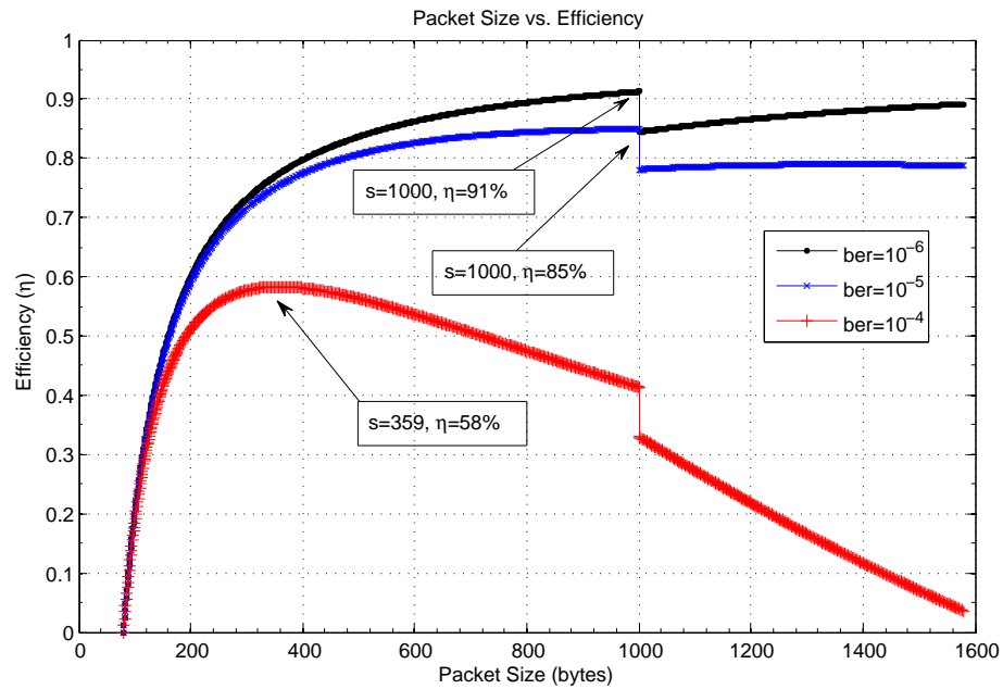
Figure 4.3: Optimal packet size estimation in a noisy channel for three different BER
