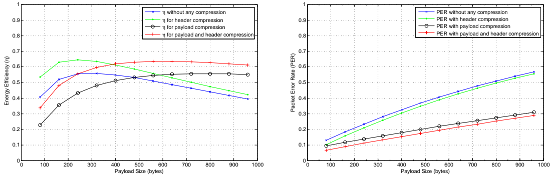
Figure 7.6: Energy efficiency and PER comparison for compression with BER 10^{-4}
