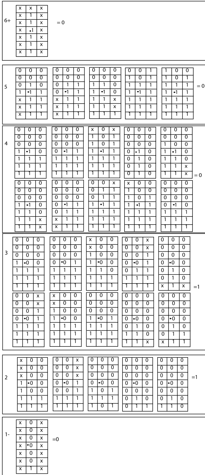
Figure 6: The local rule table for \Gamma_{(1)}^{(0)} . The number on the left of each rectangle represents the number of ones in the reference column. An 'x' represents a cell that can have any value. The · represents the central cell. Only configurations where the central cell changes are listed.
