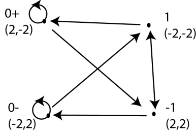
Figure 3: The graph G defines a subshift on its bi-infinite paths.
