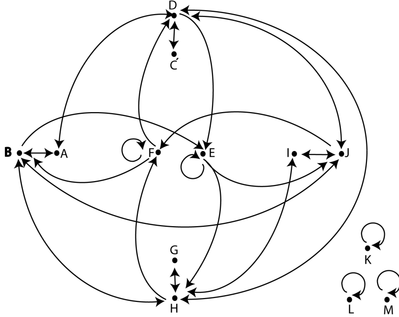
Figure 4: The graph \mathcal{H} . See Table 3 for definitions of the vertices.
