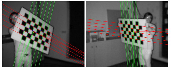
Figure 9: Example detections in 176 \times 144 rof amplitude images. The yellow dot (one-pixel radius) is the estimated centroid of the board, and the attached thick translucent lines are the estimated axes. The board on the right, which is relatively distant and slanted, was not detected by OpenCV.
