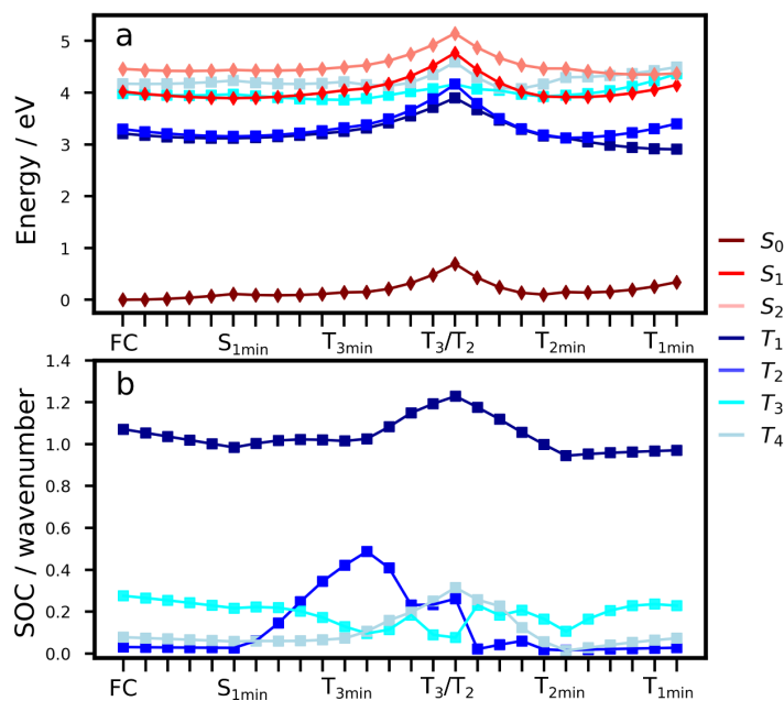
Fig. 2 (a) Linear interpolated Cartesian coordinates pathway (LICC) from the Franck-Condon (FC) geometry, to S 1 , to the excited state minima (OEC model, TD-B3LYP/6-311++G(d,p)) (b) Spin-orbit couplings values along the LICC pathway.
