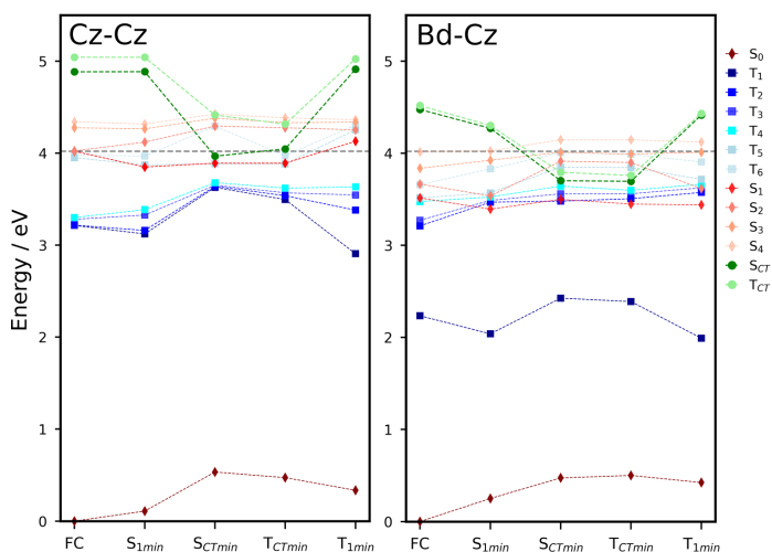
Fig. 5 Energy profiles for singlet and triplet states, including the \text{Cz}^- \text{Cz}^+ and \text{Cz}^- \text{Bd}^+ charge transfer states ( S_{CT} and T_{CT} ) computed at the critical points for the dimer A embedded in the crystal environment using the OEC model.
