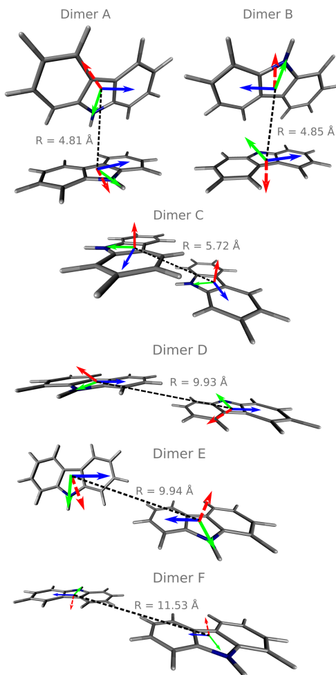
Fig. 3 Molecular dimers in the Cz crystal optimised at the TD-B3LYP/6-311++G(d,p) level using the OEC model. Distances between the centre of masses ( R ) are also shown. The green, blue and red arrows represent the transition dipole moments of the S_0 \rightarrow S_1 , S_0 \rightarrow S_2 and the T_1 \rightarrow S_0 transitions, respectively. The arrow lengths are not proportional to the transition dipole magnitudes.
