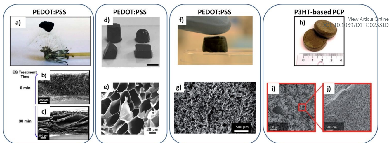
Figure 5 : Different PCP states and their macroporous structure observed by SEM. a - c) ultra-low density PEDOT:PSS cryogel placed on top of a dandelion and SEM characterizations of the gel before and after treatment with EG; 21 d - e) Digital pictures of PEDOT:PSS hydrogels with different geometric shapes (scale bars = 1 cm) and cross-section SEM image of a freeze-dried PEDOT:PSS hydrogel and after the treatment with concentrated H_2SO_4 ; 10 f - g) PEDOT:PSS, GOPS, and NFC PCP composite and SEM image of the internal structure; 25 h - j) P3HT "foam" and its internal porous structure characterized by SEM. 28 All panels have been reproduced with permission from J. APPL. POLYM. SCI. (a-c), Adv. Mater. (d-e), Adv. Funct. Mater. (f-g and h-j).
