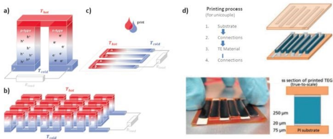
Figure 3: Schematics of (a) a thermoelectric element, which comprises one n - and one p -type thermoelectric leg that experience a temperature gradient \Delta T = T_{hot} - T_{cold} leading to charge accumulation at the cold ends, (b) a conventional thermoelectric module that comprises an array of elements, which are connected electrically in series but thermally in parallel, and (c) an in-plane (printable) array of elements. generators (according to ref. 77 reproduced with permission from the Royal Society of Chemistry). From the perspective of applications, thermoelectric generators (TEGs) containing a large number of thermoelectric p - and n -type legs connected in series are needed to achieve considerable power output. Bulk PCPs are compatible with vertical device geometry. d) From the perspective of evaluating the performances of a material, connecting in series vertical mono leg TEG (only one type of polymer) can be easily produced. In this case, a conductive electrode (gold or silver paste) is replacing the second type of leg. The printing sequence, scheme of a
