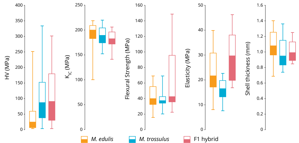
Figure 1. Boxplots comparing the phenotypes flexural strength, shell thickness, elasticity, hardness and fracture toughness to identified genotypes. The Boxplots show Q2, median and Q3 of samples and the whiskers indicate maximum and minimum values of each repeat for each sample. No statistically significant differences were identified between the genotypes by micro-indentation (HV, Hardness p = 0.75 ; K_{IC} , fracture toughness p = 0.10 ; M. edulis N = 11, F1 hybrids N = 2 and M. trossulus N = 6; see Table 2) or three-point bending tests (Flexural strength p = 0.2 , elasticity p = 0.27 , shell thickness p = 0.50 ; M. edulis N = 18, F1 hybrids N = 2 and M. trossulus N = 3; see Table 3).
