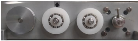
Fig. 2. Pulley system, from left to right: distance encoder, load cell, support pulley, stepper motor.
