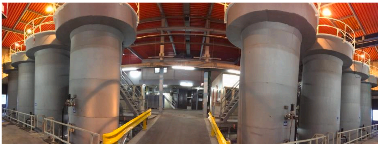
Fig. 1. Full-scale pellet softening reactors located at Waternet (Amsterdam, The Netherlands) [10].
