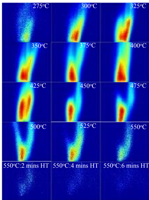
Figure 3. PAH PLIF images with increasing temperature for the 550 °C HT condition and for maintaining HT for up to 6 minutes for WS. Red colour denotes higher concentration and blue lower one
