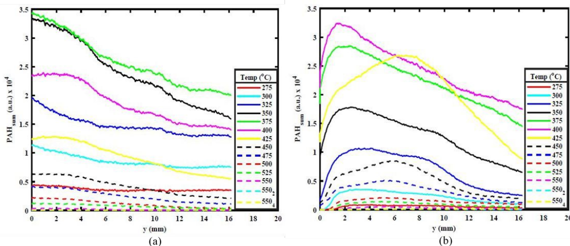
Figure 4. PAH_{sum} for different temperatures and heights above reactor bed for 550 HT condition for (a) AS and (b) WS.
