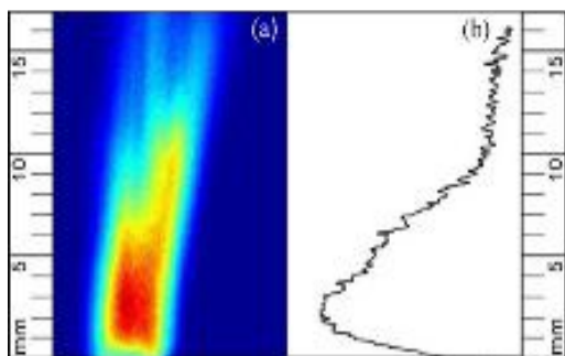
Figure 2. (a) Background corrected PAH PLIF image and (b) PAH_{sum} profile expressed as a function of height. Red colour denotes higher concentration and blue lower one.
