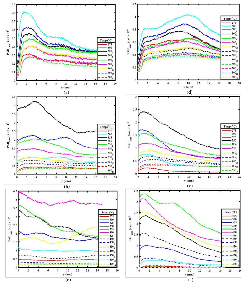
Figure 5. PAH_{sum} profiles for different holding temperatures for the two biomass samples, AS ((a) 300 °C, (b) 350 °C and (c) 450 °C) and WS ((i) 300 °C, (ii) 350 °C, (iii) 450 °C (I would suggest these are mad d, e, f instead of roman numerals for consistency). The subscript in the legend indicates the number of minutes the sample is held once (HP) once the desired holding temperature is reached.
