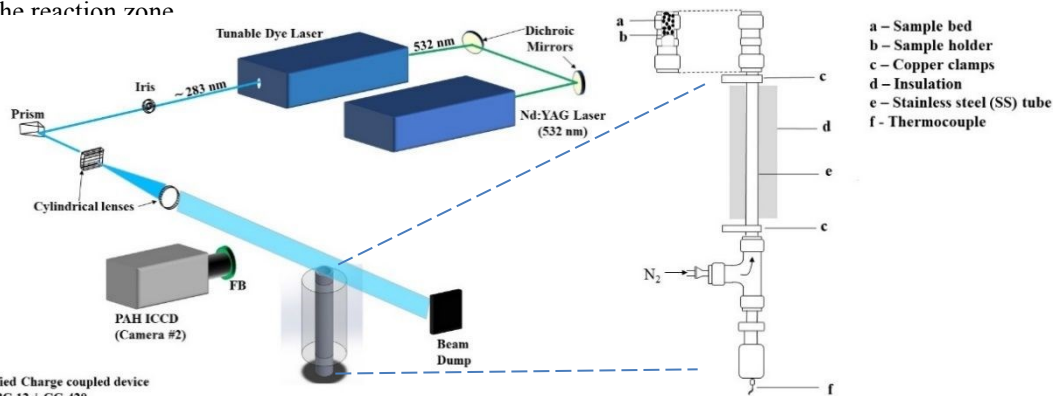
Figure 1. Schematics of experimental setup and reactor set up Ref. 21 and briefly described here. PAHs were excited using the 532 nm output from an Nd: YAG laser (Litron Nano PIV) to pump a tunable dye laser containing Rhodamine 6G dye. The fundamental wavelength
