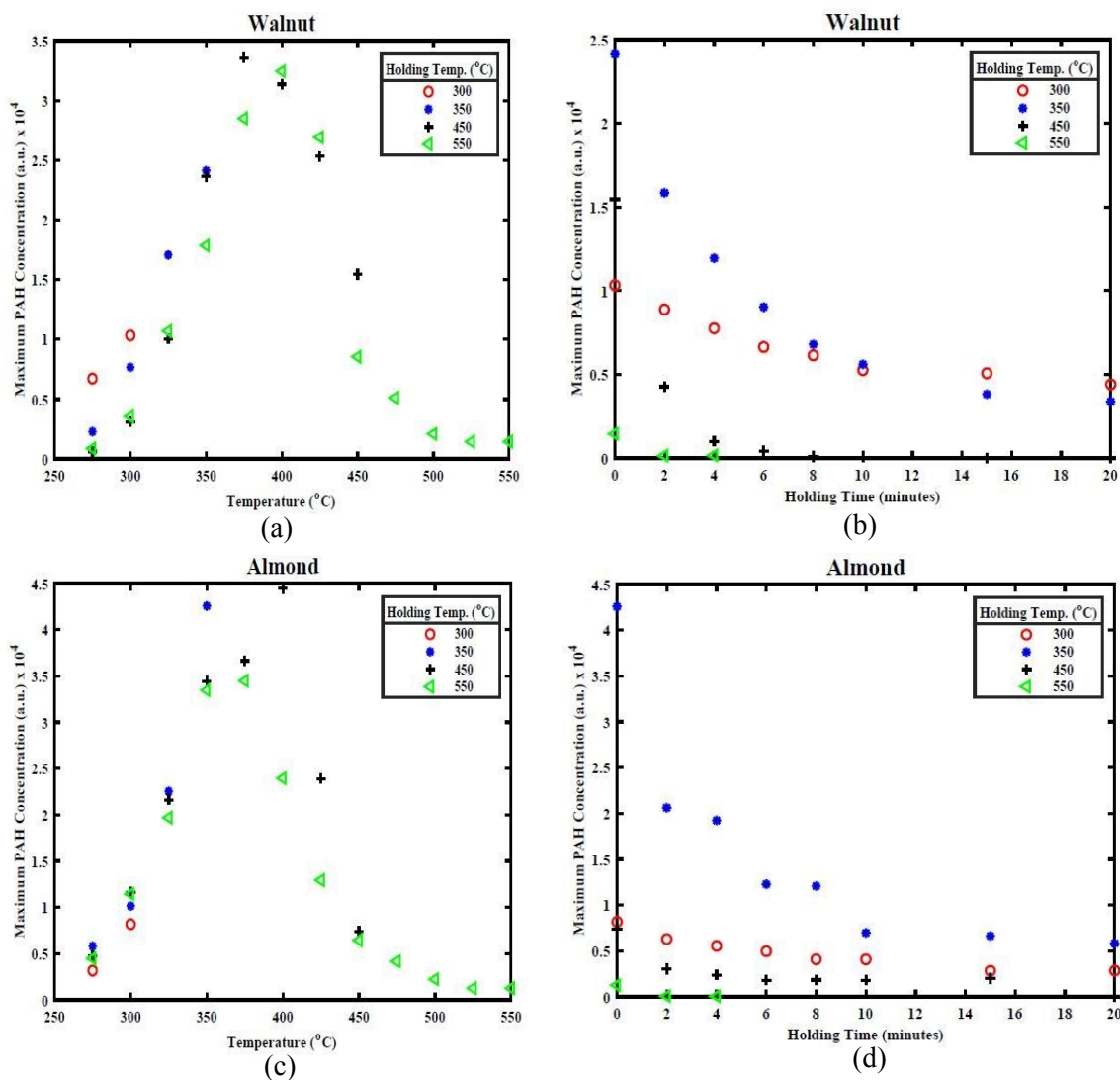
Figure 6. Maximum PAH concentration (representing maximum PAH LIF signal) for different (a) and (c) holding temperatures and (b) and (d) holding period.
