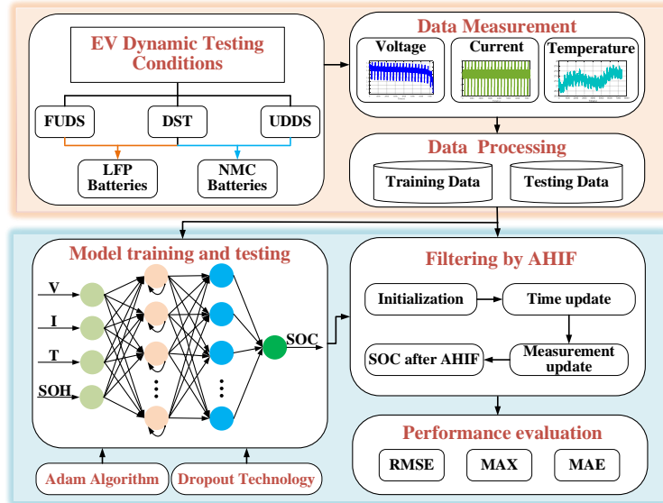
Fig. 2. The SOC estimation framework incorporating LSTM network and AHIF.
