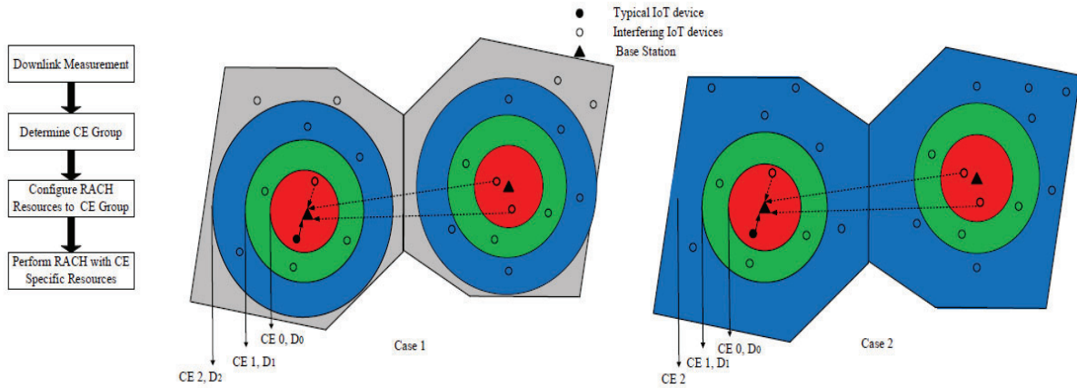
Fig. 1: NB-IoT CE Groups
