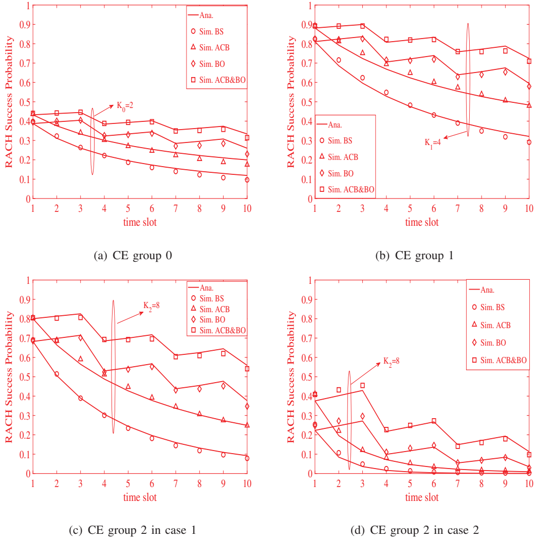
Fig. 6: RACH success probability for three CE groups in each time slot with four RACH schemes
