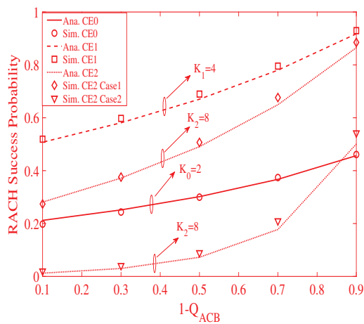
Fig. 7: RACH success probability at the 5th time slot versus ACB factors
