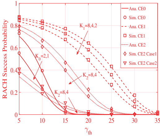
Fig. 3: RACH success probability for three CE groups versus \gamma_{th} in the 1st time slot Fig. 4: RACH success probability for three CE groups and single CE group
