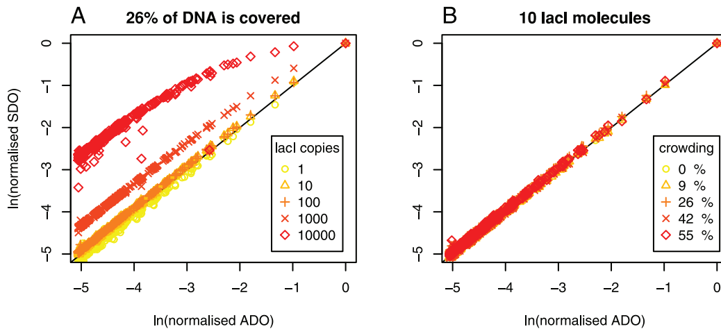
Figure 1. ADO and SDO for various abundances of lacI and crowding on the DNA. We considered the case of the lac repressor TF and 100 Kbp of DNA, which contains the O_1 site. Each system was simulated for T_I = 3000 s (which is the average cell cycle time of E.coli [31,45]) and, for each set of parameters, we considered X = 40 independent simulations. We considered only the sites that have the binding energy at least 70% of the highest value (the strongest 437 sites). (A) Five different lacI copy numbers: (i) 1, (ii) 10, (iii) 100, (iv) 1000 and (v) 10000. We assumed the case of 3 \times 10^4 copies of non-cognate TFs, which leads to 26% of the DNA being covered. (B) Five different non-cognate copy numbers: (i) 0, (ii) 1 \times 10^4 , (iii) 3 \times 10^4 , (iv) 5 \times 10^4 and (v) 7 \times 10^4 , and 10 copies of lacI. doi:10.1371/journal.pone.0073714.g001
