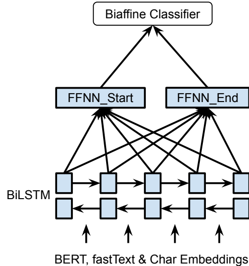
Figure 1: The network architectures of our system.
