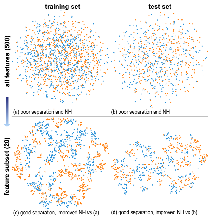
Figure 2. Madelon dataset. (a) Training set (NH: 53.9%). (b) Test set (NH: 50.97%). (c) Training set, feature subset (NH: 83.56%). (d) Test set, feature subset (NH: 74.15%).
