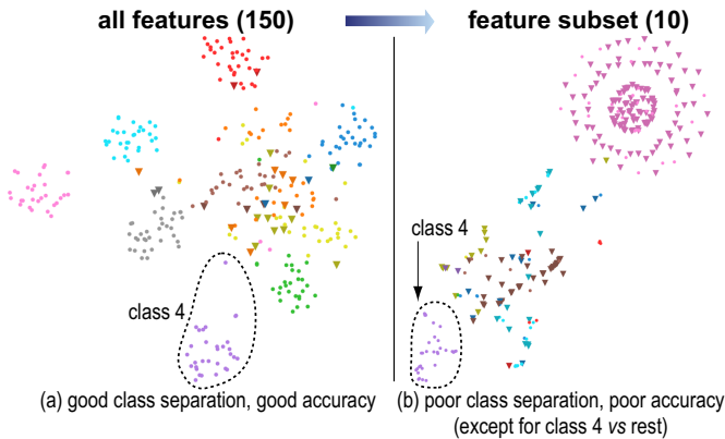
Figure 7. Corel classification. (a) RFC (AC: 91.81%). (b) RFC, feature subset (AC: 34.55%, 4 vs rest AC: 99.7%).
