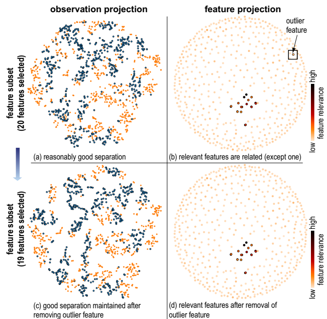
Figure 12. Madelon training set. (a,b) Observation and feature projections, 20 features selected (NH: 83.56%). (c,d) Observation and features projections, one less feature (NH: 84.55%).
