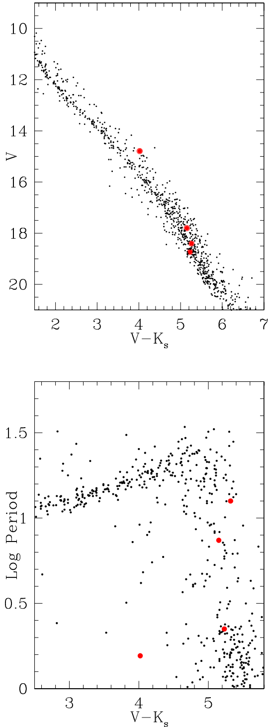
Figure 1. Color – magnitude diagram ( top ) and color – rotation period diagram ( bottom ) illustrating the location of the four new eclipsing systems relative to the sequence of Praesepe members. Top : From brightest to faintest are: AD 1508, AD 3814, AD 2615, and AD 3116 with elevation above the color-magnitude sequence a rough indicator of the mass ratio of a binary system (equal mass ratio produces a 0.75 mag magnitude excess). Bottom : from slowest to fastest rotators are: AD 2615, AD 3814, AD 3116 and AD 1508.
