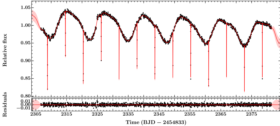
Figure 11. Systematics-corrected K2 light curve of AD 2615 (black points) with the GP-EBOP model in red. The red line and pink shaded region represent the mean and 2\sigma uncertainty of the model’s predictive posterior distribution.
