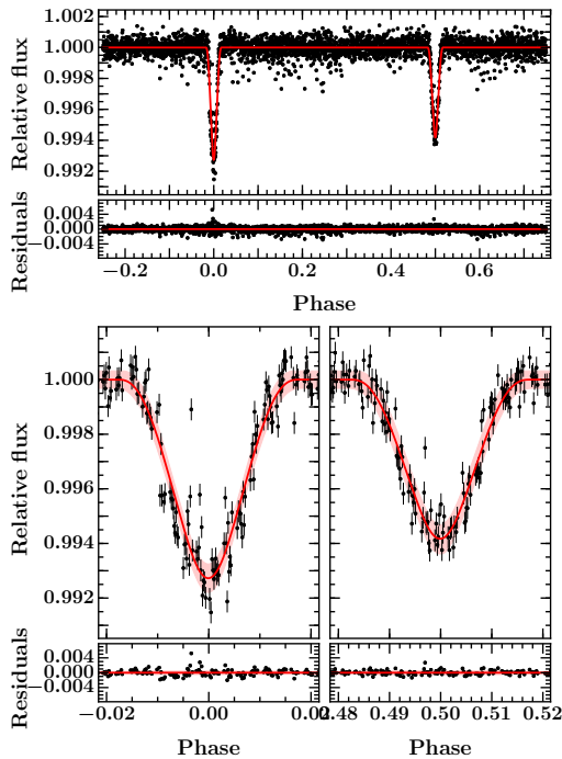
Figure 20. Top panels: phase-folded K2 light curve of AD 1508 (black), which has been detrended with respect to the Gaussian process model. The red line indicates the median EB model derived from the posterior distribution, i.e. individual draws are calculated across phase space and the median of their paths plotted. Phase zero marks the center of the primary eclipse. Immediately below are the residuals of the fit. Bottom panels: zooms on primary and secondary eclipses ( left and right respectively) with the median model and 2\sigma uncertainties shown (red line and pink shaded region, respectively). Residuals are shown immediately below.
