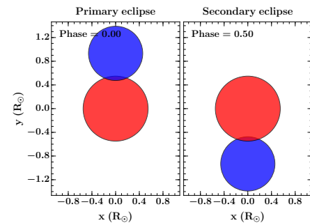
Figure 22. Geometry of AD 1508, to scale, as observed at primary and secondary eclipse. The primary star is shown in red and the secondary in blue.
