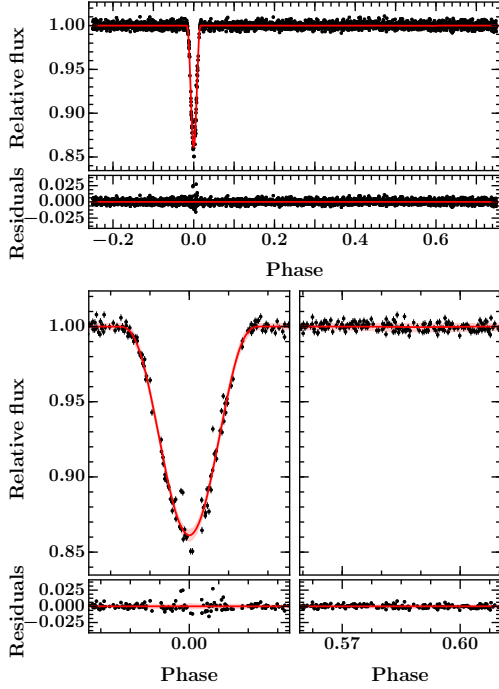
Figure 16. Top panels: phase-folded K2 light curve of AD 3116 (black), which has been detrended with respect to the Gaussian process model. The red line indicates the median EB model derived from the posterior distribution, i.e. individual draws are calculated across phase space and the median of their paths plotted. Phase zero marks the center of the primary eclipse. Immediately below are the residuals of the fit. Bottom panels: zooms on primary and secondary eclipses ( left and right respectively) with the median model and 2\sigma uncertainties shown (red line and pink shaded region, respectively). Residuals are shown immediately below.
