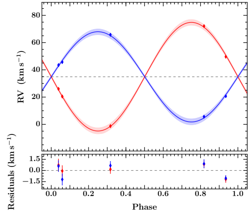
Figure 13. Top : phase-folded RV orbit of AD 2615 with Keck/HIRES RVs for the primary and secondary stars (red and blue, respectively). The lines and shaded regions indicate the median and 2\sigma uncertainty on the posterior distribution of the RV orbits. The gray horizontal dotted line shows the systemic velocity. Bottom : Residuals of the fit.
