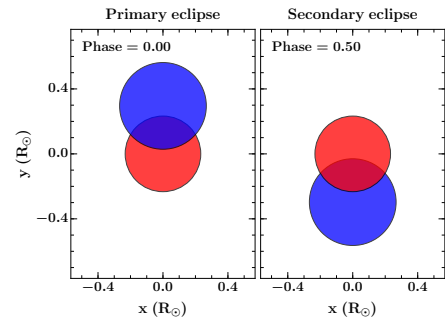
Figure 14. Geometry of AD 2615, to scale, as observed at primary and secondary eclipse. The primary star is shown in red and the secondary in blue.
