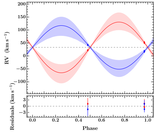
Figure 21. Top : phase-folded RV orbit of AD 1508 with Keck/HIRES RVs for the primary and secondary stars (red and blue, respectively). The lines and shaded regions indicate the median and 2\sigma uncertainty on the posterior distribution of the RV orbits. The gray horizontal dotted line shows the systemic velocity. Bottom : Residuals of the fit.
