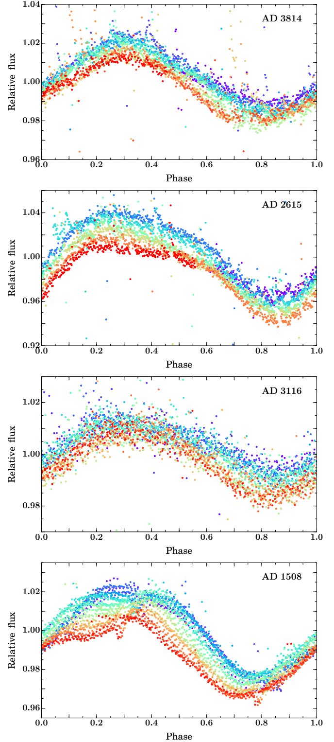
Figure 3. Evolution of the photometric modulation observed in ADs 3814, 2615, 3116 and 1508 ( top to bottom ). The systematics-detrended K2SC light curves shown in Figure 2 have been folded on the period of the observed variability. The rainbow color scheme highlights the evolution through the 75 day campaign ( beginning to end , violet to red). For ADs 3814, 2615, 3116 and 1508, the number of periods folded upon are 11, 7, 34 and 49, respectively, which simply reflects the orbital periods of the systems.
