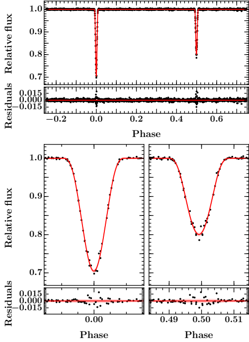
Figure 8. Top panels: phase-folded K2 light curve of AD 3814 (black), which has been detrended with respect to the Gaussian process model. The red line indicates the median EB model derived from the posterior distribution, i.e. individual draws are calculated across phase space and the median of their paths plotted. Phase zero marks the center of the primary eclipse. Immediately below are the residuals of the fit. Bottom panels: zooms on primary and secondary eclipses ( left and right respectively) with the median model and 2\sigma uncertainties shown (red line and pink shaded region, respectively). Residuals are shown immediately below.
