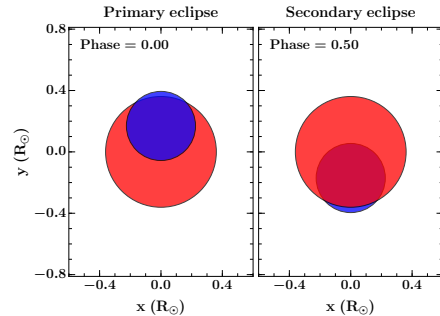
Figure 10. Geometry of AD 3814, to scale, as observed at primary and secondary eclipse. The primary star is shown in red and the secondary in blue.
