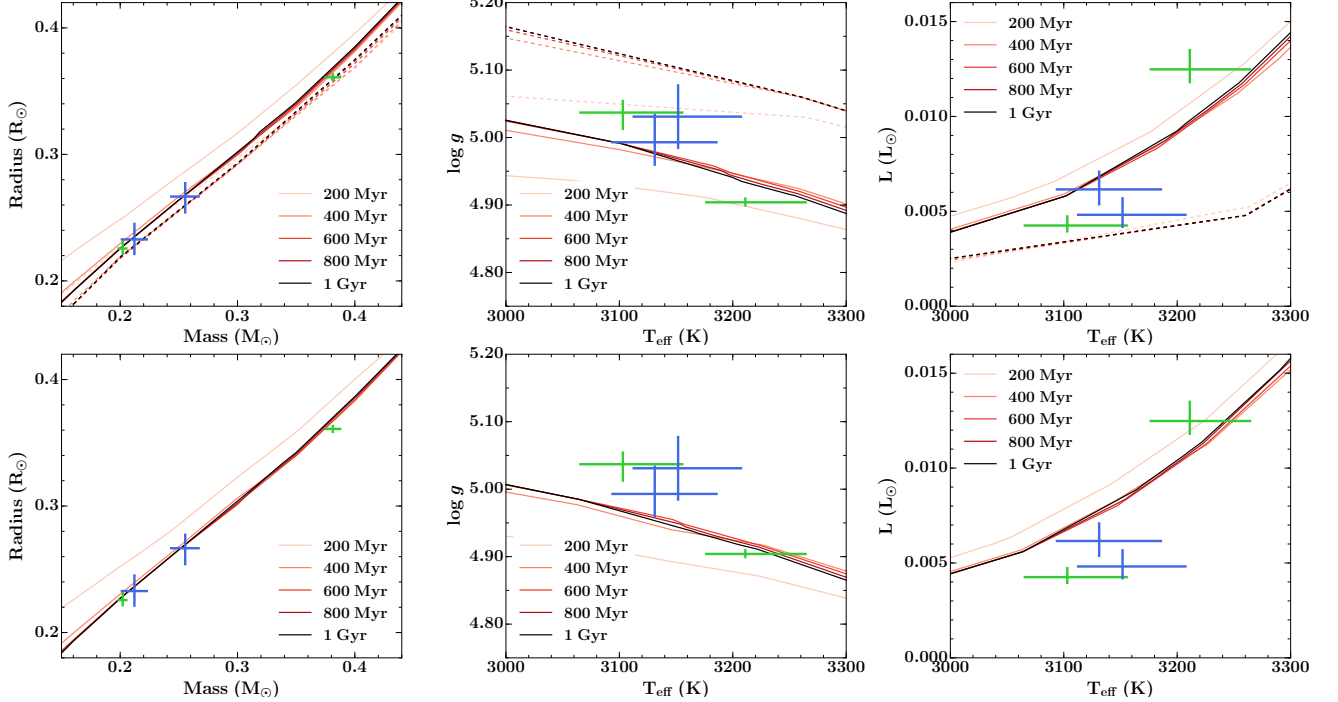
Figure 5. Comparison of the fundamental parameters of ADs 3814 and 2615 (green and blue, respectively) to the PARSEC v1.2 and BHAC15 model isochrones (solid and dashed lines, respectively). The top row shows the PARSEC (solid) and BHAC15 (dashed) models in the mass–radius, T_{\text{eff}}\text{--}\log g and T_{\text{eff}}\text{--}L planes ( left to right ) at solar metallicity. The bottom row shows the same planes but for the PARSEC models at the metallicity of Praesepe ( Z = 0.0174 ). The model isochrones shown are common in all plots and range from 200 Myr (lightest) to 1 Gyr (darkest).
