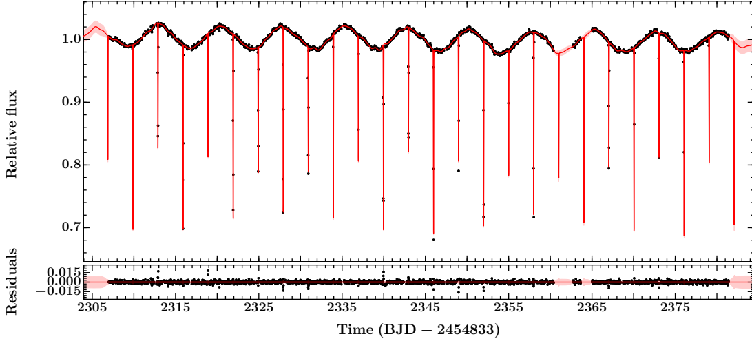
Figure 7. Systematics-corrected K2 light curve of AD 3814 (black points) with the GP-EBOP model in red. The red line and pink shaded region represent the mean and 2\sigma uncertainty of the model’s predictive posterior distribution.
