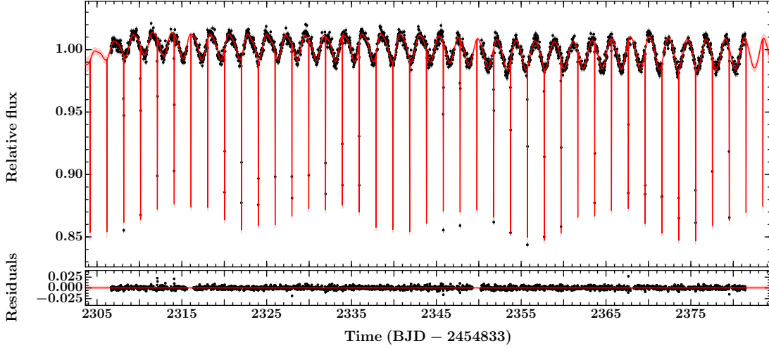
Figure 15. Systematics-corrected K2 light curve of AD 3116 (black points) with the GP-EBOP model in red. The red line and pink shaded region represent the mean and 2\sigma uncertainty of the model’s predictive posterior distribution.
