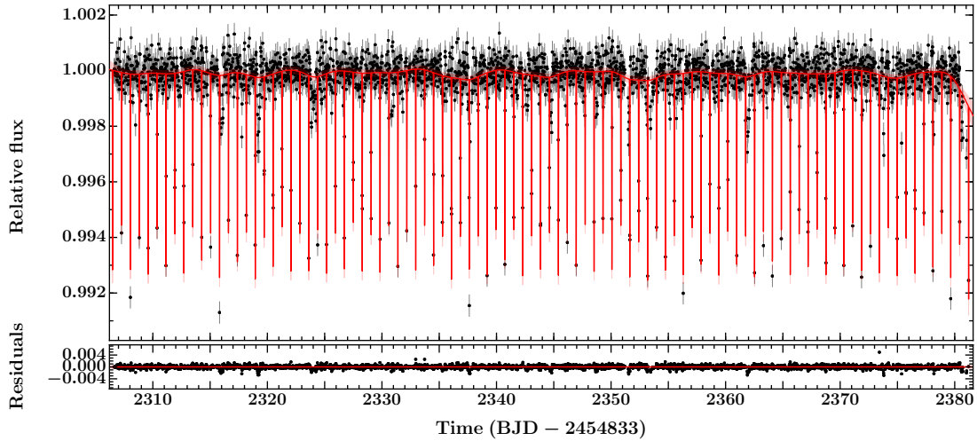
Figure 19. Systematics-corrected K2 light curve of AD 1508 (black points) with the GP-EBOP model in red. The red line and pink shaded region represent the mean and 2\sigma uncertainty of the model’s predictive posterior distribution.
