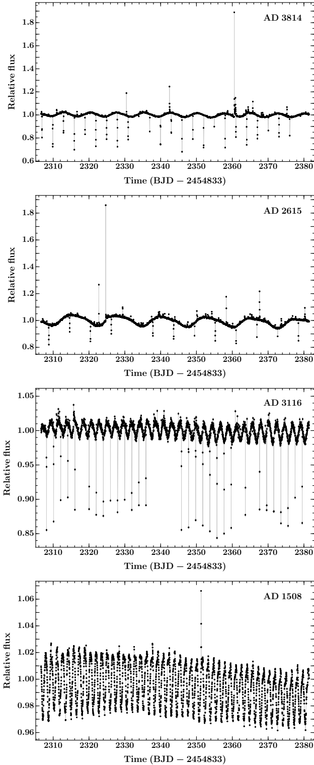
Figure 2. Systematics-detrended K2SC PDC light curves of ADs 3814, 2615, 3116 and 1508 ( top to bottom ). Each system shows out-of-eclipse variations arising from evolving starspot modulation upon which the stellar eclipses are superposed. Numerous stellar flares are visible throughout the observations, most notably on ADs 3814 and 2615, including one in each system reaching a relative flux \gtrsim 1.8 . Missing eclipses, as seen in AD 3116, are an artifact present in the PDC light curves.
