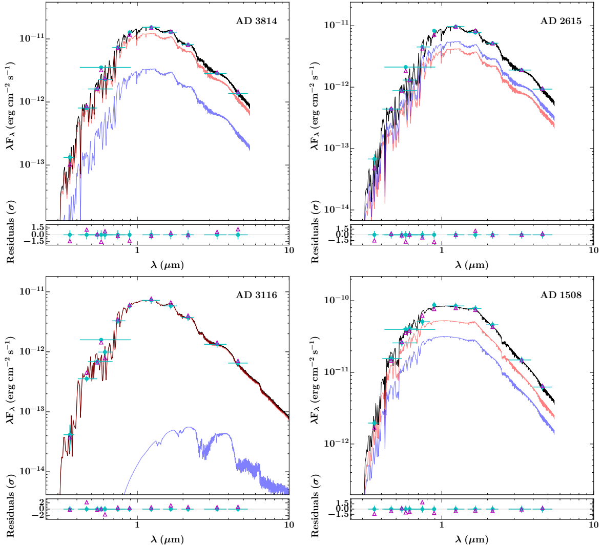
Figure 4. Spectral energy distributions (SEDs) of the four new EBs. Clockwise from top left : ADs 3814, 2615, 1508 and 3116. Cyan points represent the observed SED, which has been constructed from the broadband magnitudes reported in Table 1 (horizontal error bars indicate each band’s spectral coverage). The primary and secondary star spectra are shown in red and blue, respectively. Their combined spectrum is shown in black and the hollow magenta triangles show the combined model convolved with the ugriz , V , K p , JHK and WISE 1&2 bands. The models shown for ADs 3814, 2615 and 1508 are the PHOENIX v2 models as these produce a better fit to the data than the BT-SETTL models. However, we show the BT-SETTL models for AD 3116 as the PHOENIX models do not extend to low enough temperatures to explain the secondary component.
