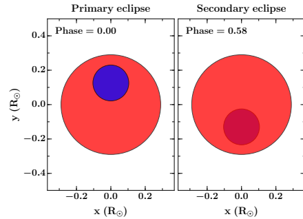
Figure 18. Geometry of AD 3116, to scale, as observed at primary and secondary eclipse. The primary star is shown in red and the secondary in blue.
