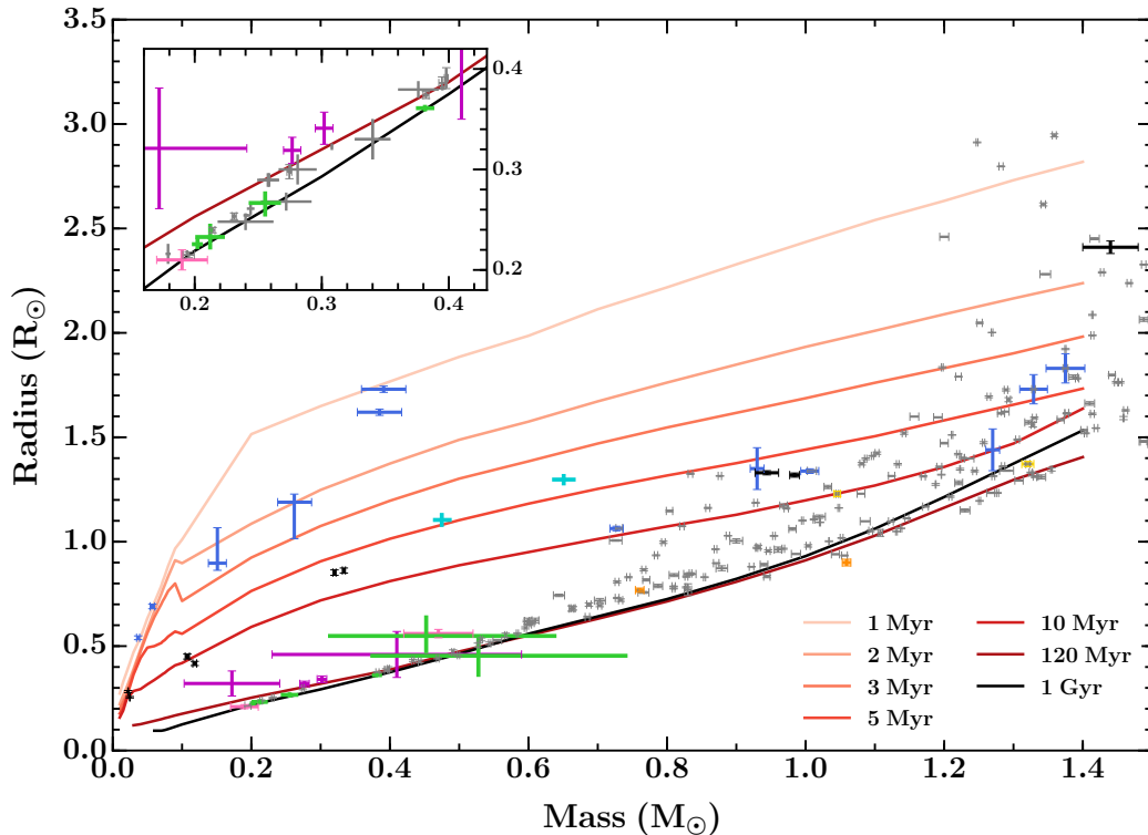
Figure 6. Mass-radius relation for detached double-lined eclipsing binaries (EBs) below 1.5 M_{\odot} . Data compiled from Table 5 and DEBCat ( http://www.astro.keele.ac.uk/~jkt/debdata/debs.html ). EBs that are members of open clusters are colored while field EBs are shown in gray. The clusters containing well-characterized EBs are Orion (blue), Upper Scorpius (black), NGC 2264 (cyan), Pleiades (magenta), Hyades (orange), NGC 1647 (pink), Per OB2 (gold), and the new Praesepe EBs (green) presented here. The colored lines represent solar metallicity isochrones of Baraffe et al. (2015) from 1 Myr to 1 Gyr (top to bottom). Inset (top left) is a zoom on the region containing ADs 3814 and 2615 to allow a closer comparison between the models and current observational constraints for low-mass stars. Here we also include the compilation of known low-mass EBs presented in Dittmann et al. (2017).
