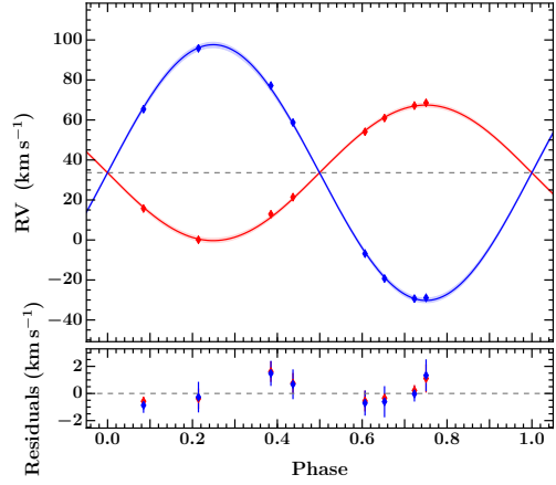
Figure 9. Top : phase-folded RV orbit of AD 3814 with Keck/HIRES RVs for the primary and secondary stars (red and blue, respectively). The lines and shaded regions indicate the median and 2\sigma uncertainties on the posterior distributions of the RV orbits. The gray horizontal dotted line shows the systemic velocity. Bottom : Residuals of the fit.
