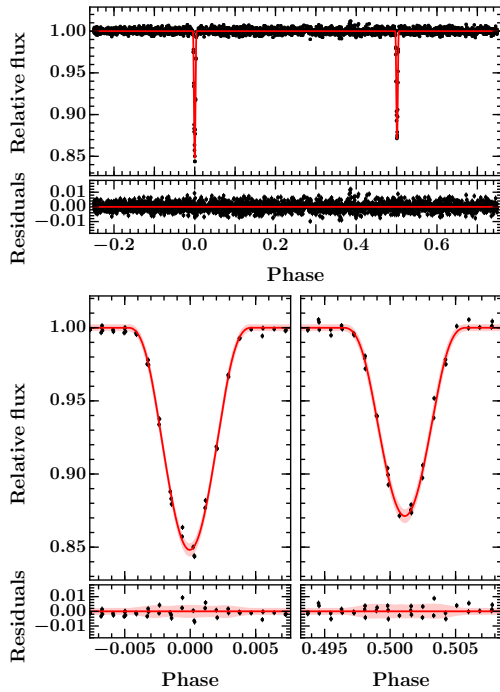
Figure 12. Top panels: phase-folded K2 light curve of AD 2615 (black), which has been detrended with respect to the Gaussian process model. The red line indicates the median EB model derived from the posterior distribution, i.e. individual draws are calculated across phase space and the median of their paths plotted. Phase zero marks the center of the primary eclipse. Immediately below are the residuals of the fit. Bottom panels: zooms on primary and secondary eclipses ( left and right respectively) with the median model and 2\sigma uncertainties shown (red line and pink shaded region, respectively). Residuals are shown immediately below.
