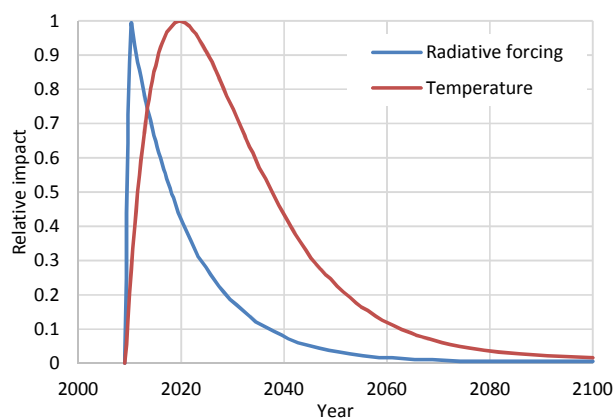
Figure 2. The relative impact of a pulse emission of methane on radiative forcing and subsequent impact on temperature change. Source: 14
