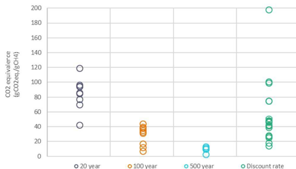
Figure 7. CO 2 equivalence of methane for different time horizons and compared to metrics which use discount rates instead of time horizons.
