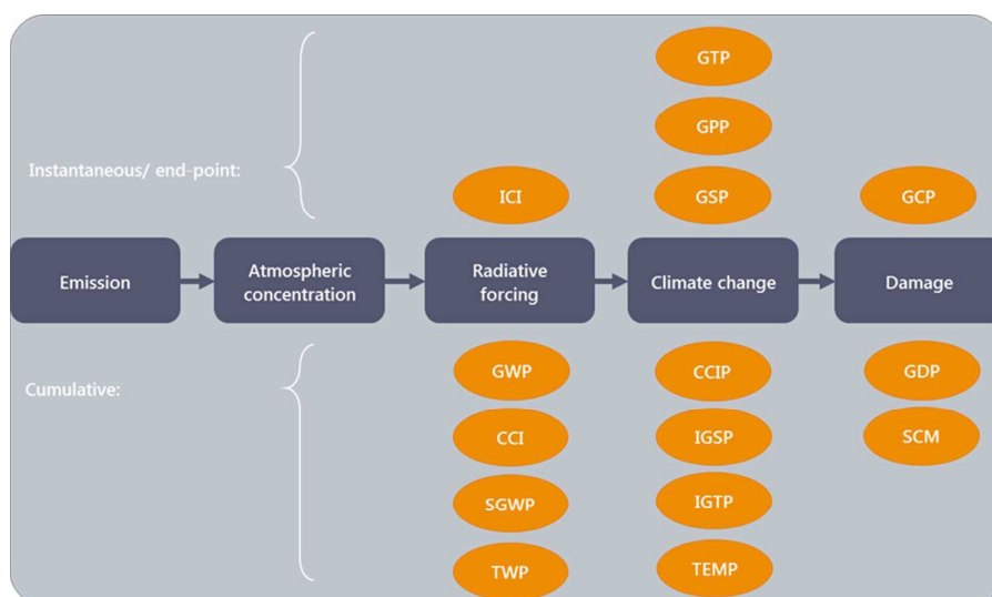
Figure 8. Climate metrics categorised by: stage in cause-effect chain; whether they indicate instantaneous or cumulative impacts.
