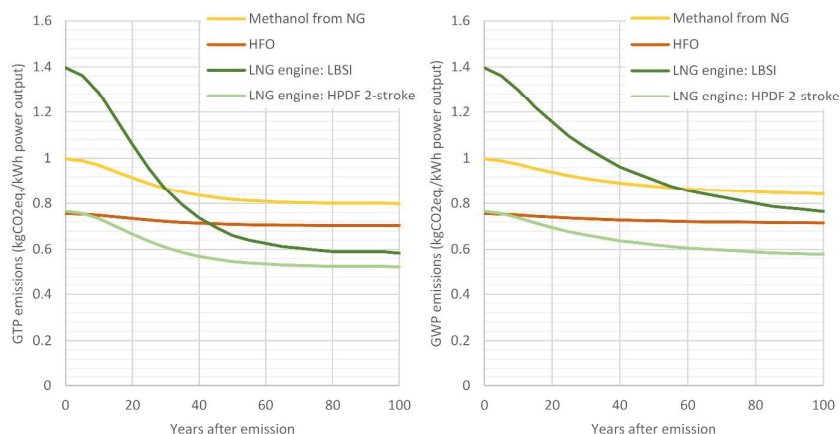
Figure 12. Life cycle GHG emissions associated with a selection of fuels and marine engine types, expressed for each year after emissions using GTP (left) and GWP (right) metrics.
