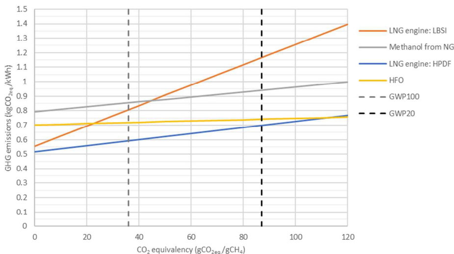
Figure 11. Estimates of total CO 2 equivalent GHG emissions for different shipping fuels and engines
