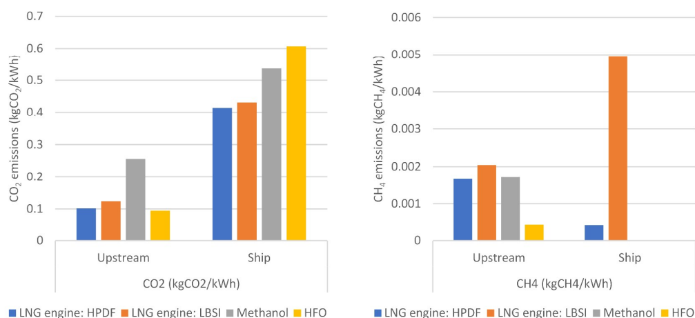
Figure 10. CO 2 and methane emissions associated with the supply and use of 4 different fuels and engines for ships. Emissions are divided into upstream supply chain and ship usage. Source: 3-11 15, 16
