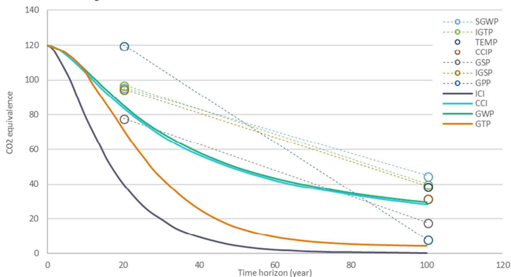
Figure 6. The CO 2 equivalence of methane using different climate metrics, against the time horizon. Dotted lines are placed between paired values of the same metric where only two points are known. Note, for static metrics the x axis denotes the time since the emission and for dynamic metrics CCI and ICI, the x axis represents the time away from the end-point stabilisation year (e.g. 40 years on the x axis means this value is associated with a time horizon of 40 years before the stabilisation period).
