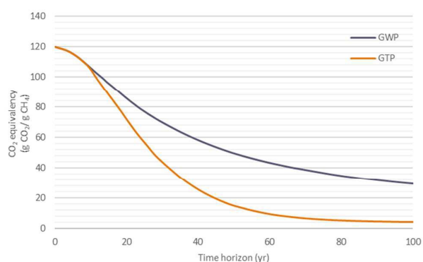
Figure 5. The global temperature change potential of methane compared to the global warming potential, CO 2 equivalencies across different time horizons. Note, indirect carbon climate feedback and methane oxidation effects are not included within these estimates. Source: 44
