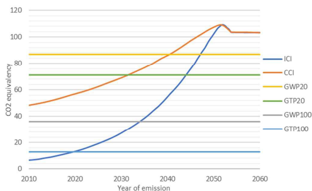
Figure 9. Comparing GWP, GTP, ICI and CCI metric values over time. ICI and CCI values are dynamic and are set to an end-point of 2059, as per Edwards and Trancik 13 , giving an equivalent initial time horizon of 49 years.
