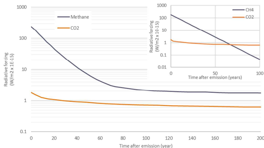
Figure 3. Radiative forcing of a 1 kg pulse emission of methane and carbon dioxide over time, including the eventual oxidation of methane into \text{CO}_2 . Graph inset is the radiative forcing of methane without the inclusion of methane oxidation into \text{CO}_2 . Source: 12, 13
