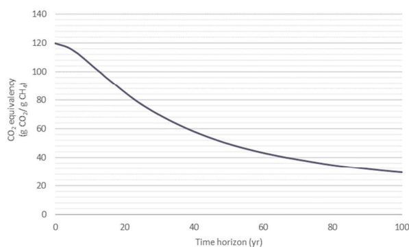
Figure 4: Illustration of the changing GWP of methane over time. Sources: 1, 2 , using GWP factors without climate-carbon feedback effects.
