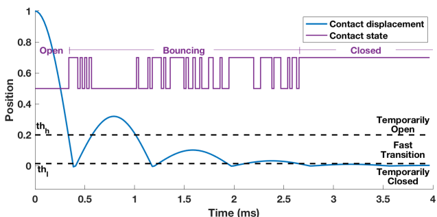
Figure 6: Synthesized contact bounce.
