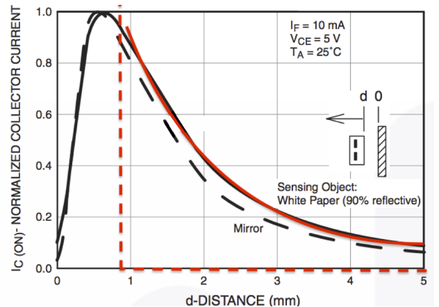
Figure 2: QRE1113: Normalized collector current vs Distance between device and reflector. This image is our overlay (red) on top of an image from the QRE1113 datasheet. The solid red line is the curve described by Eq. (1).
