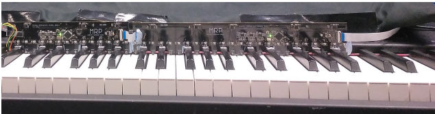
Figure 8: The keyboard scanner installed on the Yamaha CP-300.
