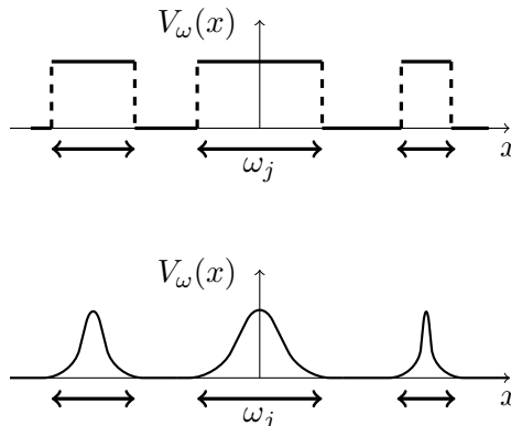
FIGURE 2. Realizations of the standard breather potential and of a general random breather potential
