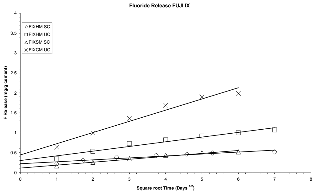
Figure 4.2: Cummulative fluoride release from FUJI IX
