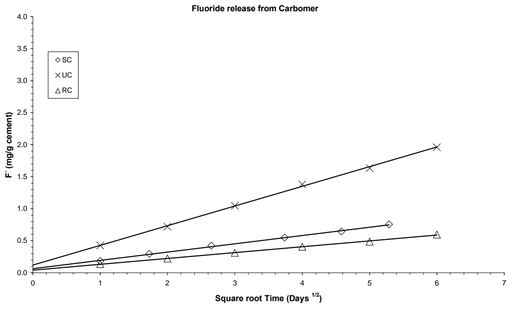
Figure 4.3: Cummulative fluoride release from Glass Carbomer.
