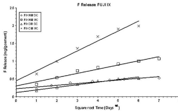
Fig. 4 Fluoride release from capsule and hand mixed Fuji IX
