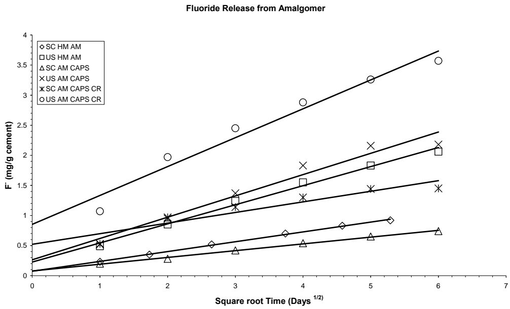
Figure 4.1: Cummulative fluoride release from Amalgomer
