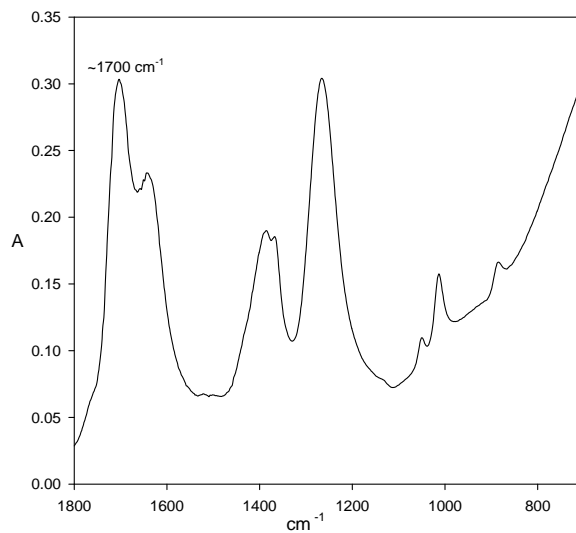
Figure 5.3: ATR-FTIR Spectrum for 45% acetic acid showing C=O peak at ~1700 cm -1
