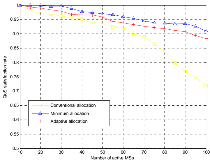
Figure 7.5 Performances of the three algorithms with respect to QoS satisfaction rate
