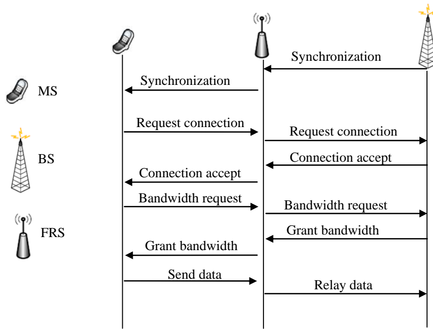
Figure 3.5 The message signalling for the two hop link
