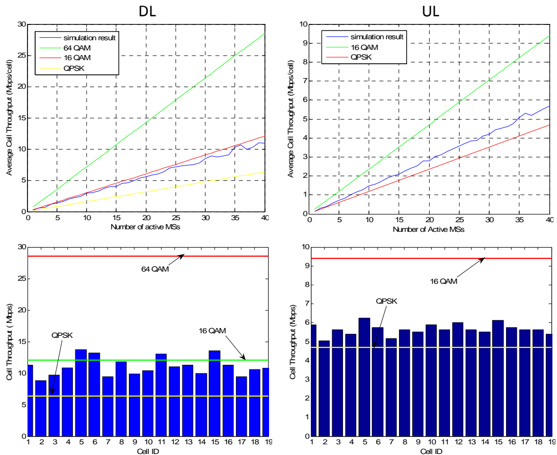
Figure 3.6 Average cell throughputs with different traffic demand
