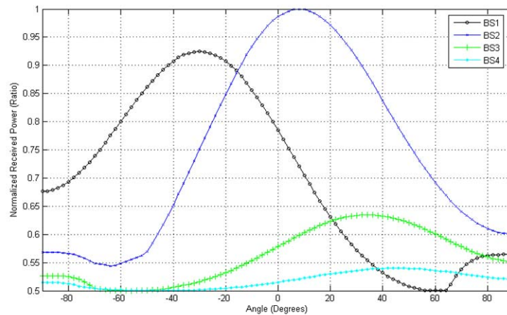
Figure 5.5 The performance of passive DoA : normalized received power from four neighbouring BSs using a 20^\circ beam width.
