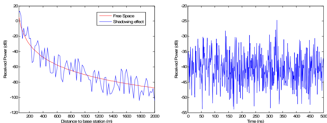
Figure 6.1 The different effects of the propagation components
