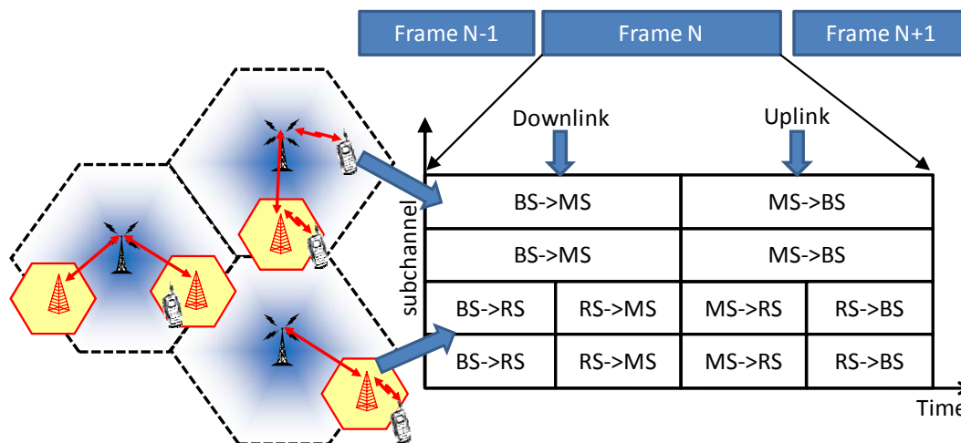
Figure 3.4 The network component topology and channel model of the simulator
