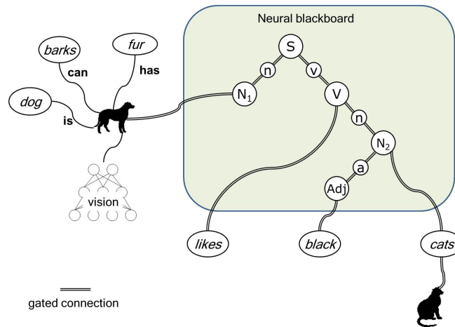
Fig. 6. A neural assembly for dog, embedded in a relation structure based on a neural blackboard architecture.
