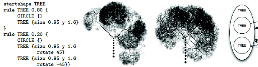
Fig. 8. Examples of non-deterministic grammar, their corresponding tree-like shapes, and their graph representation [Machado et al. 2010]. © Machado et al. Reproduced by permission.
