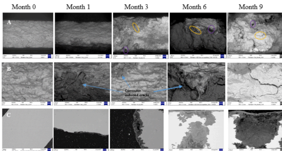
Fig. 7: SEM of AZ31 dumbbell samples showing tensile fracture surface morphology after 0, 1, 3, 6, or 9 (left to right) months immersion in PBS A) low magnification (marker bars = 100 \mu\text{m} ) and B) high magnification (marker bars = 20 \mu\text{m} ). C) polished sample cross sections remote from the tensile fracture site (marker bars = 100 \mu\text{m} ). Regions highlighted with yellow circles and purple ovals indicate regions of magnification and corrosion pits.
