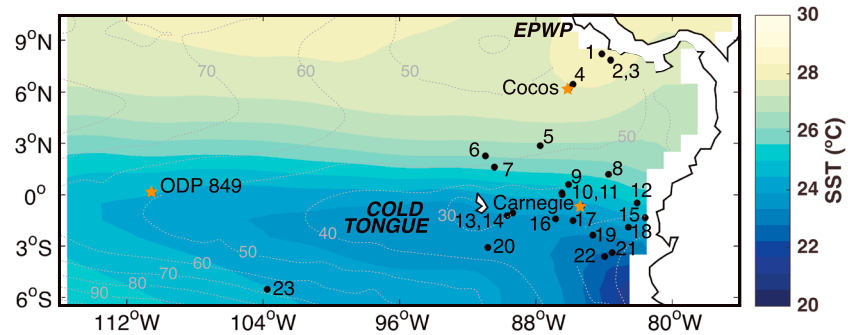
Figure 1. SST map with sites used in this study. Dashed contours are the 20 °C isotherm depth (meters) as a thermocline depth proxy. Stars are locations of new data and numbers are locations of published data (Table 2). ODP = Ocean Drilling Program; EPWP = Eastern Pacific Warm Pool; SST = sea surface temperature.
