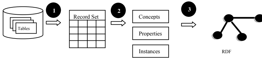
Figure 5. RDBMS to RDF mapping
