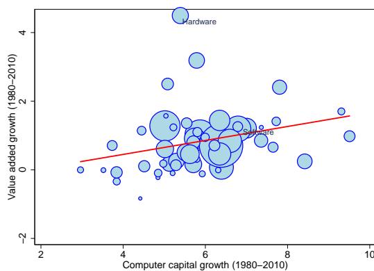
(b) Software
