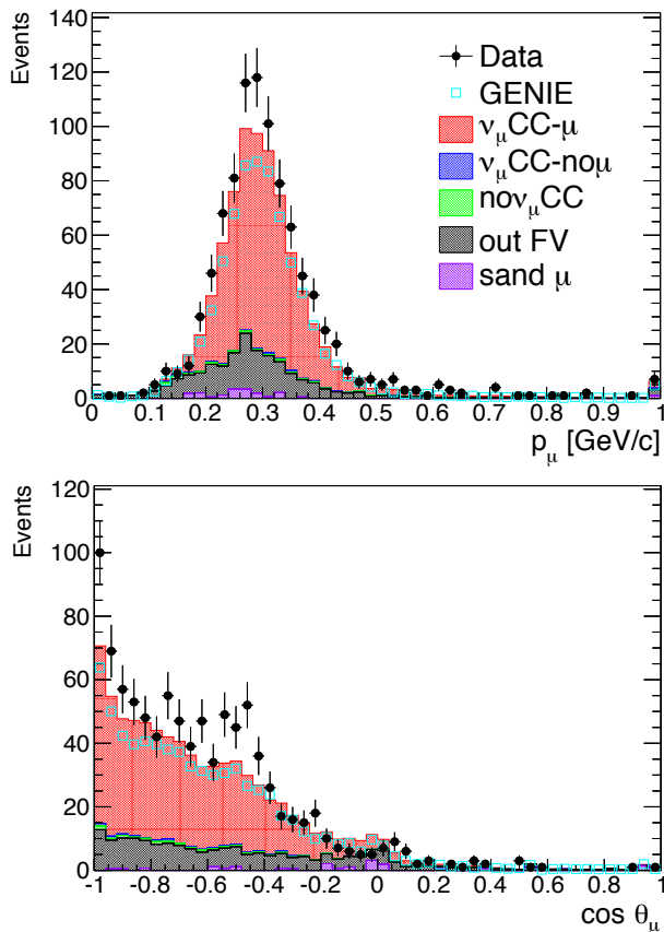
FIG. 5. Momentum (top) and cosine of emission angle (bottom) for the muon candidate when all selection criteria are fulfilled in the BWD selection. Stacked histograms indicate different reaction types predictions from NEUT. Empty rectangles indicate the prediction from GENIE. Data distributions show their statistical error bars.
