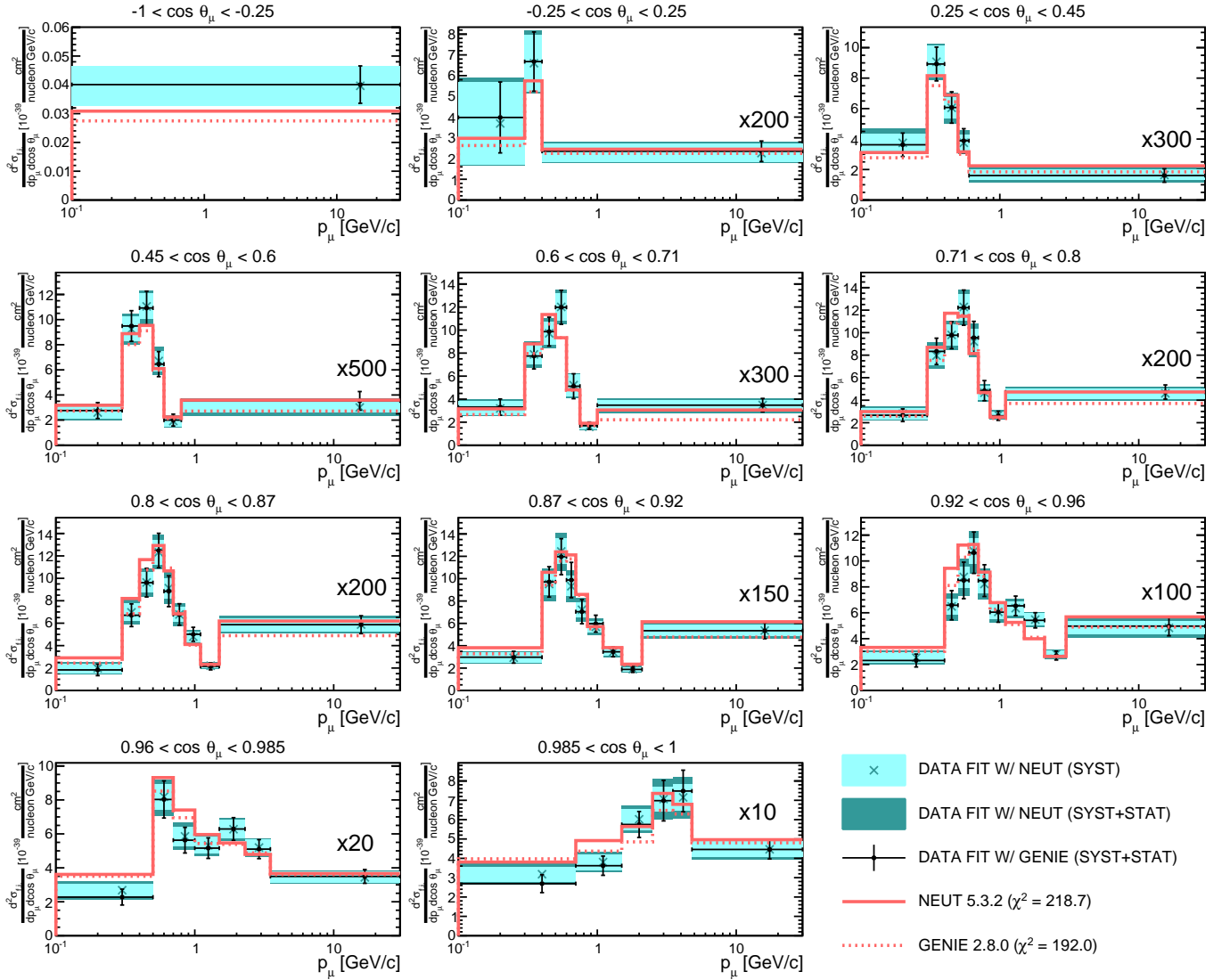
FIG. 13. The flux-integrated, double-differential cross section per nucleon for NEUT (continuous red line), for GENIE (dashed red line), and the unfolded-data result using as prior either NEUT or GENIE. The bin of highest momentum is scaled by the factor shown in each plot to make it visible. \chi^2 values are computed with unfolded-data result using as prior NEUT.
