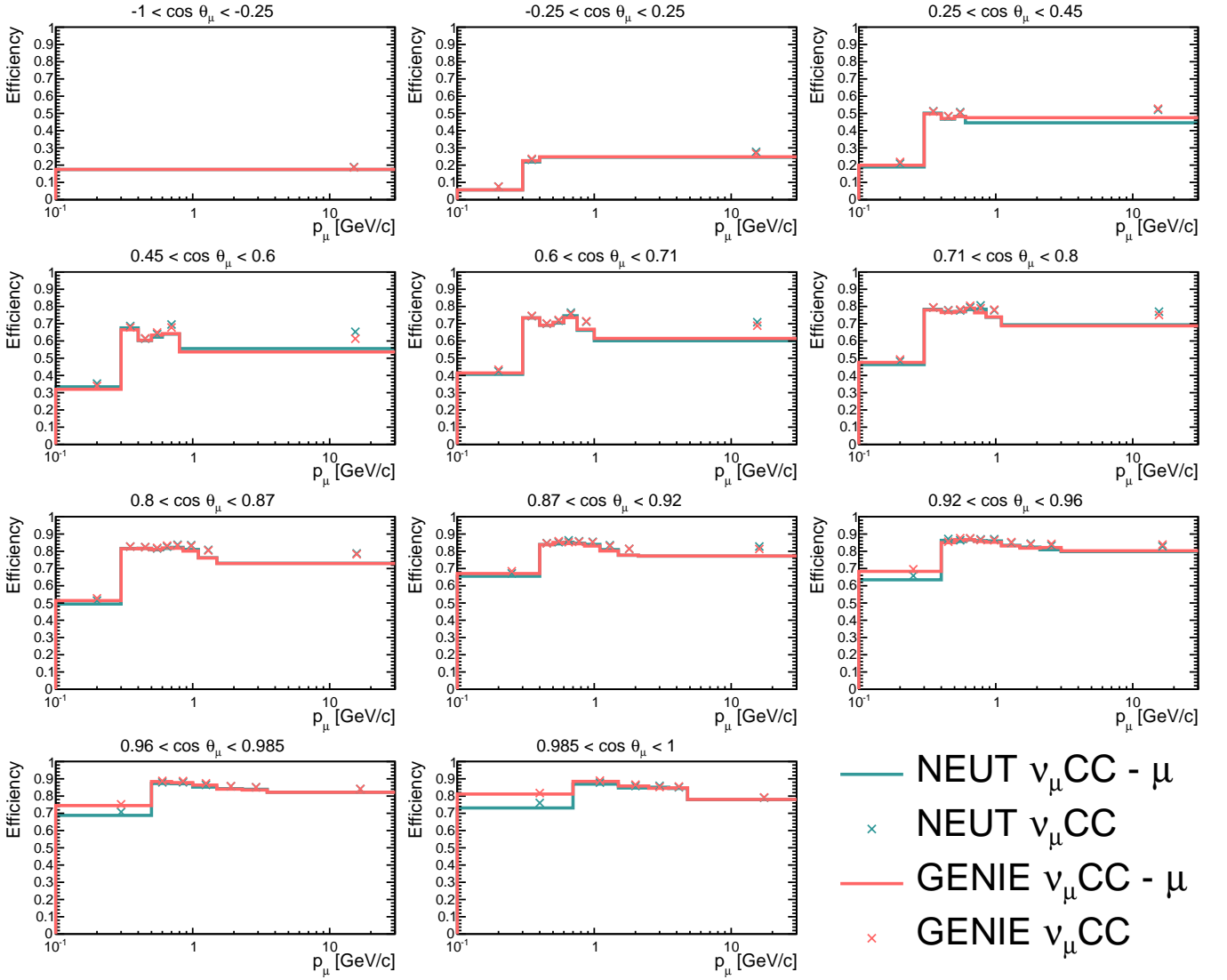
FIG. 11. The reconstructed signal efficiency as function of the momentum and cosine of emission angle of the true muon using the same binning as that for the cross-section result (see Table IV). Lines represent the efficiencies where the signal is defined as \nu_\mu CC events in which the muon candidate is the true muon, so called \nu_\mu CC- \mu events. Markers are efficiencies when the muon candidate requirement is not imposed in the sample labeled as \nu_\mu CC.
