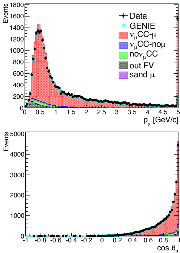
FIG. 4. Momentum (top) and cosine of emission angle (bottom) for the muon candidate when all selection criteria are fulfilled in the FWD selection. Stacked histograms indicate different reaction types predictions from NEUT. Empty rectangles indicate the prediction from GENIE. Data distributions show their statistical error bars.
