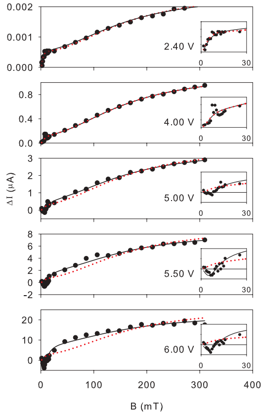
FIG. 4. (Color online) The absolute change in current for a 20-nm Alq 3 OLED as a function of magnetic field for several different drive voltages. The solid line is the fit using the trapping, dissociation and interaction components [see Eq. (1)] and the dotted line is the fit using just the trapping and interaction terms. At low voltages, these two fits overlap perfectly. The inset for each graph is the detail of the low-field region from 0 to 30 mT.
