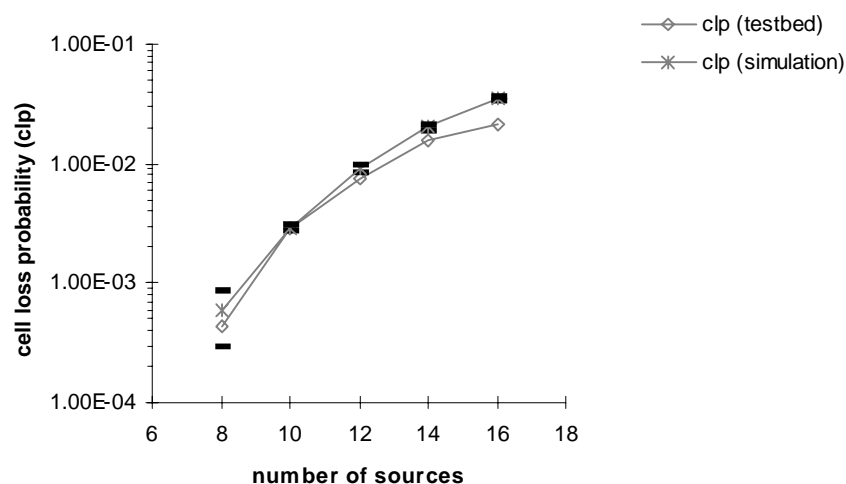
Fig.8.3 - Simulation versus ATM testbed: varying the number of sources multiplexed (network load: 32% to 64%).
