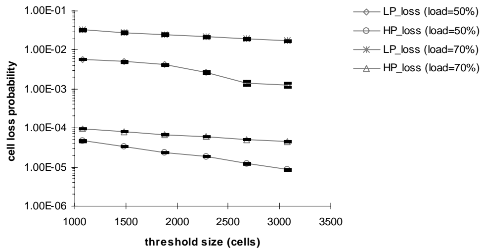
Fig.5.11 - Increase in cell loss probability for a decrease in the threshold.
