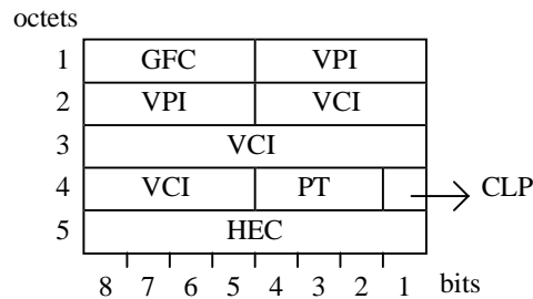
Fig.3.2 - Structure of an ATM cell's header.
