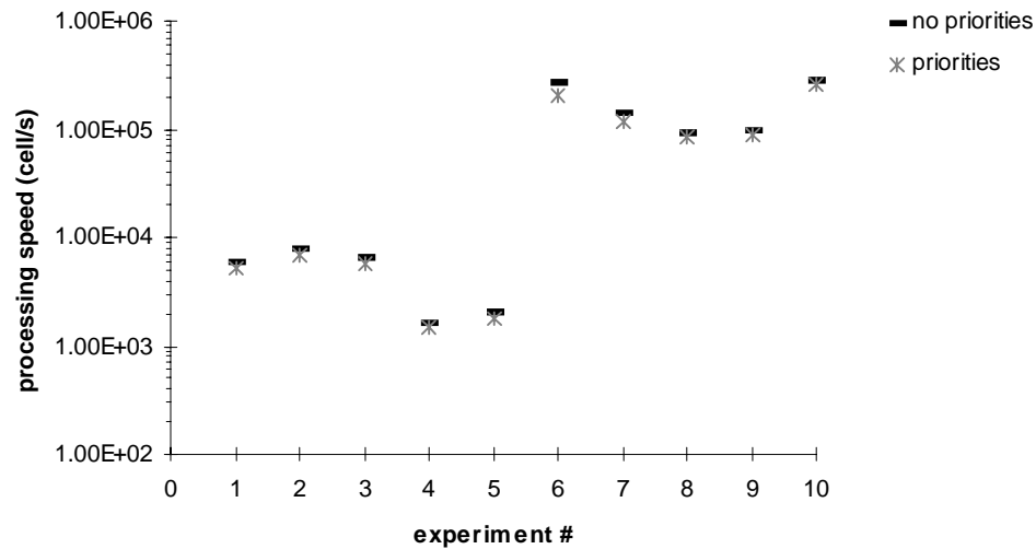
Fig.5.14 - Comparison of processing speed: no priorities versus priorities.
