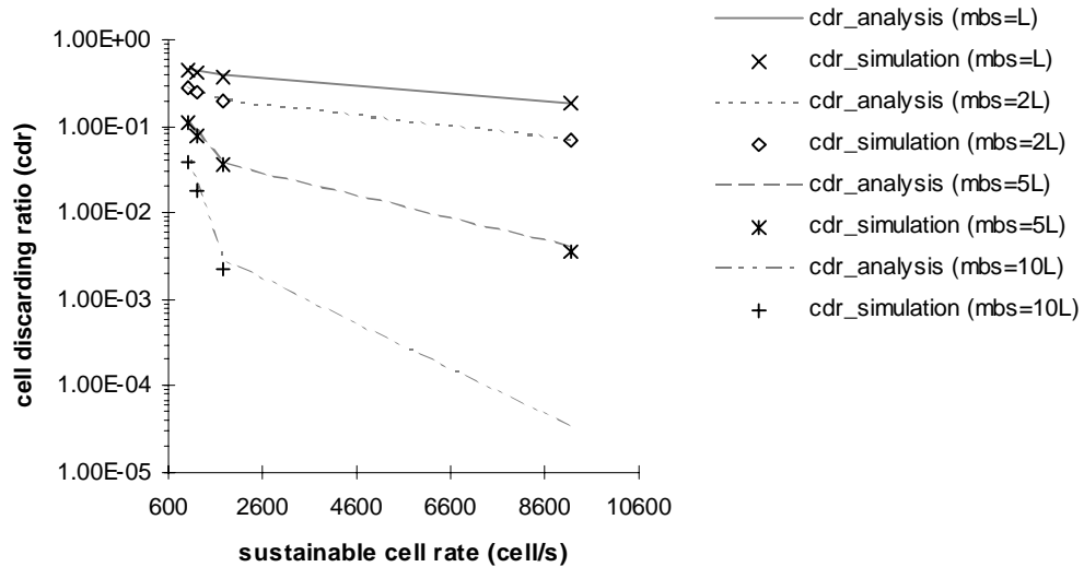
Fig.7.10 - Policed simulation versus fluid flow approximation: traffic with high burstiness ( source type B ). (*) L=abl
