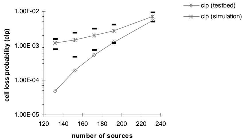
Fig.8.8 - Simulation versus ATM testbed: increasing the number of sources multiplexed (network load: 41% to 66%).
