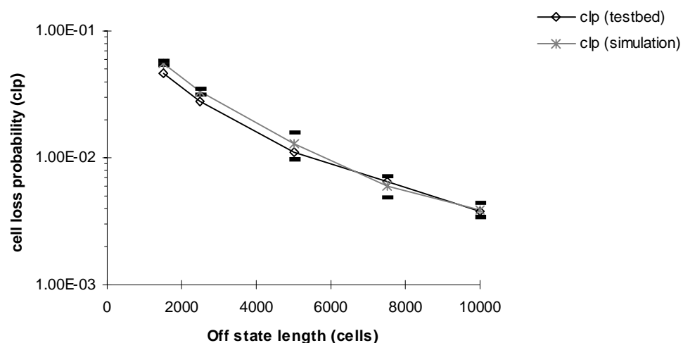
Fig.8.2 - Simulation versus ATM testbed: varying the sources' mean silence duration (network load: 66% down to 12%).
