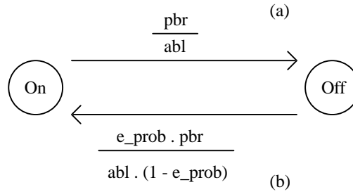
Fig.7.8 - The two-state Markov modulated rate process for the On/Off source;
