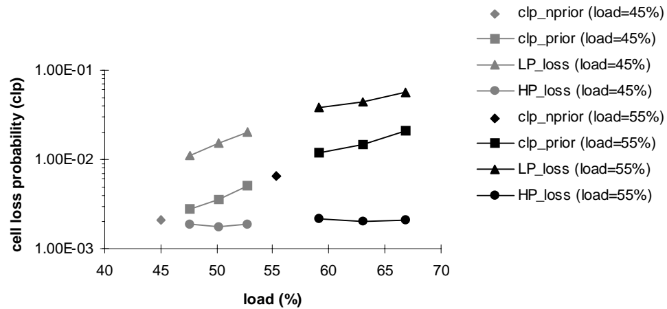
Fig.5.10 - Increase in the admissible network load when using priorities.
