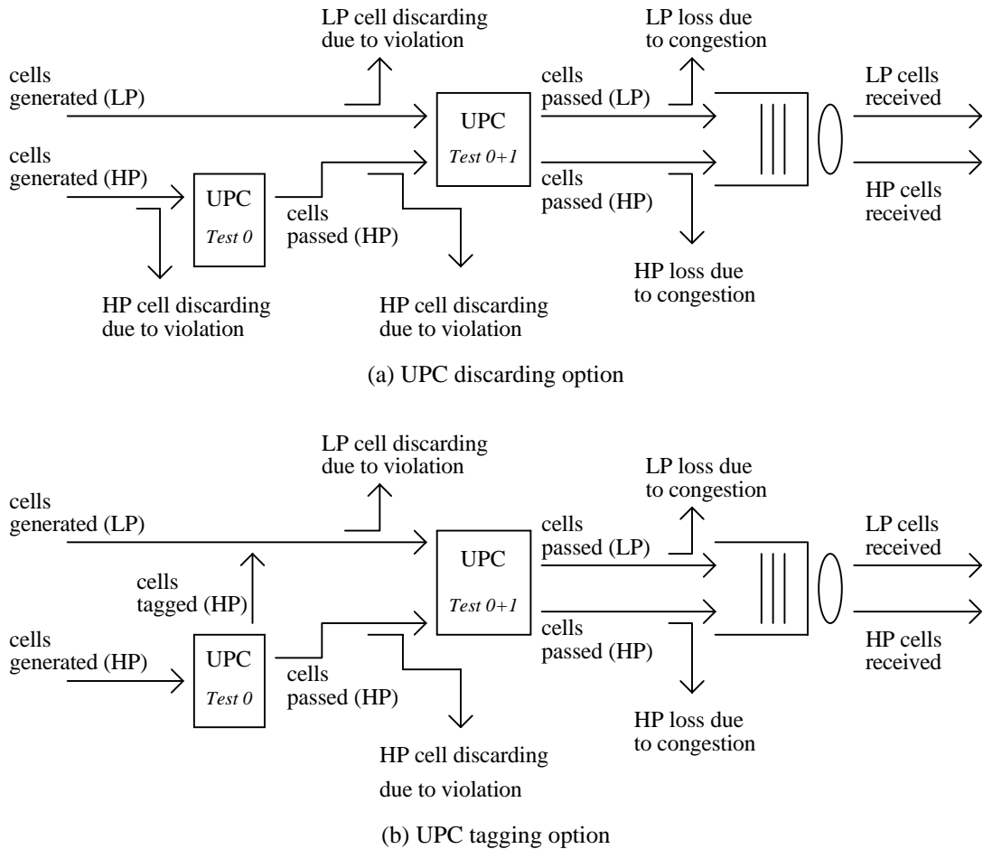
Fig.7.24 - Traffic loss with policing Scenarios 3 and 4 : discarding and tagging of high priority traffic.
