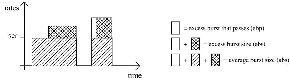
Fig.7.12 - Identification of traffic parameters for policing experiments (traffic without priorities).
