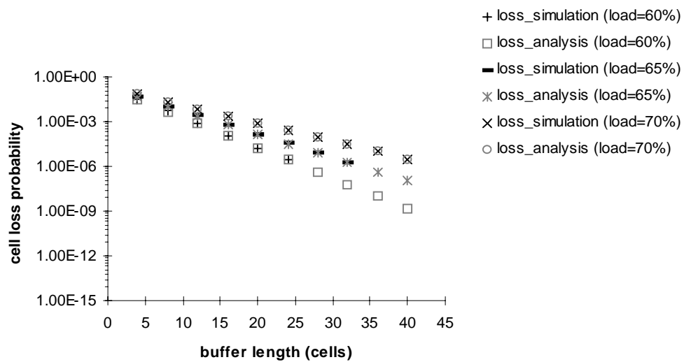
Fig.6.5 - Simulation versus approximate analysis, for traffic without priorities: increasing the network load by increasing the On source time (from Table 6.2).
