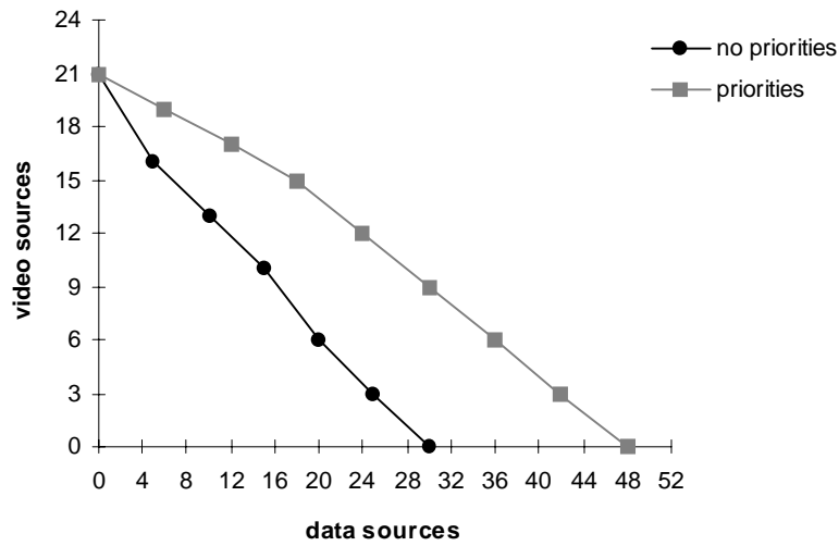
Fig.5.5 - Combinations of traffic sources (from [Krön91]).
