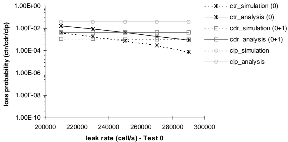
Fig.7.23 - Policed cell-rate simulator with tagging at policing Test 0 versus approximate analysis: high burstiness sources ( Scenario 4 ).
