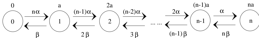
Fig.4.5 - The multi-minisource model.
