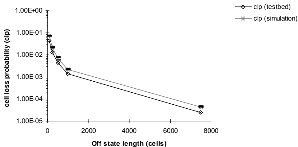
Fig.8.1 - Simulation versus ATM testbed: varying the sources' mean silence duration (network load: 80% down to 2%).
