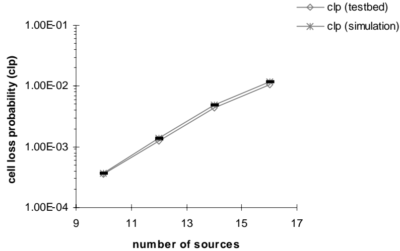
Fig.8.5 - Simulation versus ATM testbed: 3 state GMDP traffic sources (network load: 42% to 67%).
