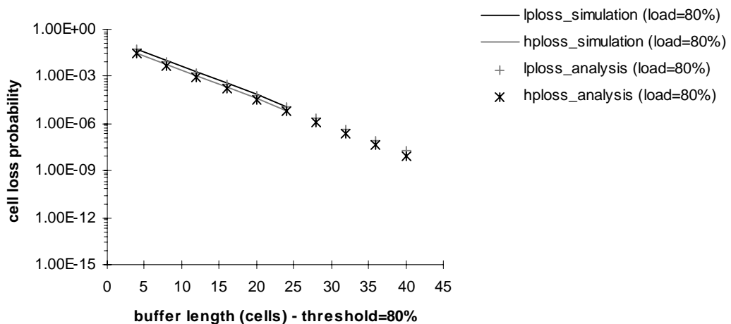
Fig.6.6 - Simulation versus approximate analysis, for traffic with priorities: increasing the queue's length (from Table 6.3).
