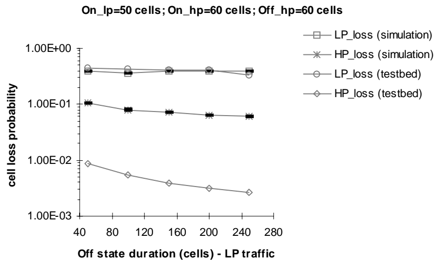
Fig.8.12 - Prioritised simulation versus ATM testbed: varying the Off state duration of the low priority traffic.
