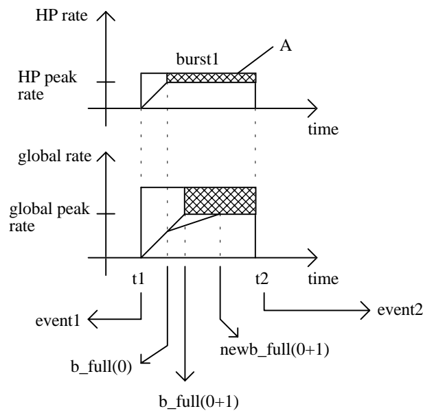
Fig.7.7 - The output of Test 0 and its influence in Test 0+1 .
