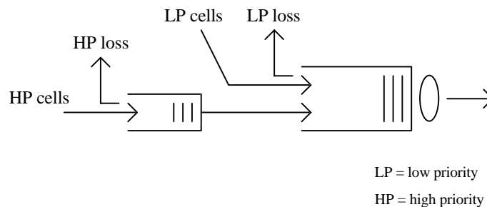
Fig.3.9 - The Partial Buffer Sharing mechanism.
