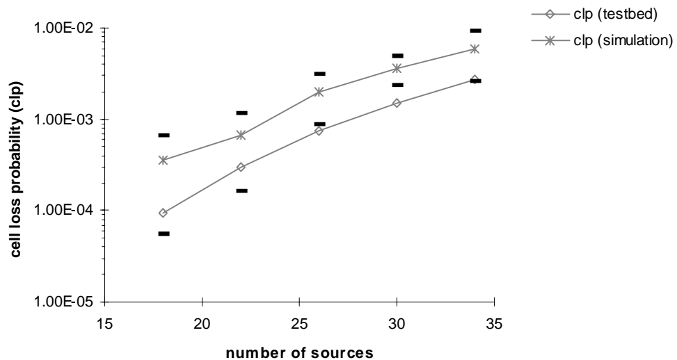
Fig.8.4 - Simulation versus ATM testbed: varying the number of sources multiplexed (network load: 18% to 34%).
