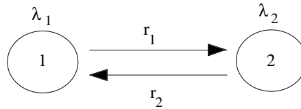
Fig.4.2 - An MMPP model with two states.
