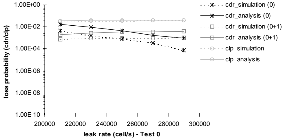
Fig.7.21 - Policed cell-rate simulator with discarding at policing Test 0 versus approximate analysis: high burstiness sources ( Scenario 3 ).
