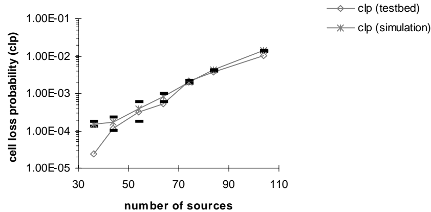
Fig.8.9 - Simulation versus ATM testbed: increasing the number of sources multiplexed (network load: 36% to 78%).
