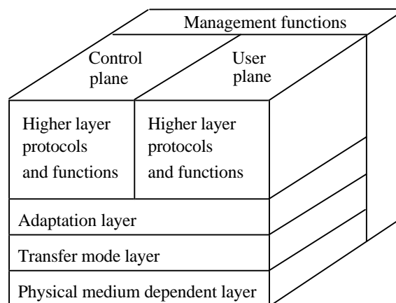
Fig.2.1 - The protocol reference model for B-ISDN.
