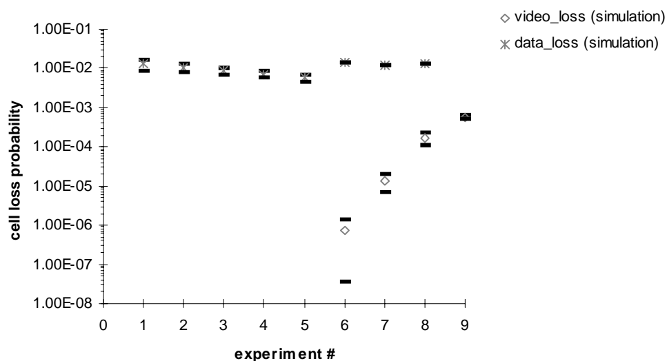
Fig.5.7 - Simulation results using LINKSIM with the PBS mechanism.
