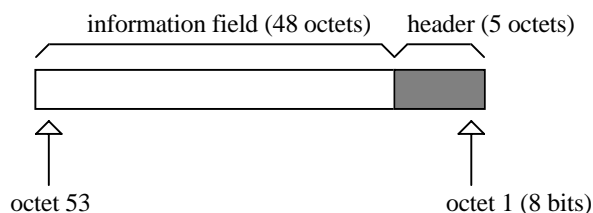
Fig.3.1 - Format of an ATM cell.
