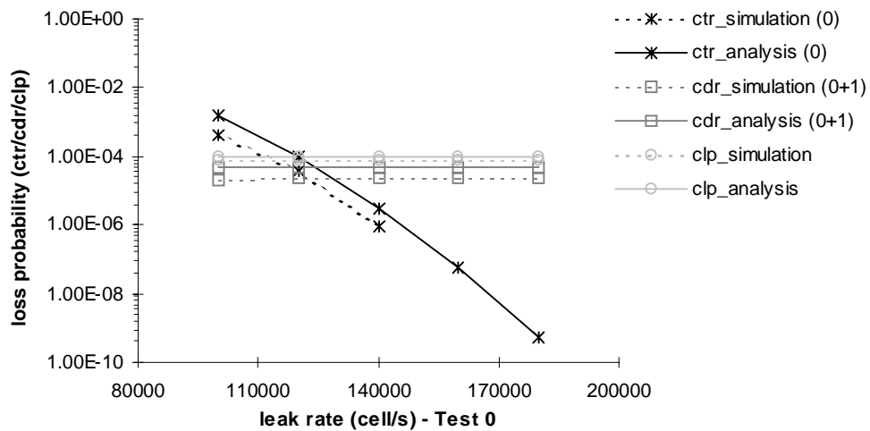
Fig.7.22 - Policed cell-rate simulator with tagging at policing Test 0 versus approximate analysis: low burstiness sources ( Scenario 4 ).
