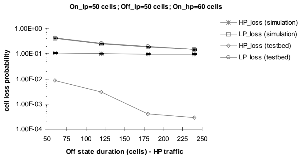
Fig.8.11 - Prioritised simulation versus ATM testbed: varying the Off state duration of the high priority traffic.
