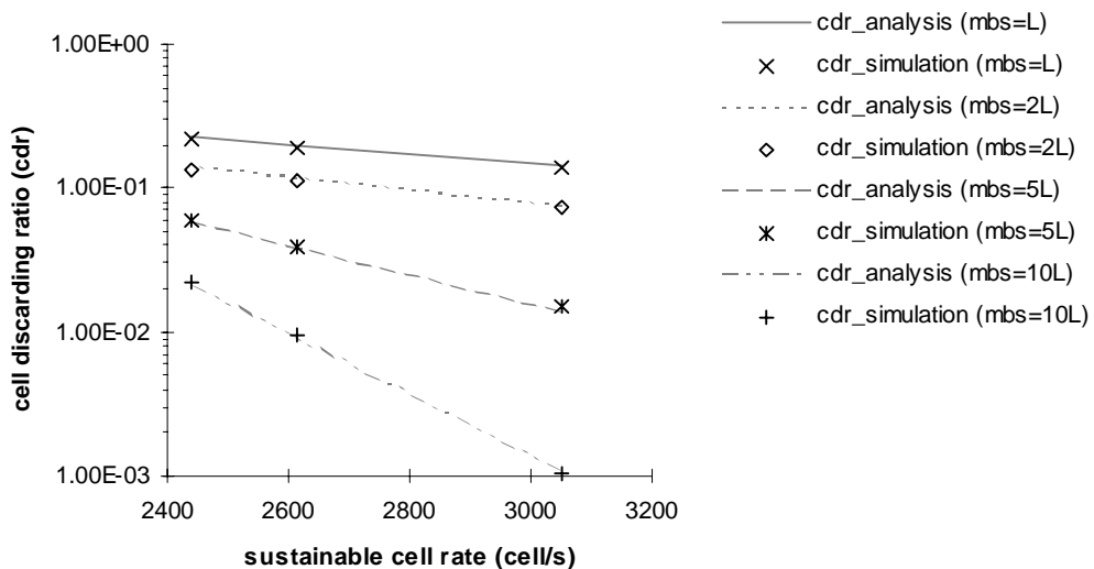
Fig.7.11 - Policed simulation versus fluid flow approximation: traffic with low peak cell rate and low burstiness ( source type C ). (*) L=abl
