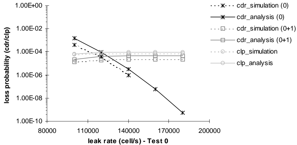
Fig.7.20 - Policed cell-rate simulator with discarding at policing Test 0 versus approximate analysis: low burstiness sources ( Scenario 3 ).
