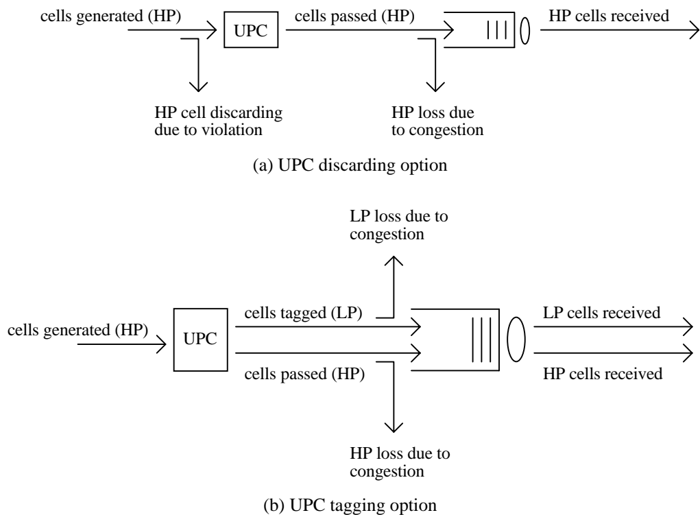
Fig.7.15 - Traffic loss with policing Scenarios 1 and 2 : discarding and tagging of traffic without priorities.
