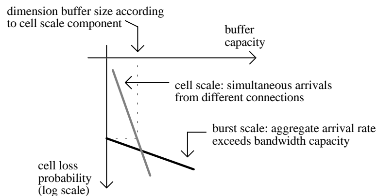
Fig.5.4 - Burst and cell scale components of queuing behaviour.
