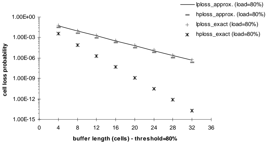
Fig.6.11 - Approximate analysis versus exact analysis, for traffic with priorities: increasing the queue's length (from Table 6.3).
