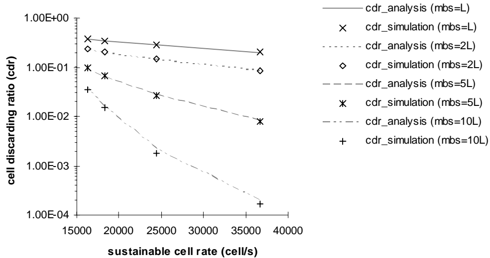
Fig.7.9 - Policed simulation versus fluid flow approximation: traffic with high peak cell rate ( source type A ). (*) L=abl
