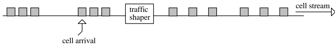
Fig.3.7 - Diagram of traffic shaping.
