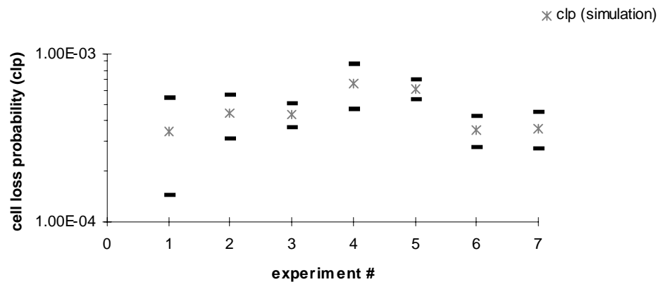
Fig.5.6 - Simulation results using LINKSIM for traffic without priorities.
