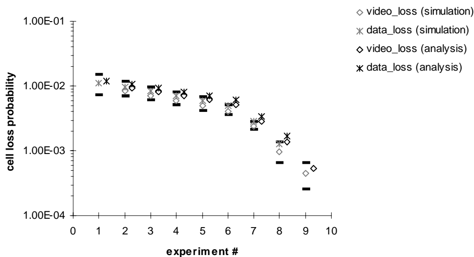
Fig.5.8 - Cell loss upper bound for traffic without priorities.
