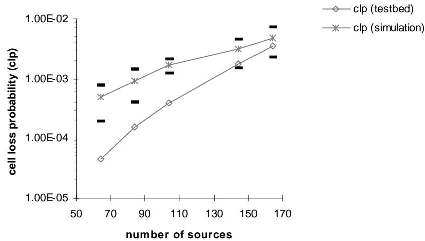
Fig.8.7 - Simulation versus ATM testbed: increasing the number of sources multiplexed (network load: 31% to 56%).
