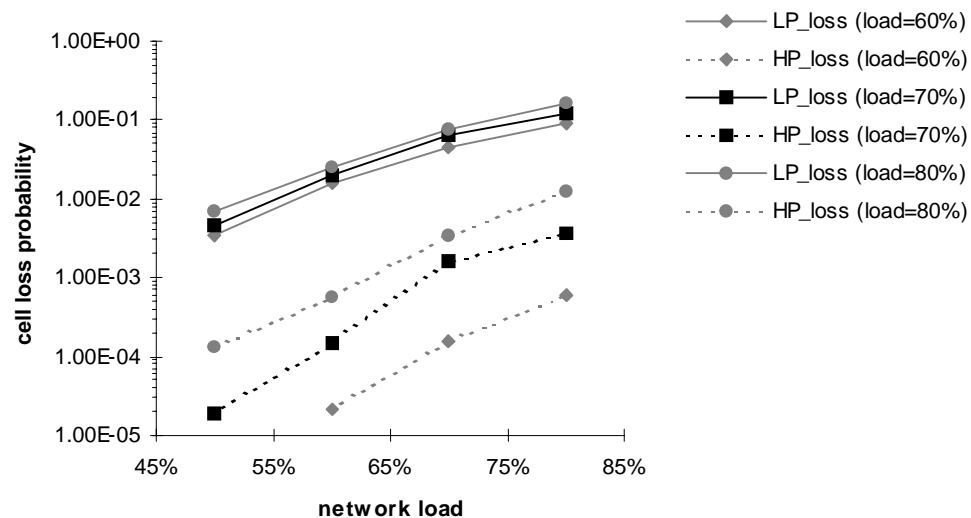
Fig.5.13 - Increasing the network load for a given high priority traffic percentage.
