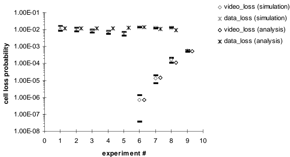
Fig.5.9 - Cell loss upper bound for traffic with priorities.
