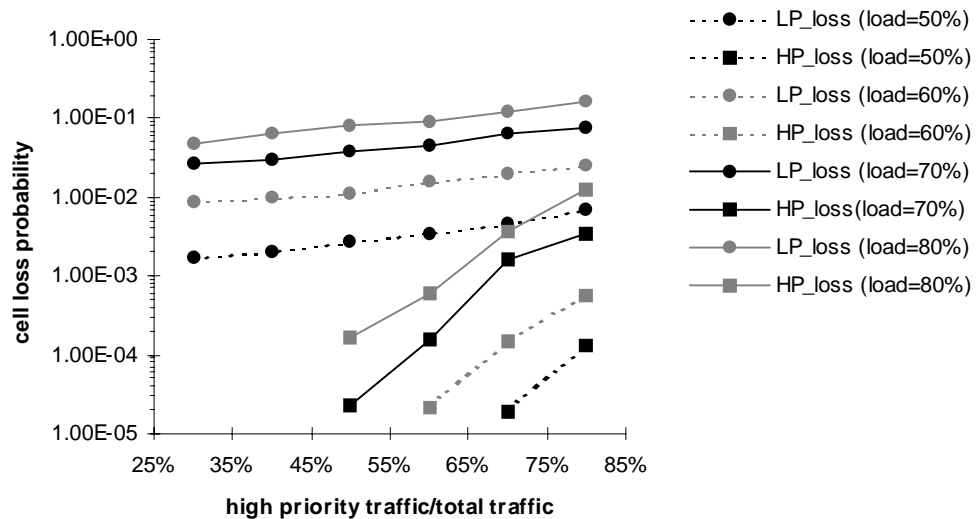
Fig.5.12 - Performance of PBS for an increasing proportion of high priority traffic.
