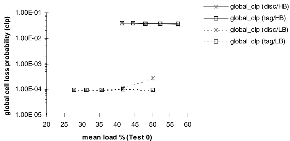
Fig.7.25 - Discarding versus tagging (for traffic with priorities): global cell loss probability for low and high burstiness sources.
