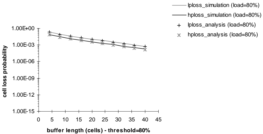
Fig.6.8 - Simulation versus approximate analysis, for traffic with priorities: increasing the input rate for a 80% network load (from Table 6.4).
