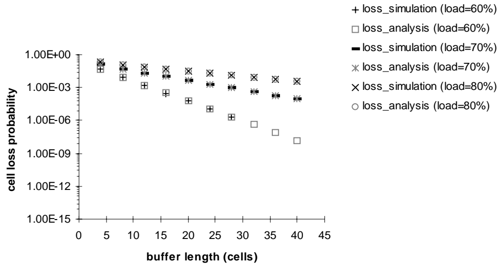
Fig.6.4 - Simulation versus approximate analysis, for traffic without priorities: increasing the network load by increasing the input rate (from Table 6.1).
