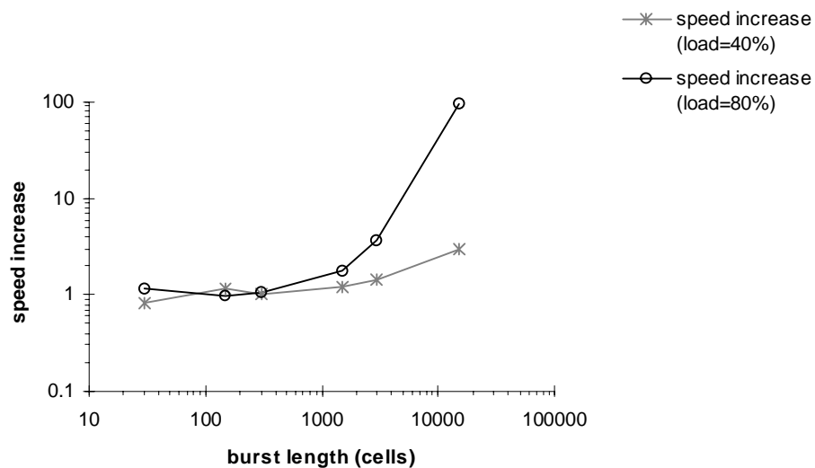
Fig.5.15 - Speed increase of original cell-rate simulator versus source's mean burst length.
