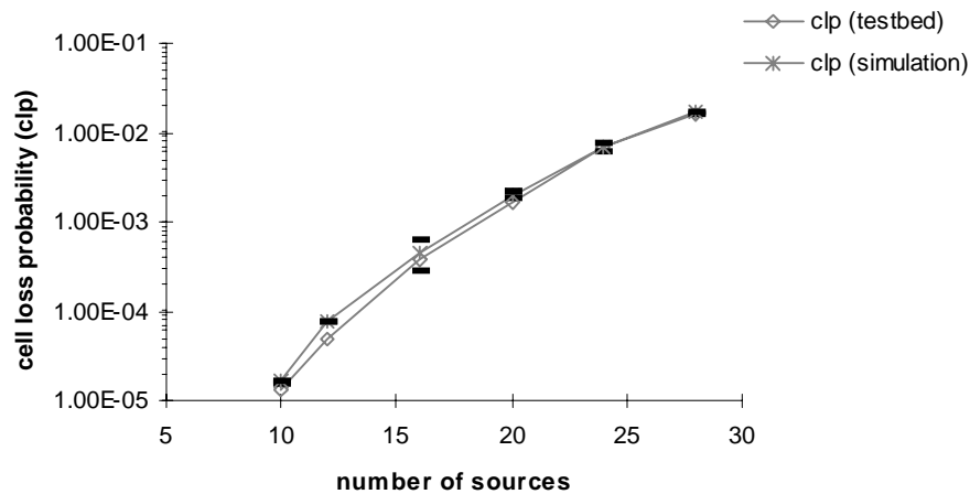
Fig.8.6 - Simulation versus ATM testbed: increasing the number of sources multiplexed (network load: 31% to 76%).
