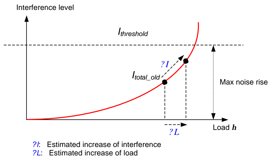
Figure 2.15 Load curve
