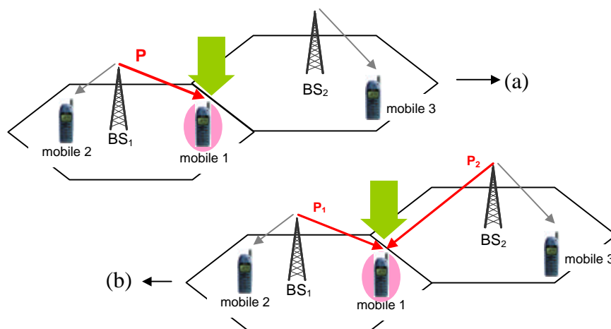
Figure 4.8 Soft handover effects on the downlink interference
