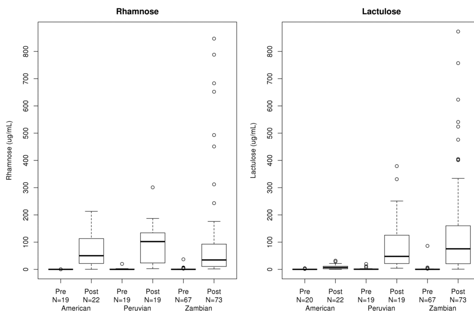
Figure 1 Box plot comparison of pre-dose and post-dose concentrations for rhamnose and lactulose for the three study cohorts.
