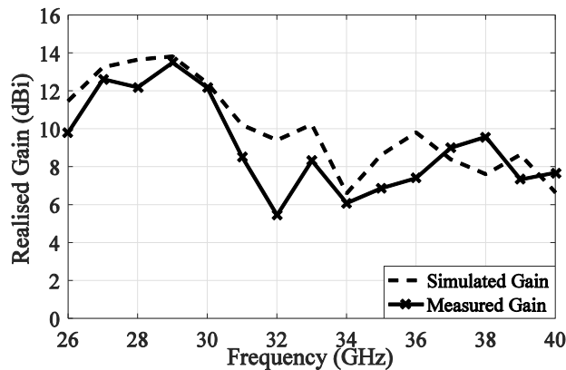
Fig. 7. Simulated and measured realized gain of the MMW 2D antenna array.
