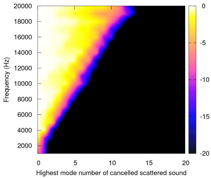
Figure 11: The variation of the damped scattered energy with the highest mode of sound cancellation for the air-filled shell in (a) free space and (b) near the hard ground of Fig 8a.
