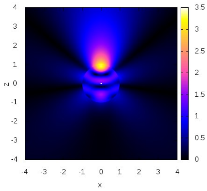
Figure 3: Scattered near-field pressure-amplitude contours that are plotted for the spherical shell when it is placed in free space of water subject to an incoming wave of 6000 Hz propagating at the z direction. The sphere is (a) filled with air and (b) filled with oil (octane). No sound forcing is applied at the shell's centre for cancellation of the scattering.
