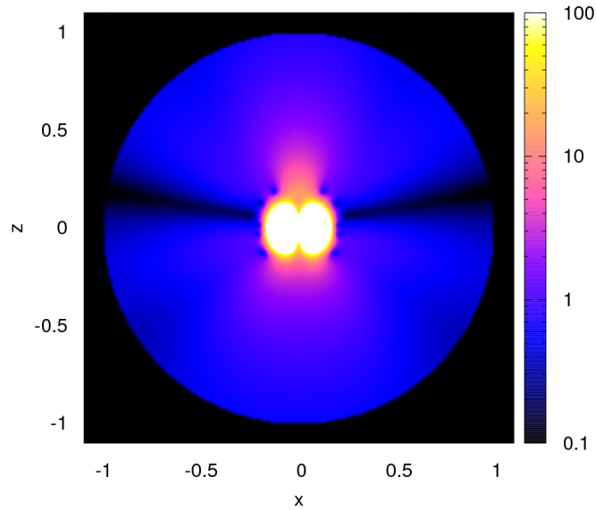
Figure 9: Pressure-amplitude contours that are due just to the forcing multi--poles acting at the centre of the spherical shell to cancel the external scattered sound field shown in Fig 8a.
