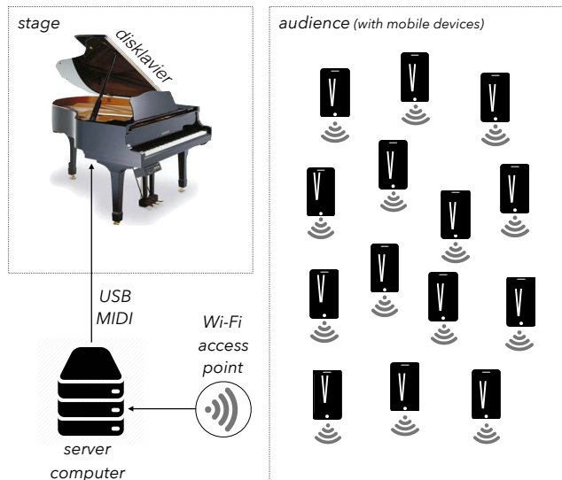
Figure 2: The technical setup of the performance consisting of the players’ mobile devices connected through a local Wi-Fi network to the server that controls the Disklavier automatized piano via a USB MIDI connection.
