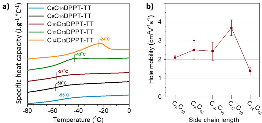
Figure 2. (a) DSC traces of C x C 10 DPPT-TT polymers during the second heating cycle (end up) recorded at a heating rate of 10°C.min -1 . (b) Hole mobilities (averaged over 10 devices) of the different C x C 10 DPPT-TT polymers measured in bottom-gate, top-contact OFET devices plotted against the alkyl side chain length.
