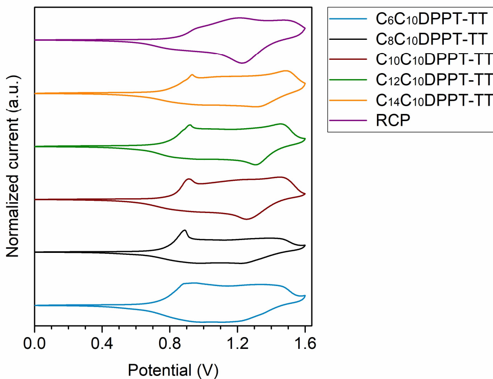
Figure S1. Cyclic voltammograms of \text{C}_x\text{C}_{10}\text{DPPT-TT} polymers and RCP , dropcast ( 5 \text{ mg.mL}^{-1} ) from chlorobenzene solutions onto glassy carbon electrodes.
