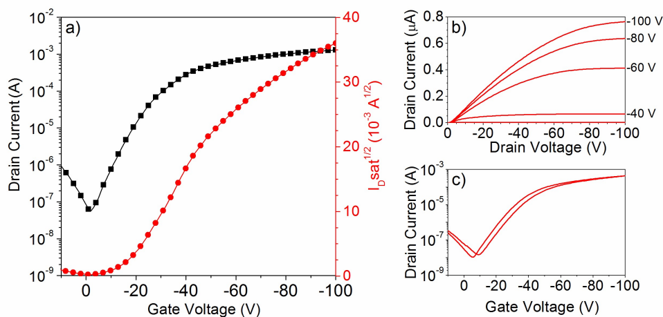
Figure 3. (a) Transfer curve, (b) output characteristics and (c) hysteresis of a BGTC OFET device using the C 12 C 10 DPPT-TT polymer as active material after thermal annealing at 200°C during 1 hour.
