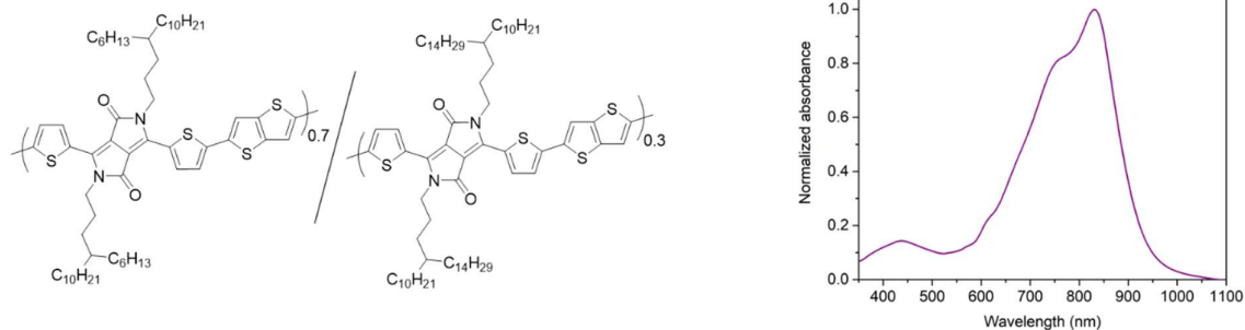
Scheme S2. Chemical structure of the random copolymer RCP and the UV-vis. absorption spectrum in thin film, spin-coated at a concentration of 5 \text{ mg.mL}^{-1} on glass substrate.
