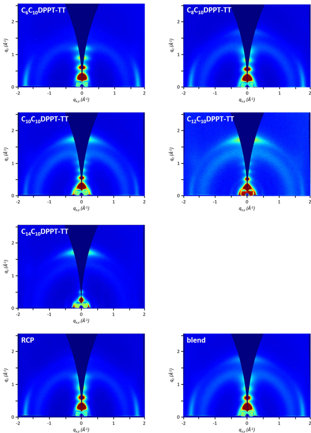
Figure S13. Grazing incidence X-ray diffraction (GIXD) patterns of the different polymers. The polymer films were spin-coated from 10 mg.mL -1 chlorobenzene solutions on Si/SiO 2 substrates. The films have been annealed 200°C for 1 hour under a nitrogen atmosphere, with the exception of RCP and blend, which have been annealed at 150°C for 20 minutes.
