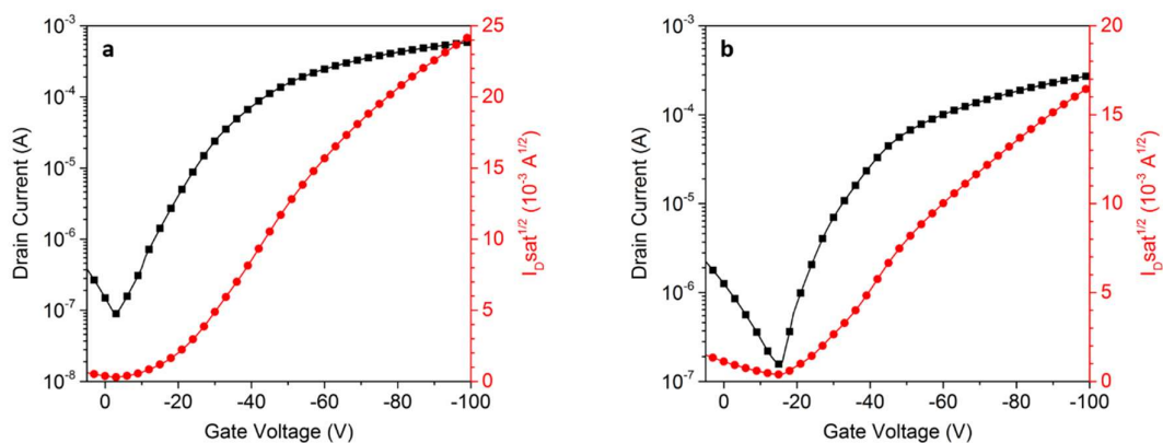
Figure S8. Transfer curves of a BGTC OFET devices of C_6C_{10}DPPT-TT (left) and C_{14}C_{10}DPPT-TT (right) after thermal annealing for 20 minutes at 150^{\circ}C .
