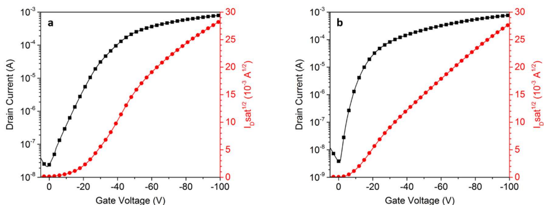
Figure S9. Transfer curves of a BGTC OFET devices of C_6C_{10}DPPT-TT:C_{14}C_{10}DPPT-TT blend (7:3) after thermal annealing for 20 minutes at 150°C (left) and for 1 hour at 200°C (right).
