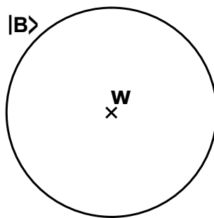
Figure 2.2: Corresponding string Feynman diagram for disk amplitude.
