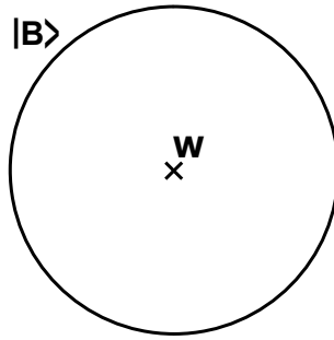
Figure 2.2: Corresponding string Feynman diagram for disk amplitude.
