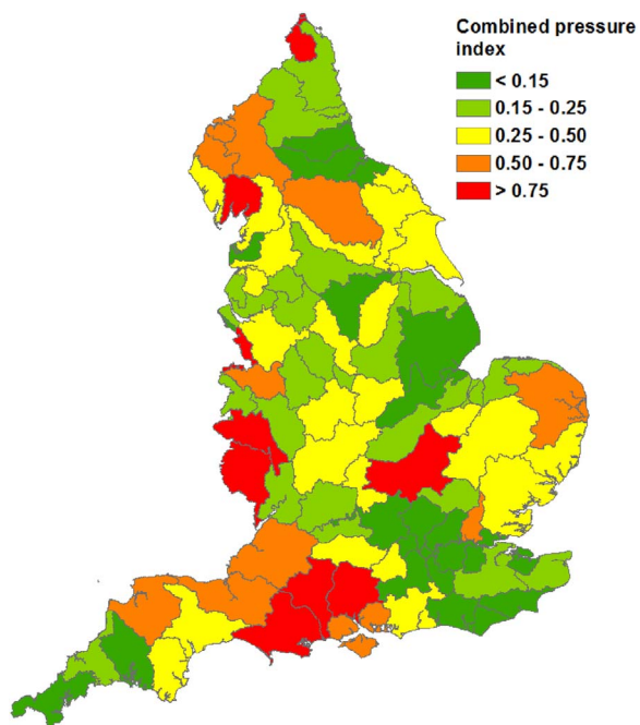
Fig. 5. The spatial distribution of the combined agricultural pollutant pressure index (CPI).
