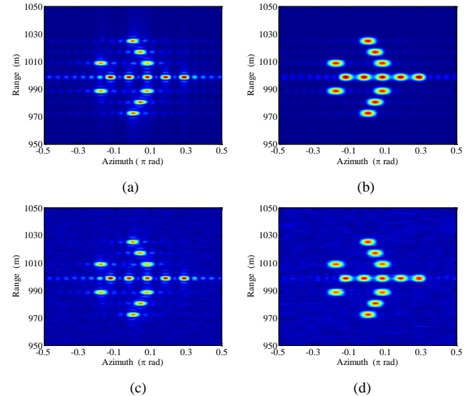
Fig. 4. Imaging results using the concentric-ring array. (a) Imaging results without window or noise contribution, (b) Imaging results with window contribution (no noise), (c) Imaging results with noise contribution (no window), (d) Imaging results with window and noise contributions.
