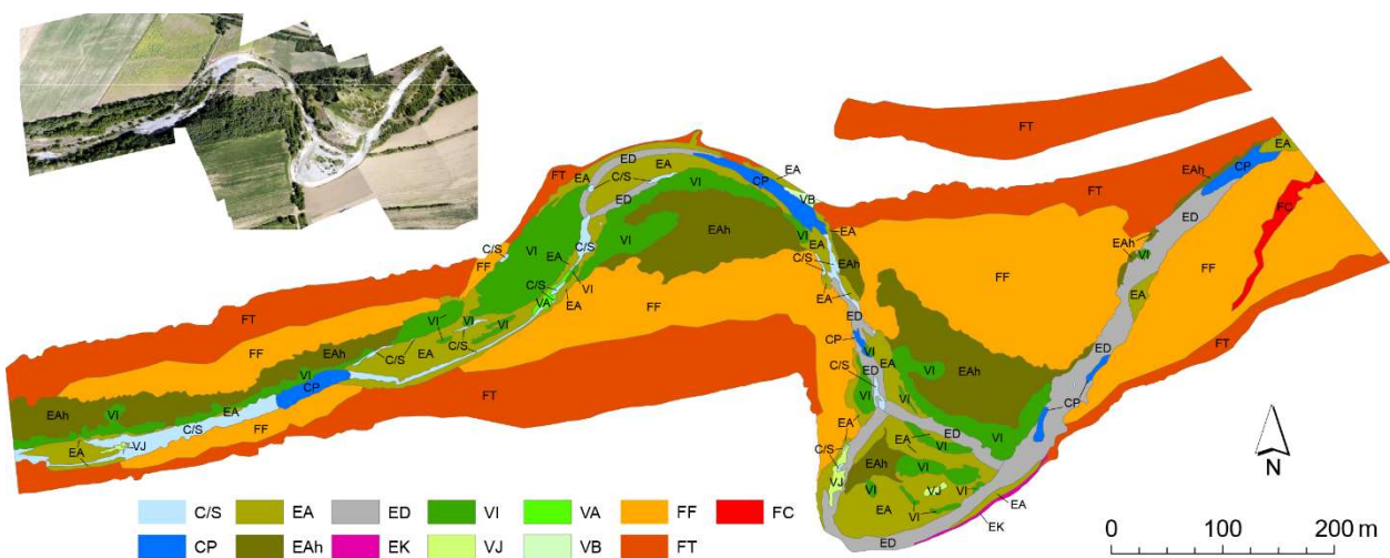
Figure 6. Application of the GUS (basic level) to a sub-reach (sub-reach (ii) in Figure 3) of the Cecina river, showing an aerial image of the sub-reach and a map of the types of geomorphic units present (C/S, base flow / secondary channels; CP, pool. EA, bank-attached bar; EAh, bank-attached high bar; ED, dry channel; EK, unvegetated bank; VI, island; VJ, large wood jam; VA, aquatic vegetation; VB, bench; FF, modern floodplain; FT, recent terrace; FC, secondary channel (within the floodplain)).
