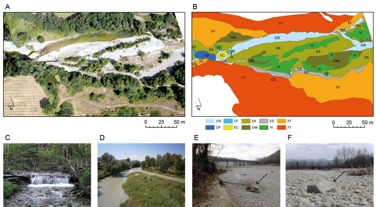
Figure 4. Sub-reach (iii) (see Figure 3 for location) illustrating GUS units and sub-units. (A) Aerial image of the sub-reach. (B) Map of geomorphic units within the sub-reach (see Figure 6 for explanation of the unit codes). (C) A log-step unit. (D) A grassy island unit. (E) A small wood accumulation sub-unit. (F) An isolated boulder sub-unit. (A and B modified from Rinaldi et al., 2016; C and D from Rinaldi et al., 2015b; E and F from Belletti et al., 2015c).
