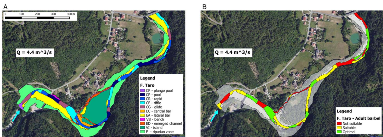
Figure 8. Example of the application of the GUS for the survey and evaluation of mesohabitats for the Taro River (Parma, Italy). (A) Spatial distribution of geomorphic units (bankfull channel and floodplain units). (B) Evaluation of the habitat suitability in terms of bed configuration units for adult barbel ( Barbus sp.). Mesohabitats are classified in three categories: not suitable, suitable and optimal. The flow rate at the time of the survey is also reported. Modified from Rinaldi et al. (2015d).
