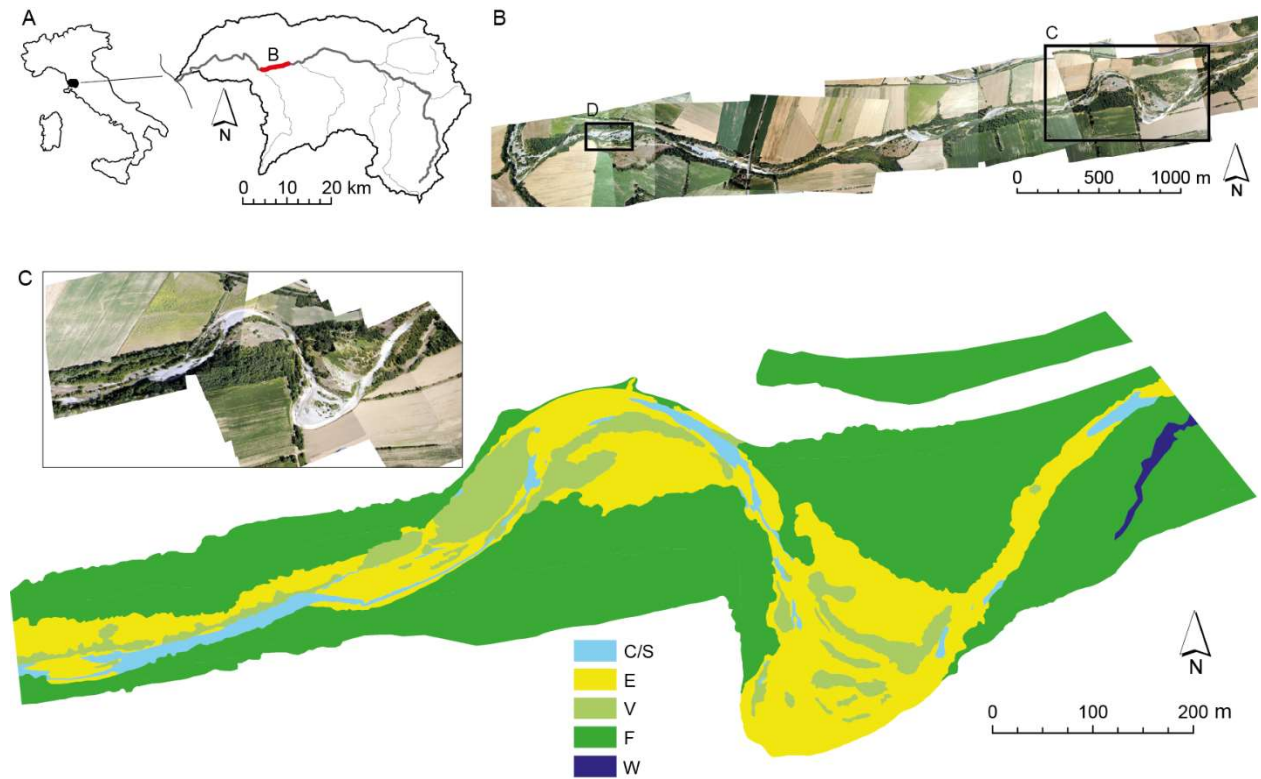
Figure 3. Examples of macro-units for a sub-reach of the Cecina river, Italy. (A) Location of the studied reach (i) displayed in (B) within the Cecina river catchment. (B) Aerial photo of the analysed reach (i) and location of the sub-reach (ii) mapped in C and detailed in Figure 6, and sub-reach (iii) detailed in Figure 4. (C) Map of the macro-units for the sub-reach (ii) at the broad level: C/S, baseflow or submerged channels; E, emergent sediment units; V, in-channel vegetation; F, riparian zone; W, floodplain aquatic zones.
