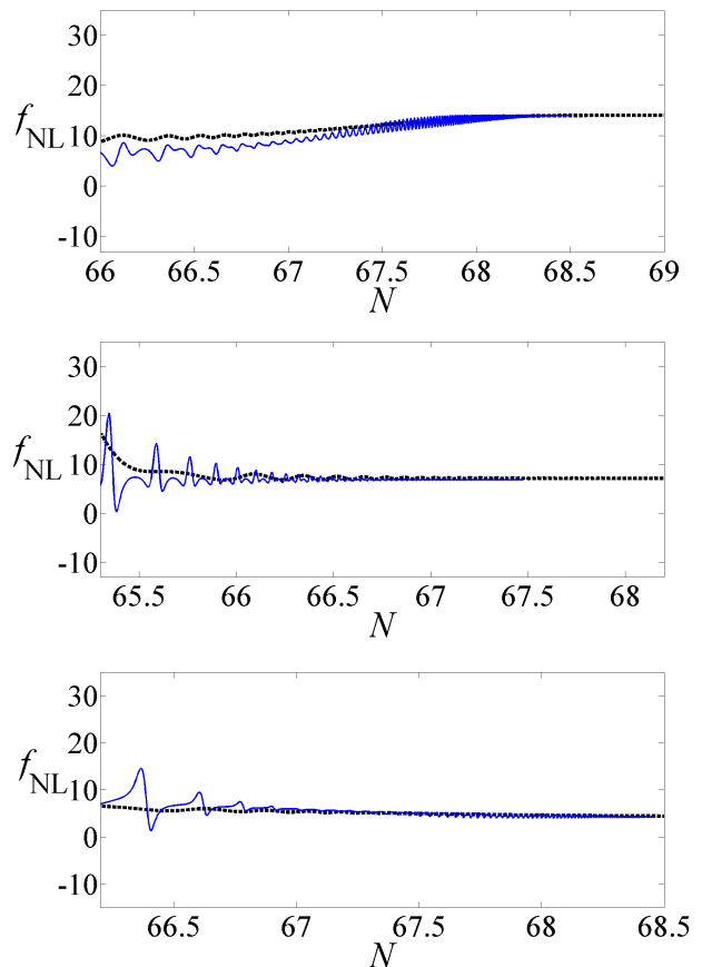
FIG. 4: Plots of f_{\text{NL}} for the axion quadratic model with parameters as given under eq. (53). The solid blue line is the numerical result and the dashed black line is the analytic result. For the top pane we use \mu = 0.6 , and the other two panes use \mu = 0.8 . The values of the \Gamma parameters, in units of m_\phi , are: Top pane: \Gamma_\phi = 0.01 and \Gamma_\sigma = 0.1 , Middle pane: \Gamma_\phi = 0.01 and \Gamma_\sigma = 0.01 , Bottom pane: \Gamma_\phi = 0.1 and \Gamma_\sigma = 0.01 .
