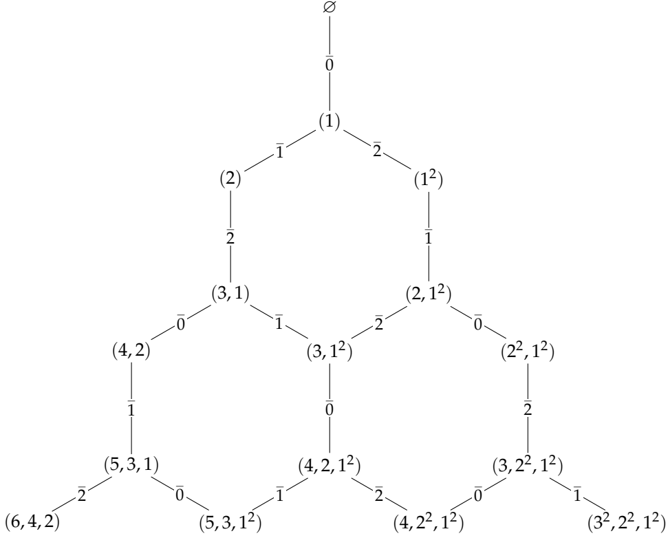
Figure 2: The level 1 action of \tilde{\mathfrak{S}}_3 on \mathcal{C}_3^{(4)}
