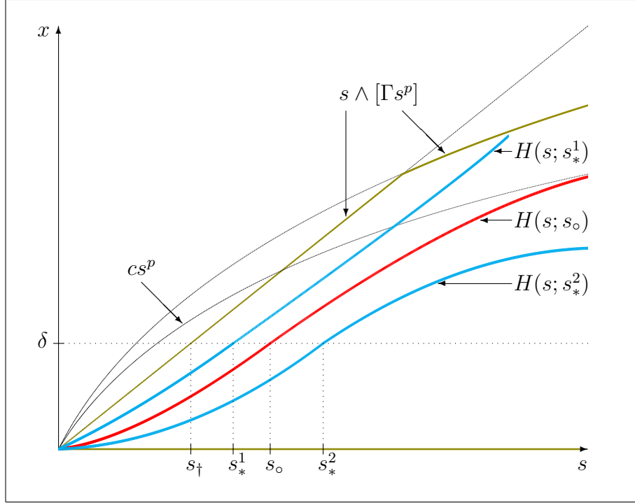
Figure 2 ( p < 1 ) Illustration of Lemma 2.(I) for s_0(\delta) = s^o(\delta) . The free-boundary function H(\cdot) = H(\cdot; s_0) that separates the stopping region \mathcal{S} from the waiting region \mathcal{W} is plotted in red. The intersection of \mathbb{R}^2 with the boundary of the domain \mathcal{D}_H in which we consider solutions to the ODE (23) satisfying (26) is designated by green. Every solution to the ODE (23) satisfying (26) with s_* \in ]s_\dagger, s_0[ (resp., s_* > s_0 ) hits the upper part of the boundary of \mathcal{D}_H in the picture (resp., has asymptotic growth as s \rightarrow \infty that is of different order than the one of the free-boundary): such solutions are plotted in blue.
