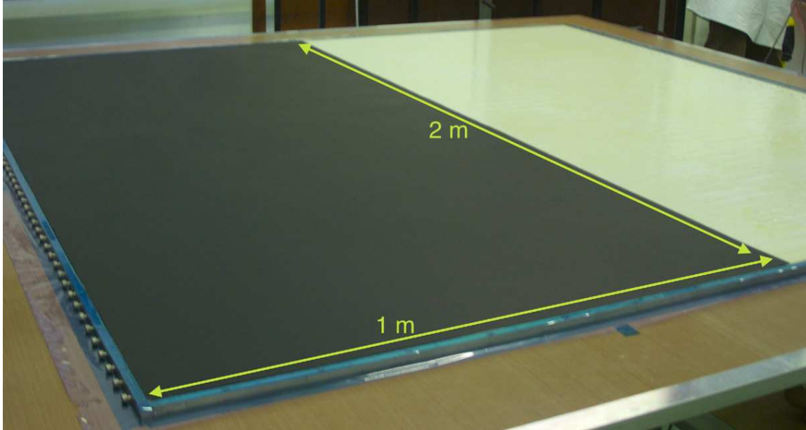
Figure 12. Ds-ECal layer under construction. The first of two sheets of lead is in place on top of the scintillator bars. Visible are the aluminium frame and the locator pins securing the scintillator bars in place for the duration of the layer construction. The frame is covered with blue tape to keep it free from epoxy.
