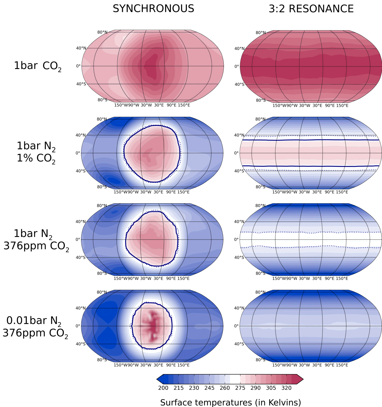
Fig. 6. Biennial mean surface temperatures of atmospheres made of a variety of 4 cocktails of \text{N}_2 and \text{CO}_2 for 2 orbital configurations (synchronous and resonance 3:2), assuming planets initially completely covered by liquid water. Solid lines and dashed lines contours correspond to the location of permanent and seasonal surface liquid water, respectively.
