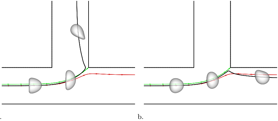
FIGURE 15. Effect of membrane shear elasticity on the capsule trajectory for Re = 20 , q = 0.53 , a/R = 0.4 : (a) Ca = 0.4 , (b) Ca = 0.1 . The streamline legend is the same as in Figure 10.
