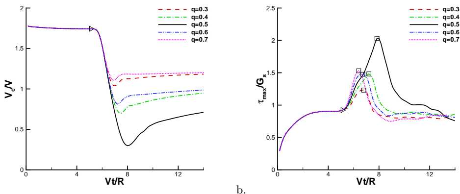
FIGURE 8. Capsule in the branched tube at different branch flow ratios ( a/R = 0.4 , Re = 0.25 , Ca = 0.5 ). Time evolution of (a) the velocity magnitude V_c/V , and of (b) the maximum principal tension. The squares indicate the dimensionless times when \tau_{max} reaches its peak value. The corresponding positions of the capsule centre of mass are shown in Figure 6. The triangle denotes the position where the bifurcation starts to affect the capsule motion.
